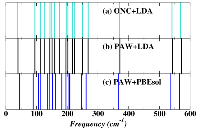
FIG. 4. Frequencies of \mathbf{q} = 0 Raman active modes of \text{Na}_4\text{P}_2\text{S}_6 in the C2/m structure. Comparing results of (a) ONC, (b) PAW, both using LDA, to the results of (c) PAW using PBEsol.
