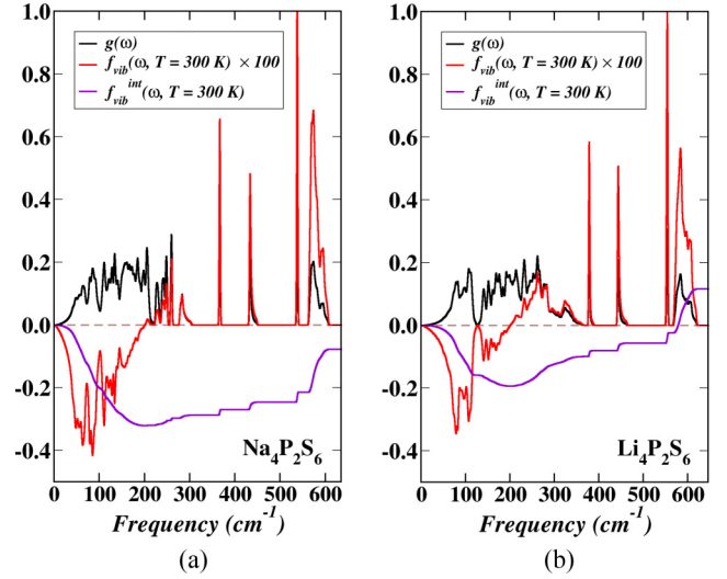
FIG. 8. Details of the vibrational stabilization at T = 300 K for (a) \text{Na}_4\text{P}_2\text{S}_6 , (b) \text{Li}_4\text{P}_2\text{S}_6 in the C2/m structure. In each subplot, the black curve indicates the phonon density of states g(\omega) , the red curve represents the weighted phonon density of states f_{\text{vib}}(\omega, T = 300 \text{ K}) scaled by a factor of 100, and the purple curve gives the integrated weighted phonon density of states factor f_{\text{vib}}^{\text{int}}(\omega, T = 300 \text{ K}) as defined in Eqs. (6), (4), and (5), respectively. In these plots the corresponding vertical scales are in units of states/ \text{cm}^{-1} for g(\omega) , eV/(formula unit)/ \text{cm}^{-1} for f_{\text{vib}} , and eV/(formula unit) for f_{\text{vib}}^{\text{int}} .
