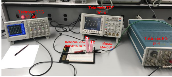
Fig. 6. Measured data acquisition setup with one receiving and one transmitting transducers.
