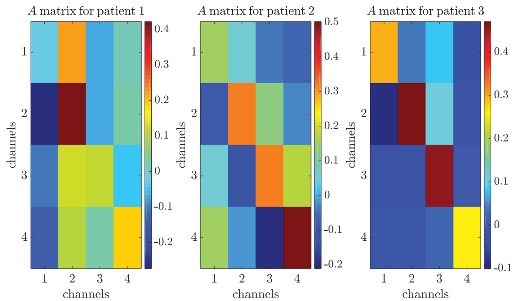
Figure 9. Heatmaps of the A matrix for the three subjects considered in our neuromodulation scheme.
