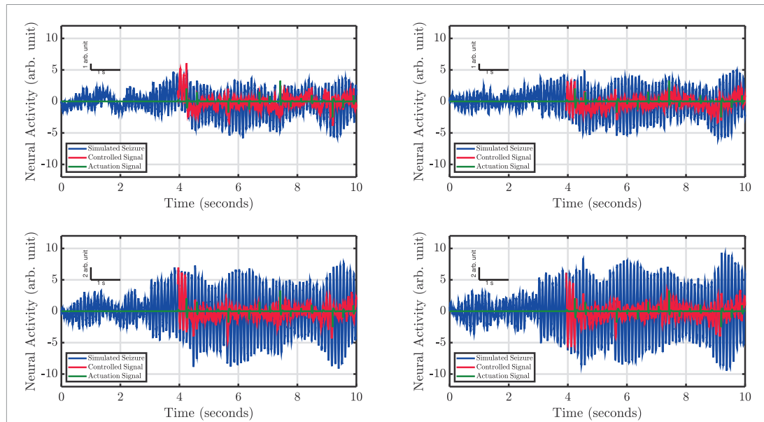
Figure 12. Results of the proposed FOS-MPC closed-loop neurostimulation strategy on iEEG seizure data collected from the second subject with epilepsy during the ictal period. The simulated iEEG signal with the seizure is depicted in blue, the controlled signal is depicted in red, and the stimulation pulses are shown in green.
