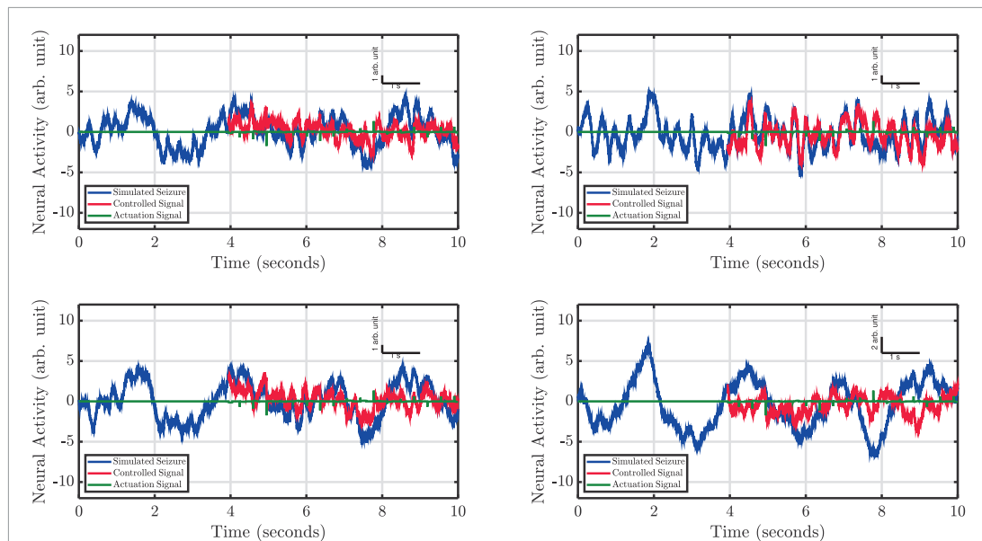
Figure 13. Results of the proposed FOS-MPC closed-loop neurostimulation strategy on iEEG seizure data collected from the third subject with epilepsy during the ictal period. The simulated iEEG signal with the seizure is depicted in blue, the controlled signal is depicted in red, and the stimulation pulses are shown in green.
