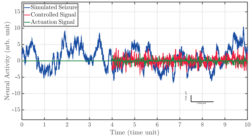
Figure 8. Results of the proposed FOS-MPC closed-loop neurostimulation strategy on an iEEG seizure simulated by the Epileptor model. The simulated iEEG signal with the seizure is depicted in blue, the controlled signal is depicted in red, and the stimulation pulses are shown in green.
