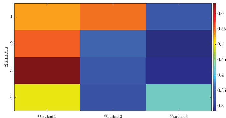
Figure 10. Heatmaps of the fractional-order coefficients \alpha for the three subjects considered in our neuromodulation scheme.
