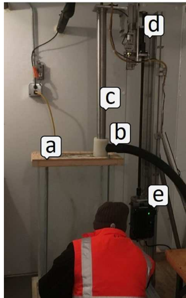
Fig. 7. Cutter test set-up. (a) 0.5 \text{ m} \times 0.25 \text{ m} \times 1 \text{ m} ice block. (b) Vacuum chip removal hose. (c) RAM-2 Motor section. (d) Ball screw linear drive. (e) Drive motor with a controller.
