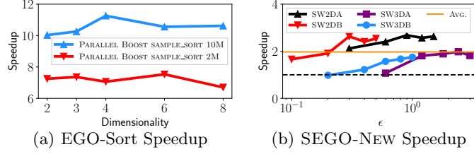
Fig. 5. (a) Speedup to EGO-Sort our synthetic datasets using SAMPLE_SORT from the Boost library over QSORT from the C standard library. S = 0\text{--}9.39\text{K} and S = 0\text{--}1.99\text{K} on the 2M and 10M points datasets, respectively. (b) Speedup of SEGO-NEW over SUPER-EGO on the SW -real-world datasets.
