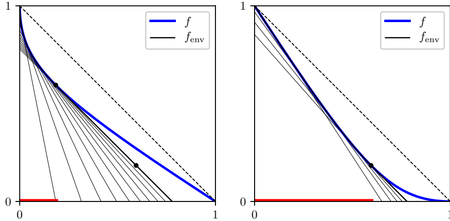
Figure 14: Symm explained. Left panel: \bar{x} \leq f(\bar{x}) . Right panel: \bar{x} > f(\bar{x}) .
