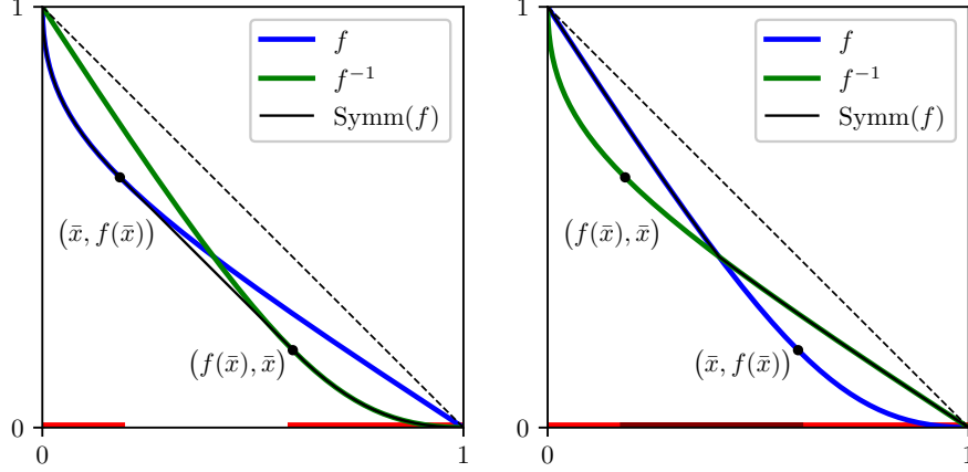
Figure 13: Action of Symm. Left panel: \bar{x} \leq f(\bar{x}) . Right panel: \bar{x} > f(\bar{x}) . For both panels the effective parts (red bars on x -axes) are [0, \bar{x}] of f and [f(\bar{x}), 1] of f^{-1} . No overlap in the left panel since \bar{x} < f(\bar{x}) , so interpolate with straight line; overlap in the right panel so the max is taken.
