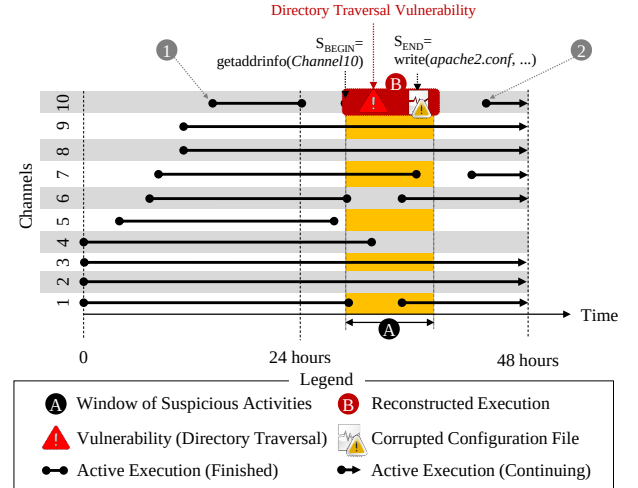
Fig. 14. Reconstructed partial execution of HexChat.
