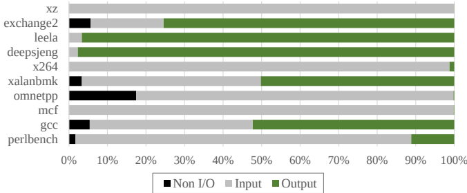
Fig. 12. SPEC CPU2017 Space Overhead Breakdown.
