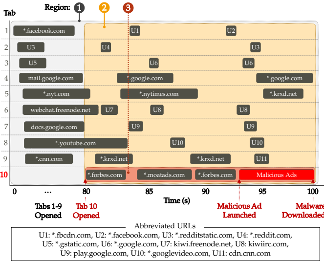
Fig. 1. Timeline of an execution of 10 browser tabs. The x-axis represents the time for the execution (in seconds) and the y-axis represents 10 different browser tabs. The abbreviated URLs (i.e., U1~U11) are shown in the bottom.
