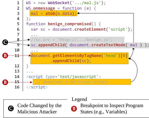
Fig. 13. Investigating a Fileless Attack via JavaScript.
