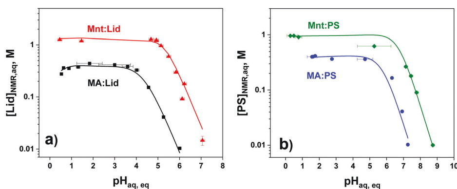
Fig. 4 pH-Dependent aqueous phase solubility of the hydrogen bond acceptor for (a) lidocaine- and (b) Proton Sponge®-based mixtures into hydrochloric acid. The subscript NMR indicates the total measured concentration (protonated and neutral combined). Lines are fit according to eqn (16).
