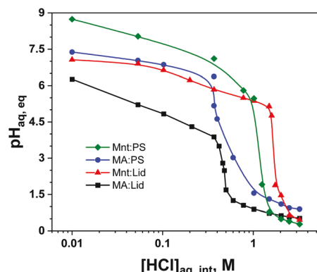
Fig. 3 Equilibrium pH of the aqueous phase after thorough mixing with each organic binary mixture as a function of initial HCl concentration in the aqueous phase. Uncertainties are smaller than the symbols. Lines are drawn to guide the eye.
