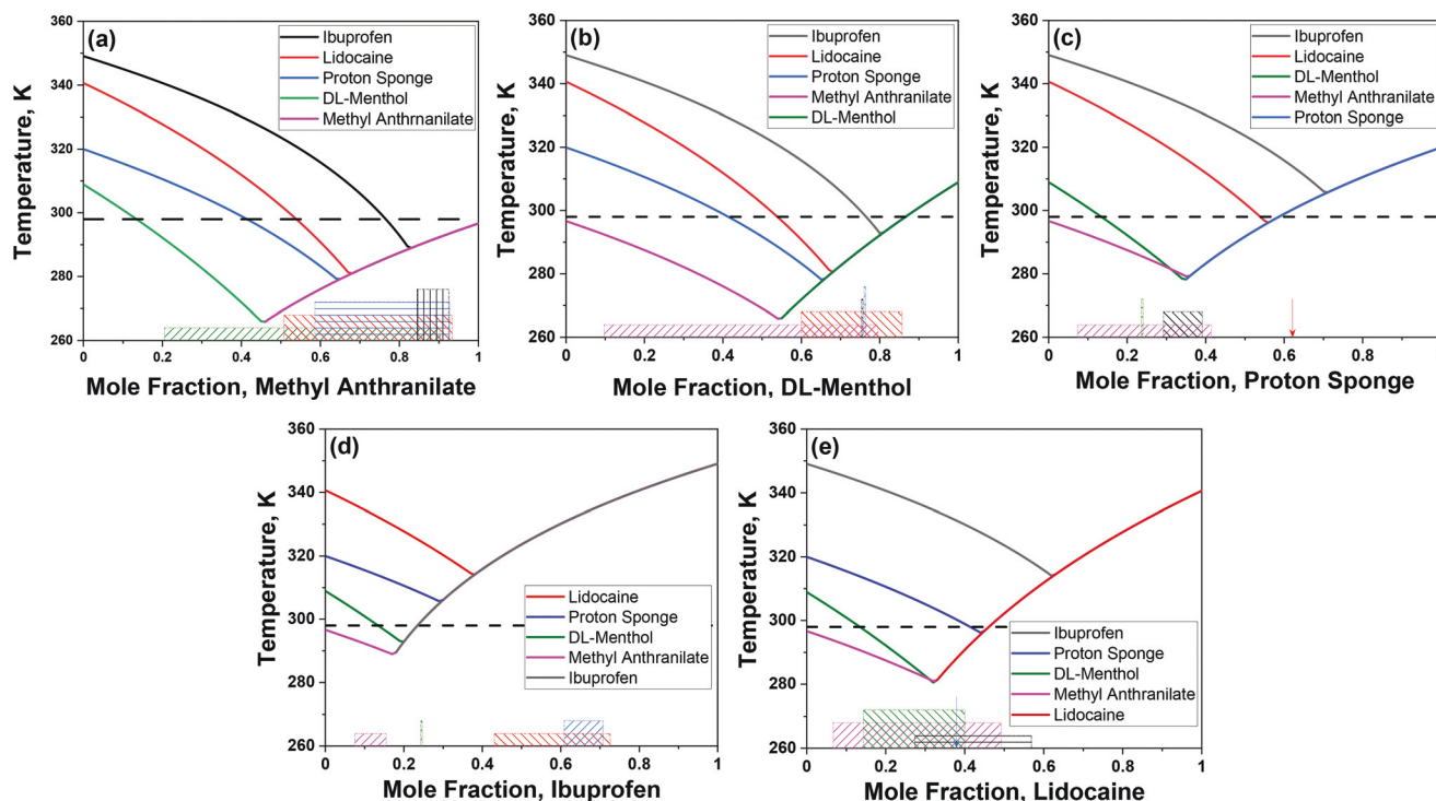
Fig. 1 Predicted ideal solubility curves for (a) methyl anthranilate, (b) DL-menthol, (c) Proton Sponge®, (d) ibuprofen, and (e) lidocaine based solvents using eqn (4). The dashed line indicates room temperature (298 K). The rectangular represents a region of experimentally found liquid at room temperature homogeneous binary mixture. The arrow shows one solid at room temperature Lid : PS eutectic.
