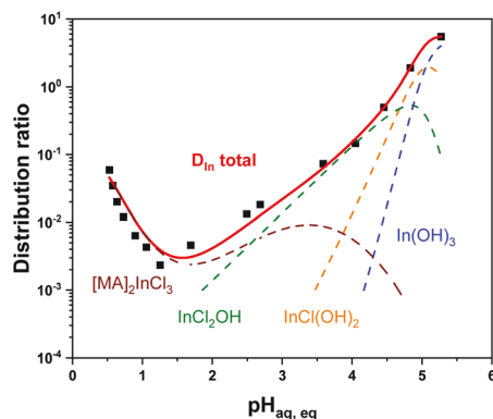
Fig. 7 Extraction of indium from HCl into MA : Lid (wet) as a function of equilibrium aqueous pH. The lines are fit according to eqn (28), with the solid line showing the complete fit and the dashed lines indicating the contribution of each individual species, calculated by setting all other extraction constants to zero. Uncertainties are smaller than the symbol size.
