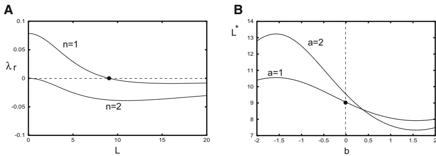
Fig. 2 Numerically determined solutions to the eigenvalue problem (13) for \Delta(u) = a(\sin(b) - \sin(u+b)) . a Real part of the eigenvalue as L varies for \lambda_m \approx n . Solid dot shows the value of L at which the \lambda_r changes sign. b The critical value L^* at which \lambda_r = 0 when n = 1 as b varies for a = 1, 2 . Solid dot corresponds to the dot in panel A
