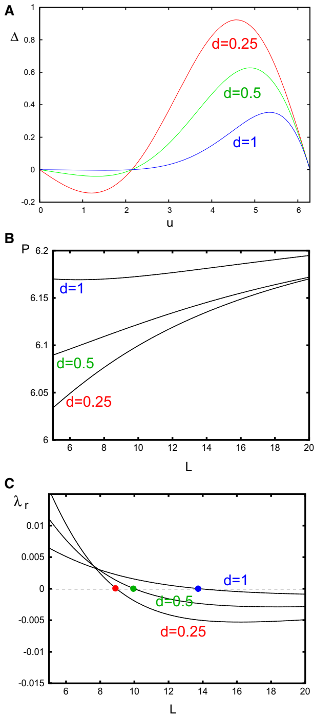
Fig. 3 Dispersion relation (period, P ) and stability of waves as the ring length, L , varies for approximations (14) of the PRC for a mitral cell. a PRC with a = 1 , b = 0.5 and d = 0.25, 0.5, 1.0 . b Dispersion relation corresponding to the PRCs in A. c Stability of waves (dots indicate the critical ring length where stability is lost)
