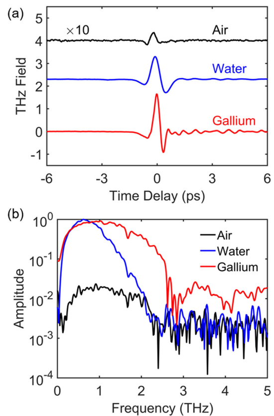
FIG. 2. Comparison of THz waves generated from air and a 210 \mu m diameter lines of water and gallium with a single-color excitation scheme. (a) Comparison of THz field strengths in air plasma, water, and liquid gallium. The THz signal from single color air plasma is enlarged by 10 times. (b) Corresponding comparison in the frequency domain.
