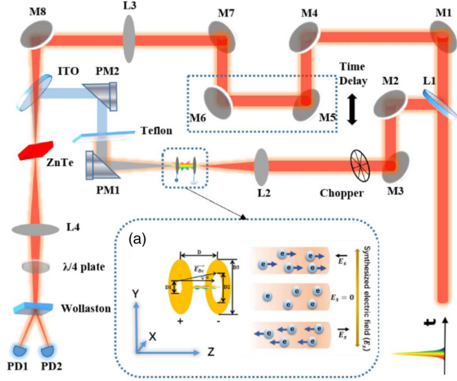
FIG. 3. Schematic diagram of the experimental setup showing the generation and detection of THz radiation. The orientation of the EO crystal and optical detection polarization are chosen to measure the appropriate THz field polarization. Inset (a) shows the construction of two circular copper electrodes and the direction of electron movement in the laser plasma under the synthesized electric field.
