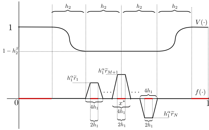
FIG. 2. The black solid line on the top represents the variance function V(\cdot) in the alternative \tilde{H}_1 , and the black solid line on the bottom represents the mean function f(\cdot) . The thick red segments mark the support of X under both H_0 and \tilde{H}_1 . Here, h_1 \asymp n^{-\frac{2\beta}{4\alpha\beta+\beta+2\alpha}} , h_2 \asymp n^{-\frac{4\alpha}{4\alpha\beta+\beta+2\alpha}} , and are chosen such that both M := h_2/(4h_1) - 1/2 and N := 2M + 1 are positive integers. \{\tilde{r}_i\}_{i=1}^N are N i.i.d. standard normal variables.
