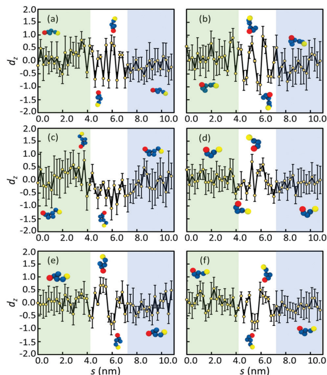
Fig. 6 Orientational analysis of carbapenems along the translocation coordinate in OccD3. The variation in d_z for (a) biapenem, (b) doripenem, (c) ertapenem, (d) imipenem, (e) meropenem, and (f) panipenem as a function of s . The mean d_z values are denoted by the yellow dots, and the standard deviations are shown by the black bars. The s coordinate is subdivided into outer membrane region (white), constriction region (green), and periplasmic region (blue).
