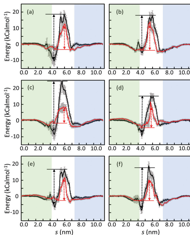
Fig. 5 The PMF profiles of carbapenems through OccD3 and OccD3m. The comparison of (a) biapenem, (b) doripenem, (c) ertapenem, (d) imipenem, (e) meropenem, and (f) panipenem translocation through OccD3 (black line) and OccD3m (red line). The error bars calculated using the bootstrap analysis are marked in gray. The barrier heights (dashed lines) are marked in each panel. The translocation coordinate ( s ) is subdivided into outer membrane region (green), constriction zone (white) and periplasmic region (blue).
