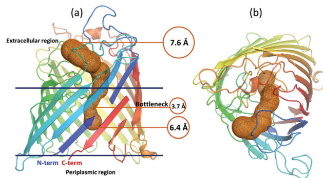
Fig. 1 Molecular structure of OccD3 porin. The (a) side-view and (b) top-view of OccD3 in cartoon representation (colored blue to red from N-term to C-term) along with the porin channel (in orange surface representation). The diameter of the channel is marked in circles. The two horizontal lines show the membrane embedded region of the porin.
