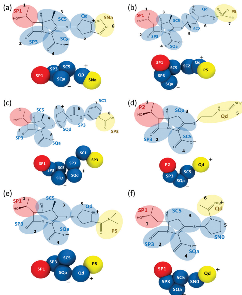
Fig. 4 Atomistic to CG mapping for (a) biapenem, (b) doripenem, (c) ertapenem, (d) imipenem, (e) meropenem, and (f) panipenem showing the MARTINI bead type assignments along with positive and negative charges. The red bead, which is part of the \beta -lactam ring, denotes the head and the yellow bead, the farthest bead from the \beta -lactam ring, denotes the tail.
