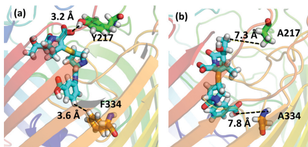
Fig. 8 Comparison of reserve-mapped atomistic structure and orientation of ertapenem in the bottleneck region, s = 5.8 nm of (a) OccD3 and (b) OccD3m channel. The contacts the molecules make with the pore-lining residues in their highest energy conformation. The porin is shown in ribbon representation (blue to red from N-term to C-term) and ertapenem is shown as sticks (C cyan; O red; H white; S gold; and N blue). The pore-lining residues are shown in stick representation Y217 and A217 (C green), and F334 and A334 (C orange); the other atoms have same color scheme as in ertapenem.
