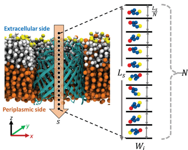
Fig. 3 The CLASP simulation setup. The membrane embedded porin channel oriented parallel to the z -axis is divided into N equidistant umbrella sampling windows. The probe molecule is inserted into each W_i window.
