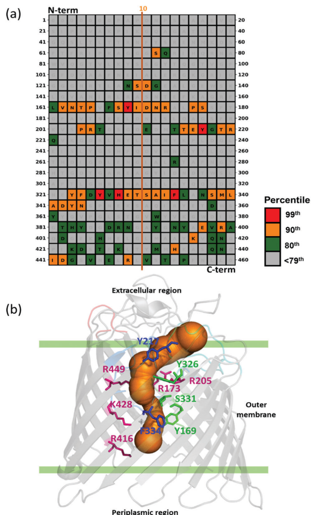
Fig. 7 Interaction of meropenem with OccD3 porin channel. (a) Meropenem-OccD3 contact map, and (b) structure of the OccD3 (cartoon representation, gray) along with key pore-lining residues (stick model) that line the channel (orange, surface representation).
