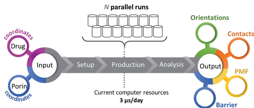
Fig. 2 The CLASP workflow. The systematic representation of CLASP inputs and outputs. The porin and solute coordinates are the required inputs, which then are processed by the C_setup.py python script to generate N parallel umbrella sampling runs. The post simulation analysis scripts combine the N trajectories to generate the free energy profile, solute-protein residue contact map, and solute orientational analysis.
