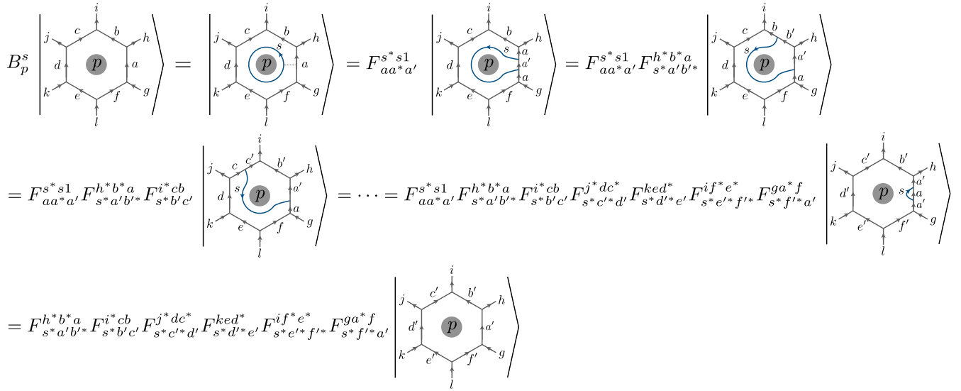
FIG. 11. Definition of the B_p^s term in the Levin-Wen model where we use the Einstein summation convention, i.e., summation is assumed for repeated indices. B_p^s inserts an anyonic flux s around the plaquette p ; we use a series of F -matrices to compute the matrix element of B_p^s . B_p^s is a 12-spin interaction for a hexagonal plaquette p , and it acts diagonally on states on external legs denoted as states i, j, \dots, h .
