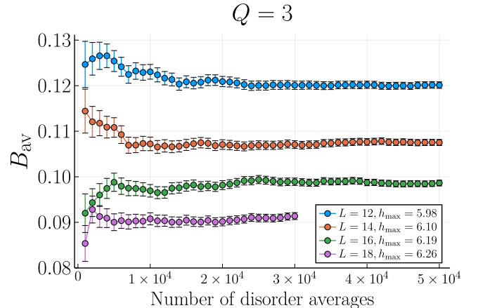
FIG. 35. Convergence of the disorder-averaged binder ratio B_{\text{av}} as a function of the number of disorder averages for Q = 3 for various system sizes L and the field strength h_{\max} .
