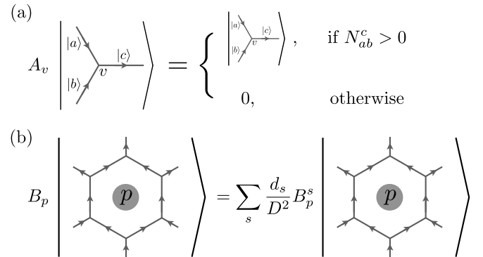
FIG. 32. (a) Definition of the vertex term A_v in the Levin-Wen model. A_v projects onto the configuration where three anyons on the adjacent links are compatible with the fusion rule. (b) Definition of the plaquette term B_p in the Levin-Wen model. B_p is given by the summation of \frac{d_s}{D^2} B_p^s , where B_p^s operator is defined in Fig. 11.
