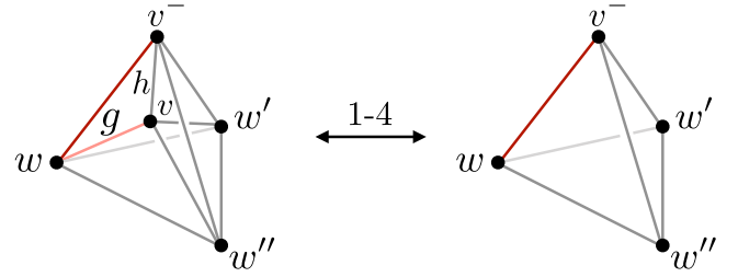
FIG. 24. Graphical proof of Eq. (B3). The 3-manifold on the left is obtained by gluing the tetrahedron associated with the U(1) phase factors appearing in the amplitude of |g; g_1, g_2\rangle in Eq. (B2) and the 3-manifold from the tent construction of A_v^{h,w} . The 3-manifold on the right is associated with the phase factor of the amplitude of |h \cdot g; g_1, g_2\rangle in Eq. (B2). The U(1) phase factors associated with the above two 3-manifolds are identified by a 1-4 Pachner move.
