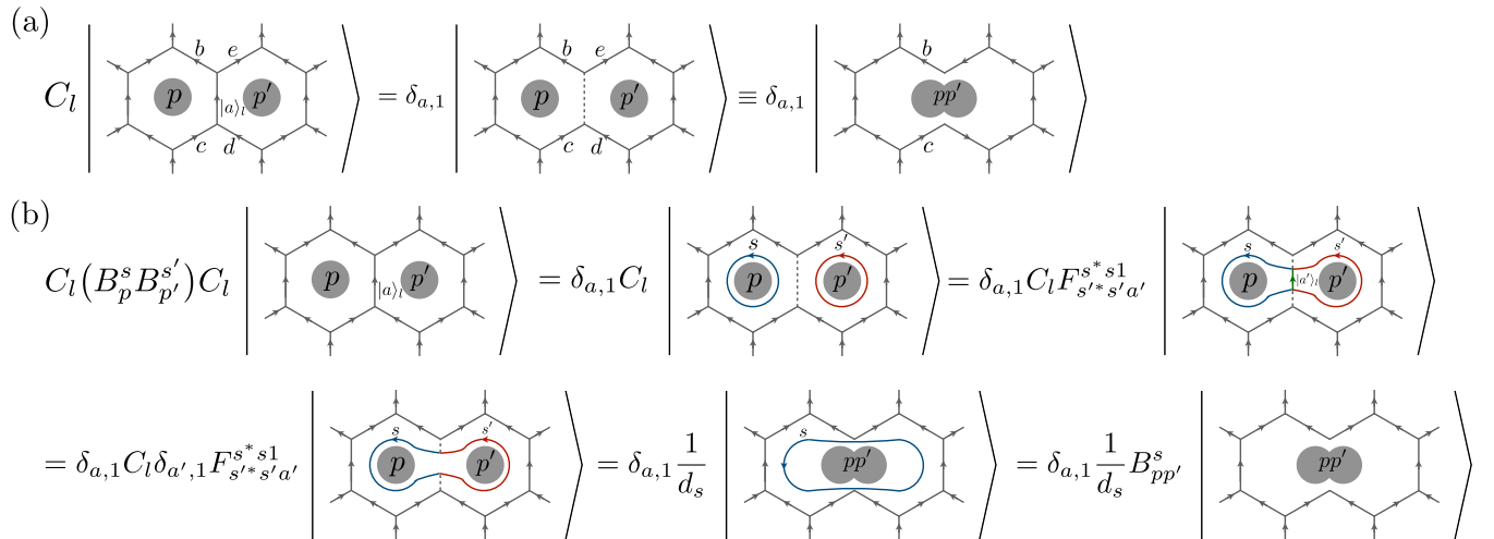
FIG. 12. (a) For a link decimation C_l = 1 , we polarize the spin state at l to the trivial state |1\rangle and remove link l from the lattice. Such link decimation naturally identifies the states b = e^* and c = d^* , where * appears due to the direction of links. Accordingly, four adjacent links to l become two links after the identifications as described in the RHS. (b) Computation of C_l(B_p^s B_{p'}^{s'})C_l on the C_l(|a\rangle_l \langle a|_l) = 1 subspace. The summation over a' is implicit in the RHS of the second equality. As a result of computation, we get the plaquette term B_{pp'}^s associated with the larger plaquette pp' .
