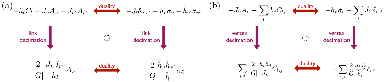
FIG. 4. The RSRG of the Q -state Potts model and the G -gauge theory and the duality mappings (where Q = |G| ). Here we denote the Ising-type interaction and the transverse field term in the Potts model as \hat{\delta}_{v,v'} and \hat{\sigma}_v . (a) Link decimation and (b) vertex decimation both commute with the duality mapping where the corresponding changes in the graph \mathcal{G} \mapsto \mathcal{G}' can be found in Fig. 2. A long-link term C_l such as C_{l_{34}} in Fig 2 (b) corresponds to a dual higher-neighbor ferromagnetic interaction term between spin states at vertex 3 and 4 with respect to a planar graph \mathcal{G}' .
