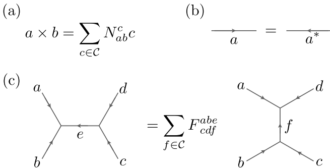
FIG. 31. Input data for the Levin-Wen model. (a) The fusion rule among anyons in \mathcal{C} . (b) If we invert the direction of a link, we take antiparticle of the corresponding anyon label. (c) F -matrix associated with the change in the fusion basis.
