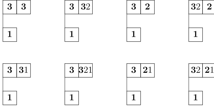
FIGURE 5. The eight elements of \overline{\mathfrak{A}}\mathfrak{SSF}(102) . The set \overline{\mathfrak{A}}\mathfrak{2}\overline{\mathfrak{P}}(102) consists of two fillings, specifically the leftmost filling in each of the two rows. Each of the eight illustrated fillings destandardizes to the leftmost filling in its row.
