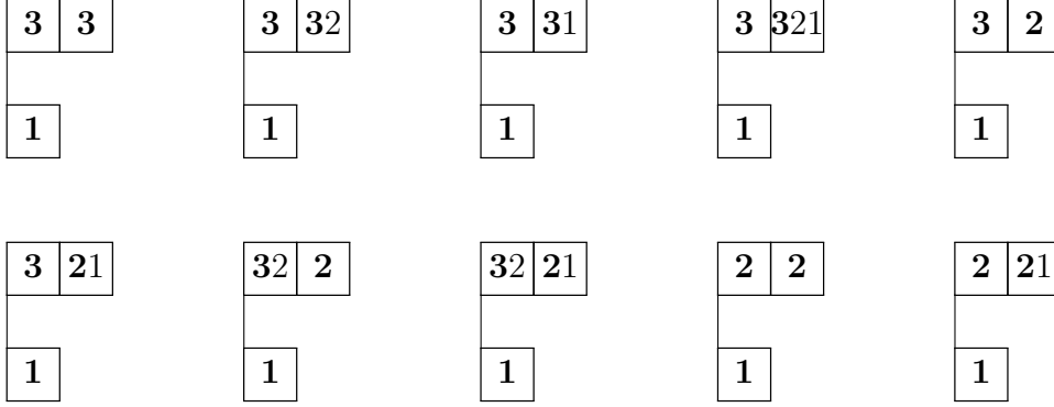
FIGURE 6. The ten elements of \overline{\mathcal{Q}}\text{SSF}(102) .
