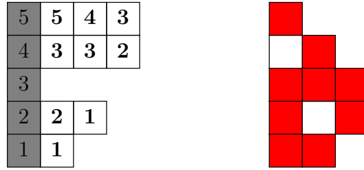
FIGURE 8. The semistandard key tableau equivalent to the filling T \in \mathfrak{DSSF}(a) of Example 4.29, together with its corresponding Kohnert diagram.
