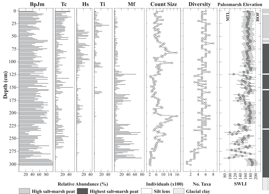
FIGURE 3. Foraminifera enumerated from 1-cm thick samples of sediment in core F25 from Big River, Newfoundland. Taxon abundance (cumulatively these taxa comprise 99% of counted individuals in the core) are shown as percentages for ease of comparison among samples, but count size is presented. BpJm = Balticammina pseudomacrescens/Jadammina macrescens ; Tc = Tiphotrecha comprimata ; Hs = Haplophragmoides spp.; Ti = Trochammina inflata ; Mf = Miliammina fusca . Paleo-marsh elevation was reconstructed using a weighted averaging (WA) transfer function applied to full counts, where the relationship between foraminifera and tidal elevation was empirically determined from a regional-scale modern training set of 134 samples from Big River, Hynes Brook, and Placentia. SWLI = standardized water level index where a value of 100 corresponds to local mean tide level (MTL) and 200 is the highest occurrence of foraminifera (200). Modified from Kemp et al. (2018b).
