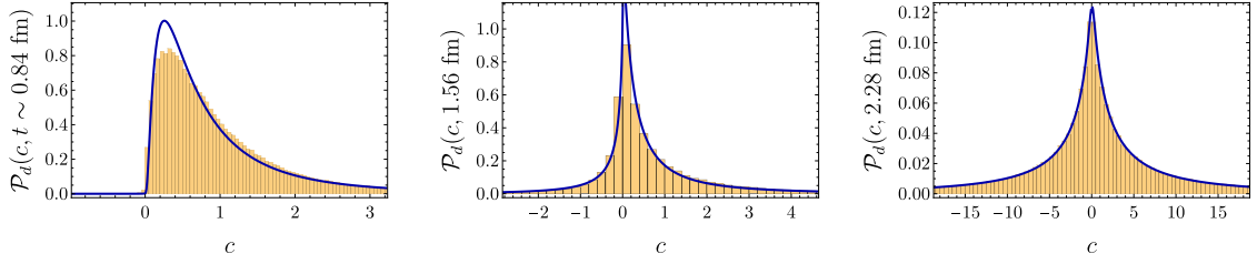
Fig. 6. Histograms of the real parts of deuteron correlation functions with m_\pi = 450 MeV from Ref. [304], at three values of t normalized independently by multiplying by 1/(\text{Re } C_d(t)) . The blue curves show fits to complex log-normal distributions obtained as in Refs. [379,380] from a product of a log-normal distribution with mean \mu_R = \langle r_d \rangle and variance \sigma_R^2 = \langle r_d^2 \rangle - \mu_R^2 times a wrapped-normal distribution with zero mean and variance \sigma_\theta^2 = -\ln((\cos \theta_d)^2 + (\sin \theta_d)^2) obtained using sample mean estimators for \mu_R , \sigma_R^2 , and \sigma_\theta^2 from LQCD results for C_d = e^{r_d + i\theta_d} . The distribution of the real part shown is obtained by marginalizing over the imaginary part of the resulting distribution for the complex variable C_d .
