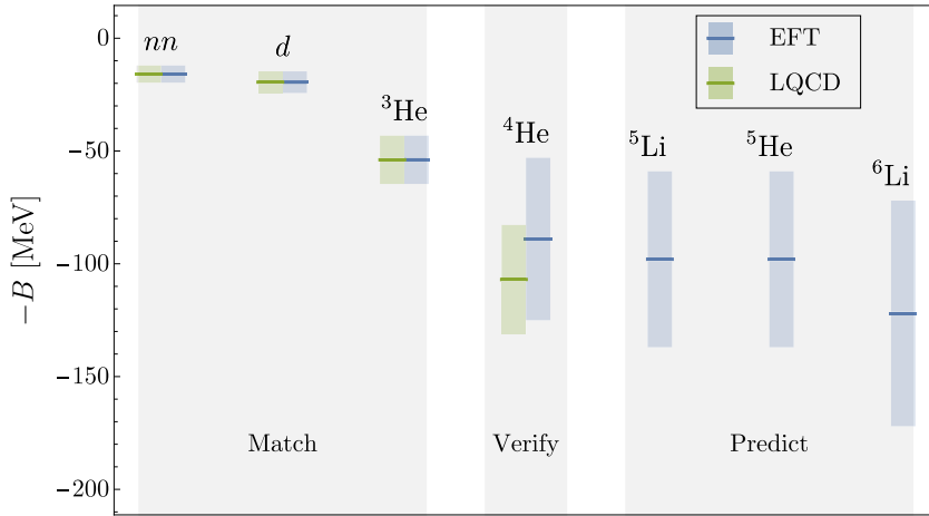
Fig. 5. Binding energies of the deuteron, dineutron, ^3\text{He} , and ^4\text{He} at an \text{SU}(3) flavor-symmetric point obtained with LQCD at quark masses corresponding to a pion mass of 806 MeV [108] are used to obtain the binding energy of light nuclei up to A = 6 using an AFDMC computation with the pionless EFT [127]. The two- and three-nucleon LECs were constrained by the LQCD calculation of the A \in \{2, 3\} binding energies. Source: Data from Refs. [108,127].
