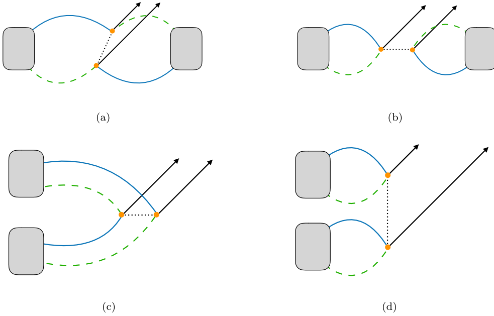
Fig. 17. Contractions for the \pi^- \rightarrow \pi^+ e^- e^- transition, (a) and (b), and for the \pi^- \pi^- \rightarrow e^- e^- transition, (c) and (d). The solid blue and dashed green lines represent down and up quark propagators respectively, and the circles correspond to the \Delta I = 1 weak vertices. The dotted and solid black lines represent the Majorana neutrino propagator and electron final states respectively. Source: Figure modified from Ref. [628].
