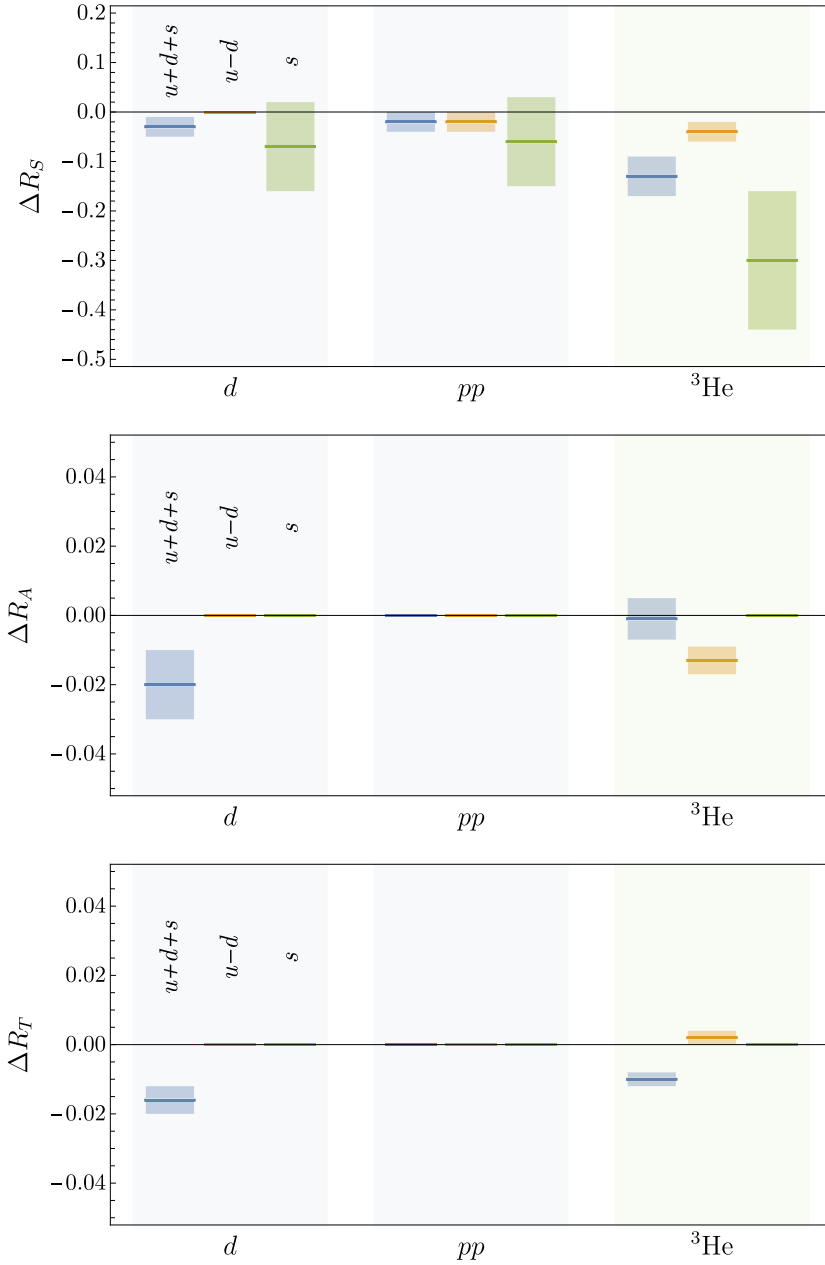
Fig. 21. Differences \Delta R_X between LQCD calculations of the ratios R_X^{(f)}(A) = g_X^{(f)}(A)/g_X^{(f)}(p) for nuclear matrix elements g_X^{(f)}(A) of nuclei A with Dirac structure X = \{S, A, T\} and flavor combination f , from their values calculated using nuclear ground states with non-interacting nucleons occupying only the lowest shell-model states. The strange-quark matrix elements are small and indistinguishable from zero for the axial and tensor matrix elements. Quantities that are identically zero are shown by lines at zero, and there is no associated uncertainty band. Source: Data from Ref. [41].
