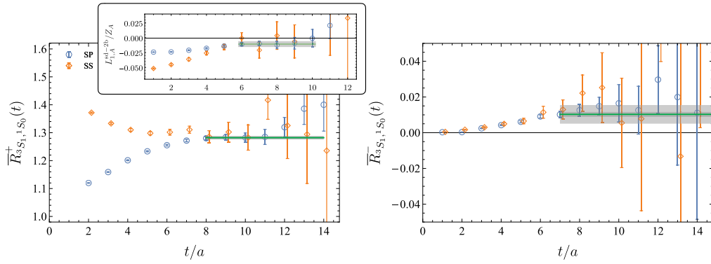
Fig. 12. The quantities \bar{R}_{3, S_1, S_0}^+(t) (left) and \bar{R}_{3, S_1, S_0}^-(t) (right). The former asymptotes to the pp \rightarrow d bare matrix element at large times, while the latter gives an estimate of dominant excited-state contaminations to the desired matrix element. Shown in the inset in the left is the (unnormalized) difference between the full matrix element and the single-nucleon contribution, giving rise to quantity L_{1,A}^{sd-2b}/Z_A at large times. Different colors (blue and orange) represent two different choices for the sink interpolating operators. For further detail, see Refs. [38,39]. Source: Figure modified from Ref. [38].
