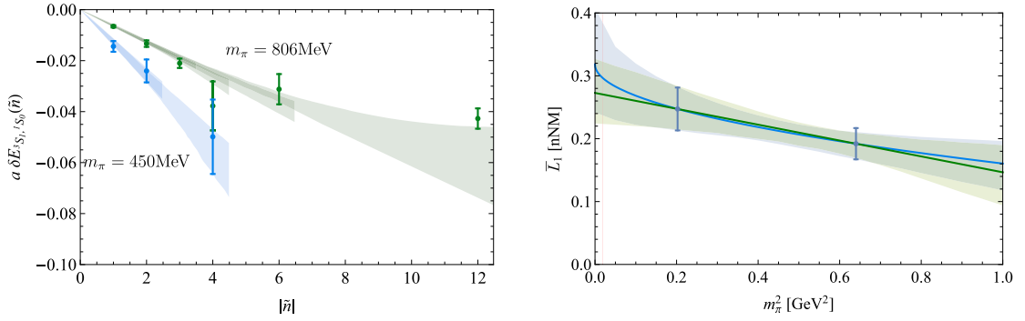
Fig. 11. LQCD results for the energy splittings between the two lowest-lying eigenstates of the \mathfrak{S}_1 – \mathfrak{S}_0 system (left), with the single-nucleon contributions removed as a function of the magnetic field strength quantum \tilde{n} , along with the associated fits to extract the linear response. Also shown are the results of LQCD calculations of \bar{L}_1 (blue points) (right). The blue (green) shaded regions show extrapolations of \bar{L}_1 to the physical pion mass (red vertical line) in natural nuclear magnetons (nNM) which are linear (quadratic) in m_\pi . Source: Figure modified from Ref. [37].
