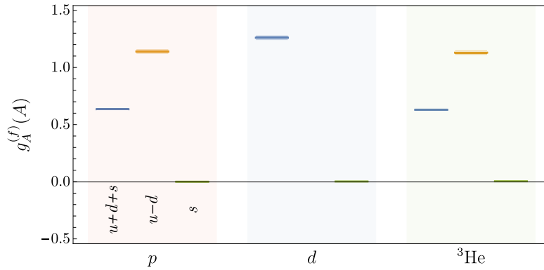
Fig. 14. Flavor separation of the axial-current matrix elements in the proton, deuteron, and ^3\text{He} , determined in Ref. [41] using calculations with m_\pi = 806 MeV. Since the deuteron is isoscalar, it has no isovector charge. The strange quark charges are very small and consistent with zero in each case.
