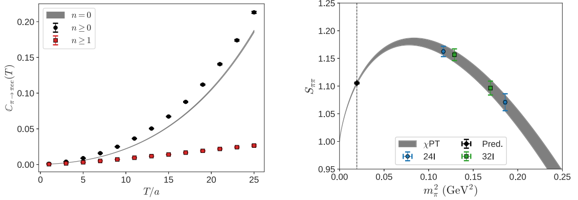
Fig. 18. The integrated transition amplitude from Ref. [149] for an example ensemble before and after subtracting the vacuum state contribution in Eq. (96) for fixed t (left). Also shown is the pion mass dependence of the matrix element normalized by the matrix element in the chiral limit, S_{\pi\pi} , as constrained by the chiral/continuum/finite volume extrapolation [149] (right). The dotted vertical line in the right panel indicates the physical pion mass.
