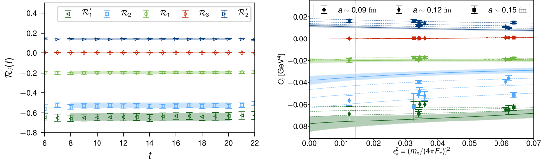
Fig. 20. An example of the ratio of correlation functions, \mathcal{R}_i \equiv \mathcal{R}_{3/2, \mathcal{O}_i^{++}}^{(\pi)} for the five relevant 0\nu\beta\beta operators on a near-physical pion-mass ensemble with a \approx 0.12 fm (left). The horizontal bands are the ground-state contributions to R_i extracted from single-state fits. Interpolations/extrapolations of the pion matrix elements (right). The bands represent the 68% confidence interval of the continuum, infinite-volume extrapolated values of the matrix elements. The vertical gray band indicates the physical pion mass. Source: Figures from Ref. [145].
