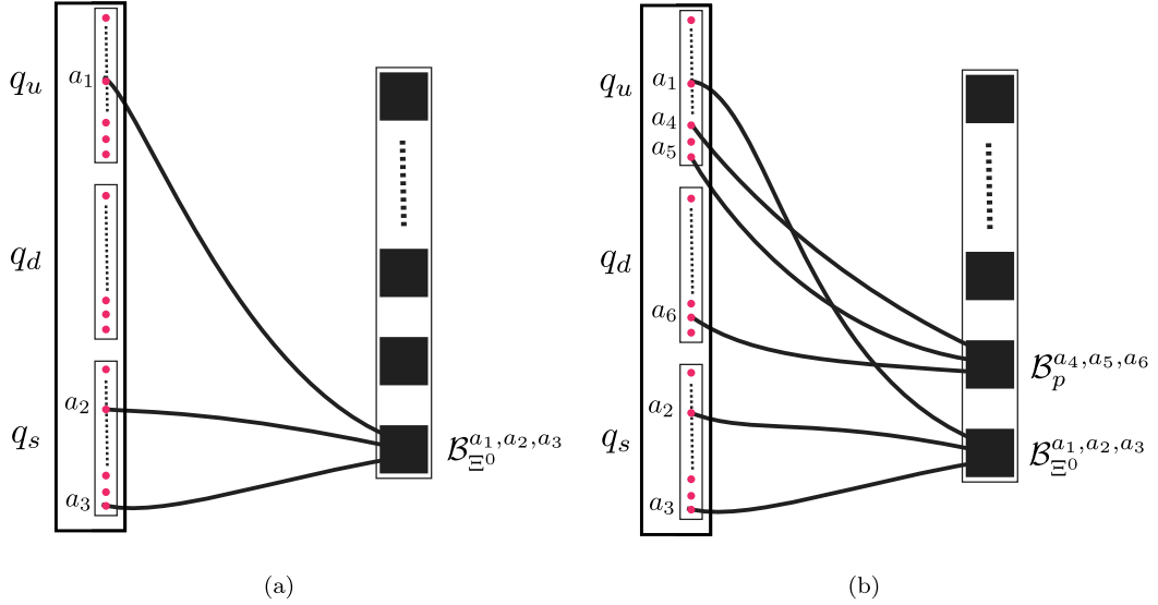
Fig. 2. Illustration of the first two steps of the quark-hadron contraction method. The small circles in the left-hand section of each figure correspond to the quarks in the source interpolating operator, while the large squares in the right-hand sections, and lines extending from them, correspond to the hadronic blocks. In the first step (a), the indices of the first baryon block are contracted with the quark fields. In the second (b) and subsequent steps, additional baryon blocks are included and contracted with the remaining quark indices in the source wavefunction.
