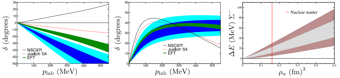
Fig. 4. The 3S_1 (left panel) and 1S_0 (center panel) n\Sigma^- phase shifts versus laboratory momentum computed with LQCD and extrapolated to the physical pion mass using EFT (blue bands), along with other determinations (green bands are EFT fits to data, while the black and red curves are predictions from phenomenological models). The right panel shows the energy shift versus neutron density of a \Sigma^- in a non-interacting Fermi gas of neutrons as determined from Fumi's theorem. The inner (outer) band encompasses statistical (systematic) uncertainties. Source: Figure from Ref. [129].
