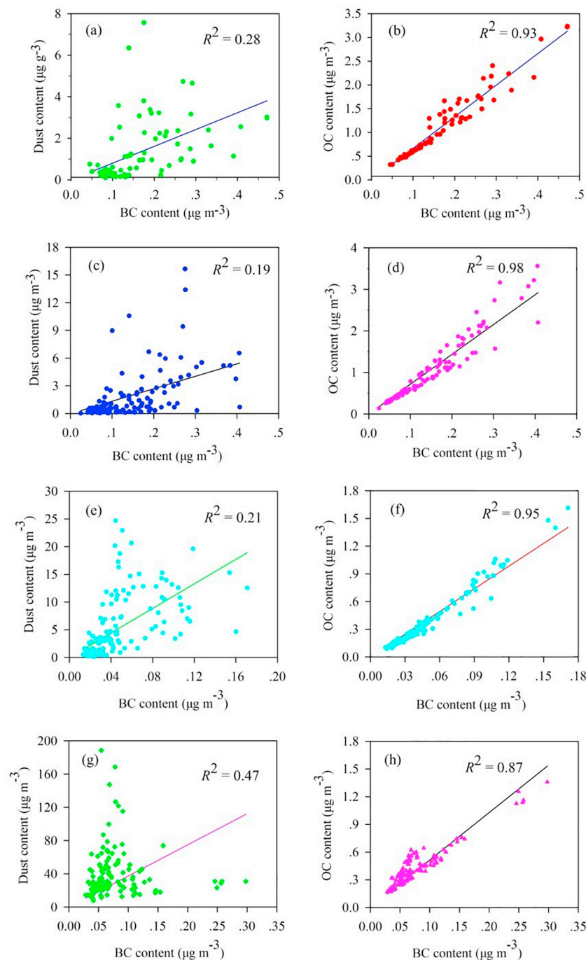
Fig. 11. Correlations between simulated near-surface atmospheric BC and dust, BC and OC concentrations at Mt. Yulong glacier (a), (b); Zhadang glacier (c), (d); DKMD glacier (e), (f); LHG glacier (g), (h).
