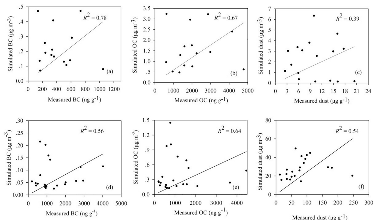
Fig. 10. Regression analysis of measured and simulated BC, OC, dust concentrations in the surface layer of snowpack and in the aerosol at surface over the Mt. Yulong (upper panel) and Laohugou glacier (Lower panel).
