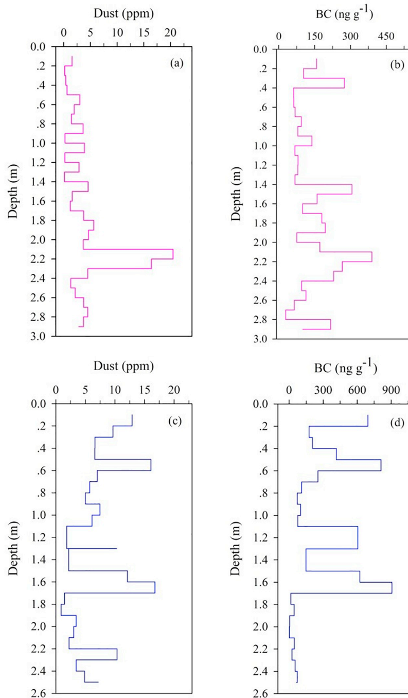
Fig. 4. Vertical distribution of BC and dust in snowpits collected on 14 June 2017 (a, b) and 22 June 2017 (c, d).
