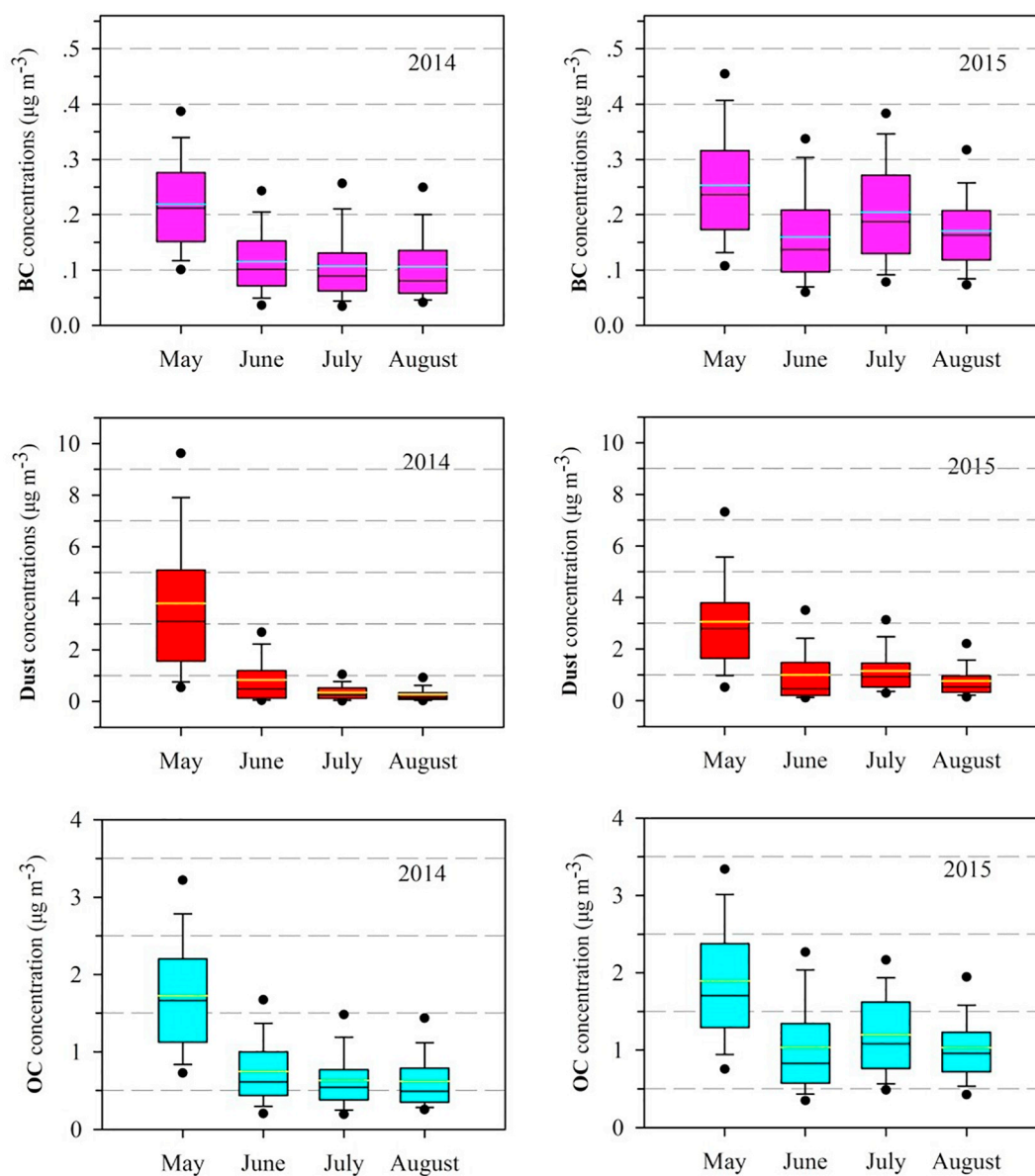
Fig. 9. Monthly and annual differences of the modeled BC, dust, and OC concentrations in aerosol at surface over Mt. Yulong in May–August in 2014 and 2015.
