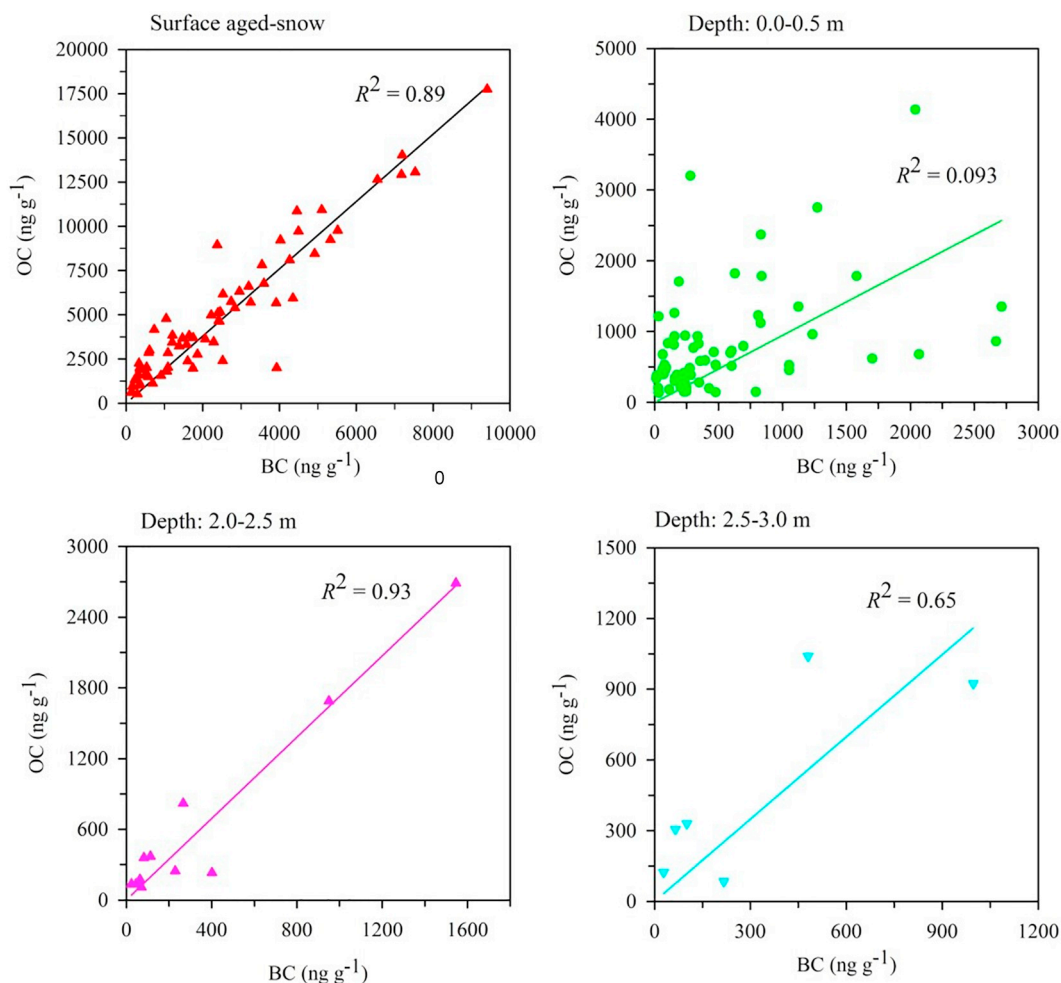
Fig. 3. Regression analyses between measured BC, OC concentrations in surface aged-snow and three depth bins of snowpit from Mt. Yulong.
