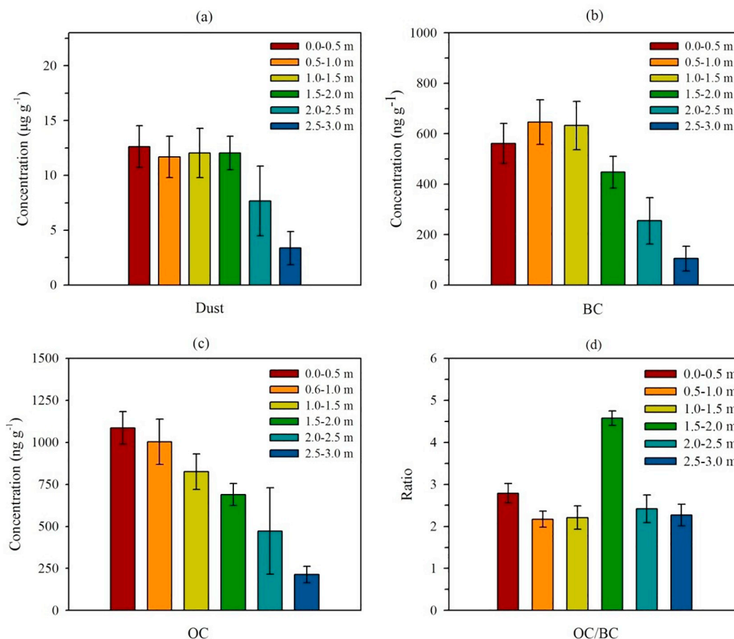
Fig. 6. The average BC, OC, dust concentrations and OC/BC ratio in different depth-intervals of snowpit from Mt. Yulong.
