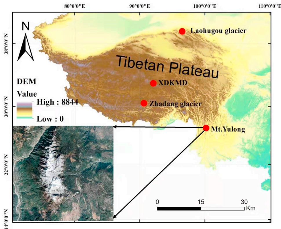
Fig. 1. The location of Mt. Yulong, Laohugou (LHG), Xiaodongkemadi (XDKMD), and Zhadang (ZD) glaciers on the Tibetan Plateau.
