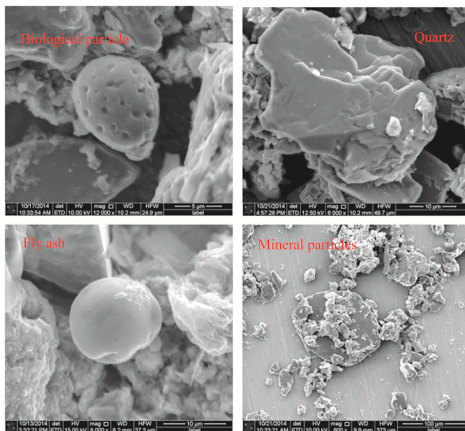
Fig. 13. Typical morphology of individual particles in the glacier cryoconite from Mt. Yulong detected using scanning electron microscopy, coupled with energy dispersive X-ray spectrometer (SEM-EDX) method.
