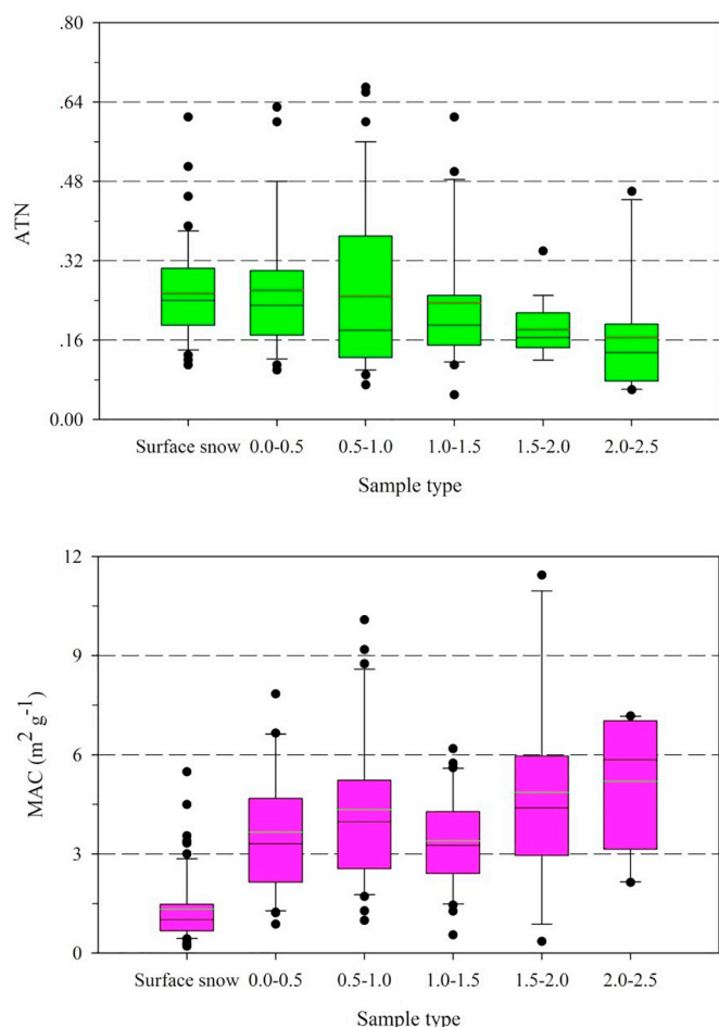
Fig. 7. Variation of light absorbing characteristics of BC in the surface aged-snow and five depth intervals of snowpit. ATN denotes optical attenuation of BC, MAC denotes mass absorption cross-section of BC (unit: \text{m}^2 \text{g}^{-1} ).
