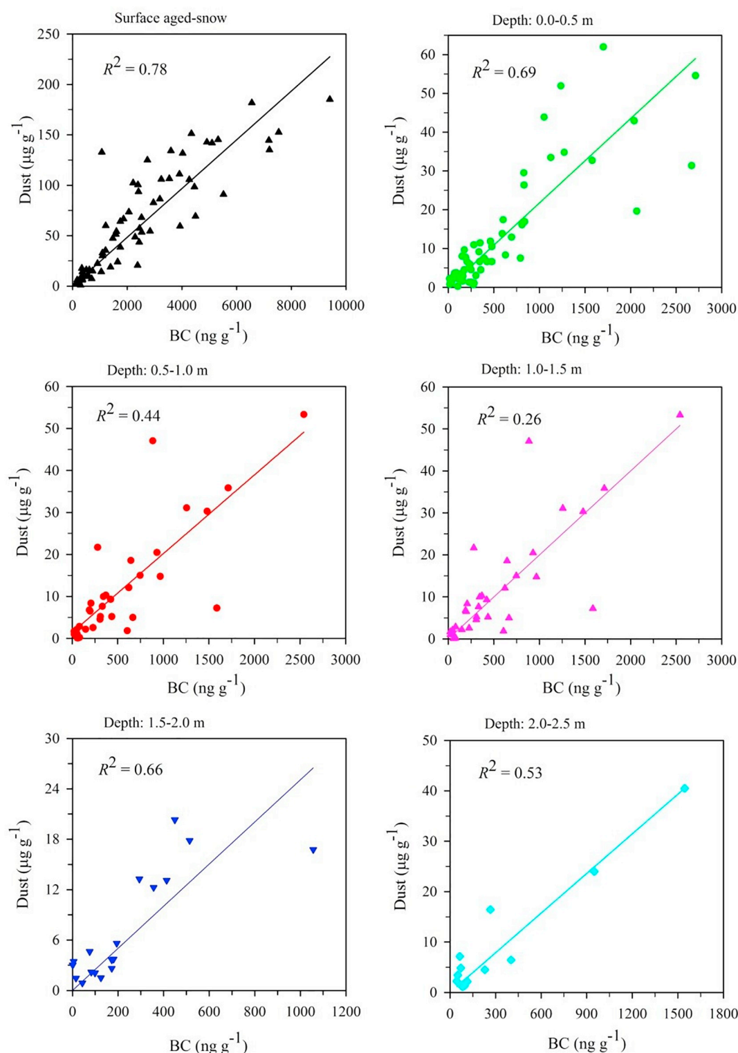
Fig. 2. Correlations between measured BC, dust concentrations in surface aged-snow and five depth bins of snowpit from Mt. Yulong.
