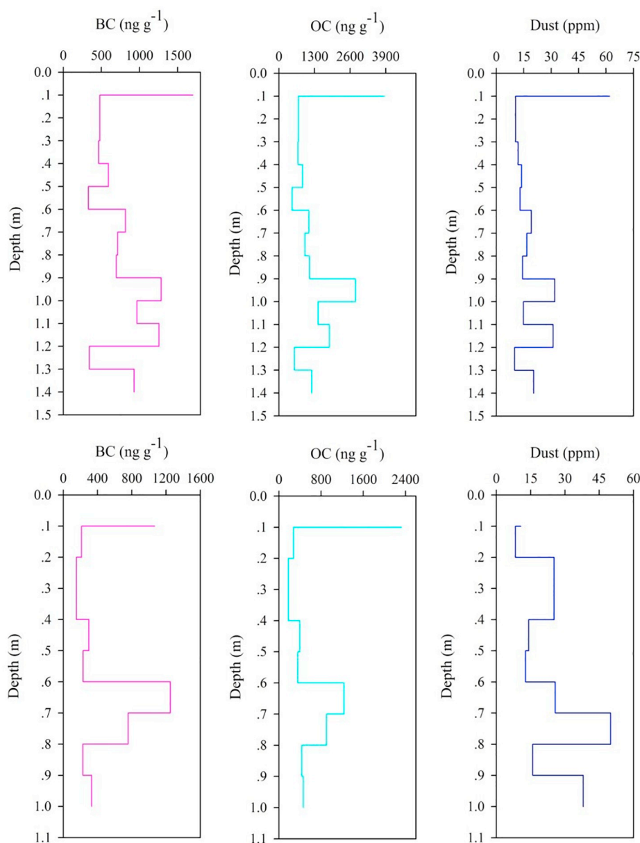
Fig. 5. Vertical distribution of BC, dust, and OC concentrations in snowpits collected on 3 June 2016 (upper panel) and 17 April 2018 (lower panel) from Mt. Yulong.
