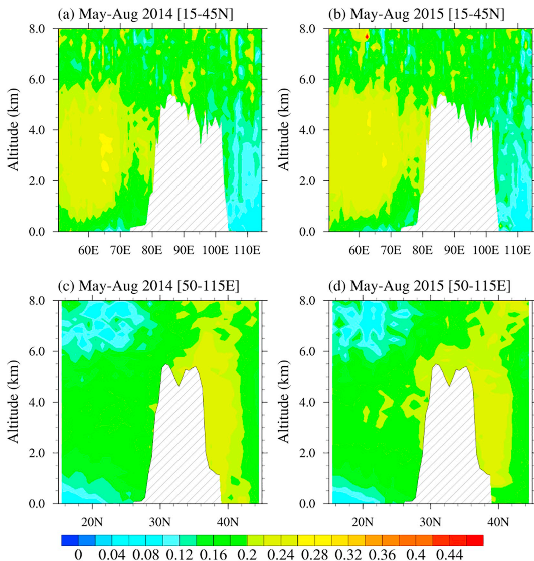
Fig. 12. Longitude-altitude cross sections and latitude-altitude cross sections of particulate depolarization ratio at wavelength of 532 nm from CALIPSO measurements in May–August 2014 (a, c) and 2015 (b, d). The latitude and longitude bounds for the average are from 15° N to 45° N and from 50° E to 115° E, respectively. The shaded parts in each plot indicate the topography of Tibetan Plateau at 30° N (a, b) and 87.5° E (c, d).
