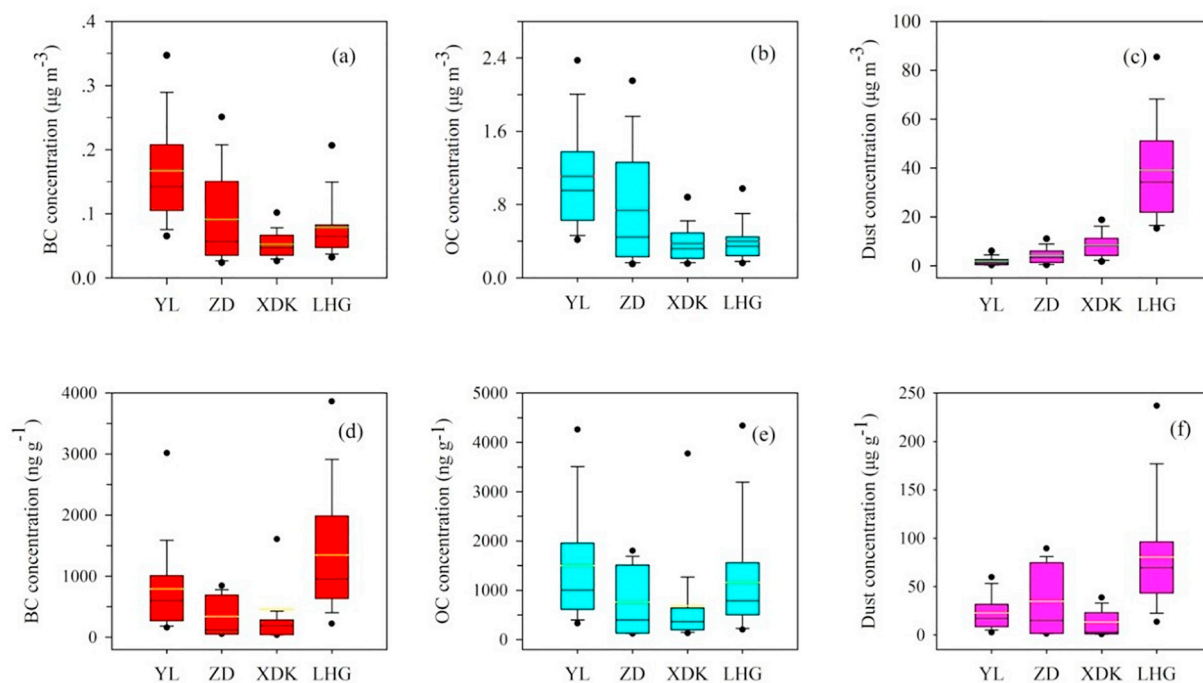
Fig. 8. Spatial difference of ILAIs concentrations in atmospheric aerosol at surface over the four glaciers (a, b, c) and in the surface-aged snow of glaciers (d, e, f) on the TP. The average ILAI contents in surface-aged snow of ZD glacier (Li et al., 2018), XDKMD glacier (Li et al., 2017), LHG glacier (Zhang et al., 2017), and Baishui glacier on Mt. Yulong (YL) are presented in the figure.
