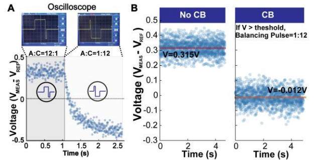
Fig. 5. A. Transient voltage response at the measurement electrode to the switching of the pulse output profile without the charge balancing mechanism: 1) Anodic vs Cathodic=12:1, 2) Anodic vs Cathodic=1:12. B. The effect of charge-balancing. Measured steady-state voltage is 0.315 \pm 0.048 when there is no charge-balancing, and -0.012 \pm 0.052 when there is active charge balancing. The voltage is measured once per each cycle as in Fig. 3B. CB: Charge-Balancing. *Each dot represents a voltage sample taken at 80% of each duty cycle of the 200 Hz pulse train.
