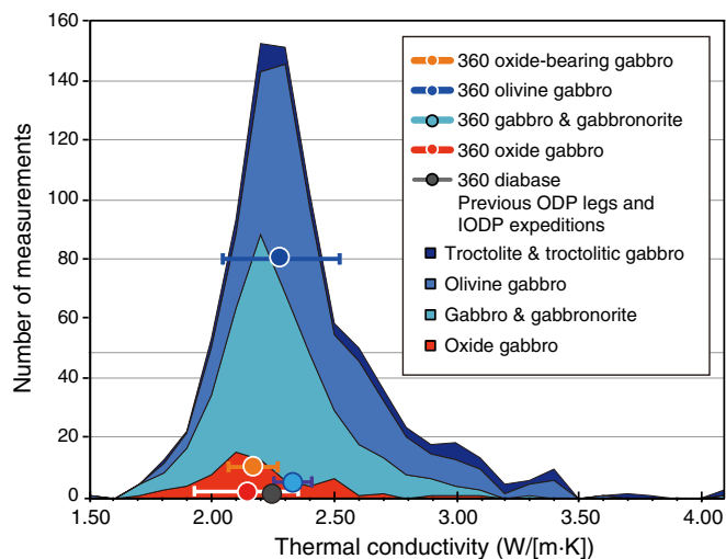
Figure F181. Thermal conductivity measurements in ODP, Integrated Ocean Drilling Program, and IODP gabbroic cores. Cumulative curves are compiled data from fast- and slow-spread crust: Hess Deep at ODP Site 894 (Gillis, Mével, Allan, et al., 1993), Hole 1256D (Teagle, Alt, Umino, Miyashita, Banerjee, Wilson, and the Expedition 309/312 Scientists, 2006), Hole 735B at SWIR (Robinson, Von Herzen, et al., 1989; Dick, Natland, Miller et al., 1999), MARK area (Cannat, Karson, Miller, et al., 1995), Mid-Atlantic Ridge in 15°N area (Kelemen, Kikawa, Miller, et al., 2004), and Site U1309 (Atlantis Massif) on Mid-Atlantic Ridge at 30°N (Blackman, Ildefonse, John, Ohara, Miller, MacLeod, and the Expedition 304/305 Scientists, 2006). Large circles = average Expedition 360 thermal conductivity values, horizontal bars = range of Expedition 360 thermal conductivity values.
