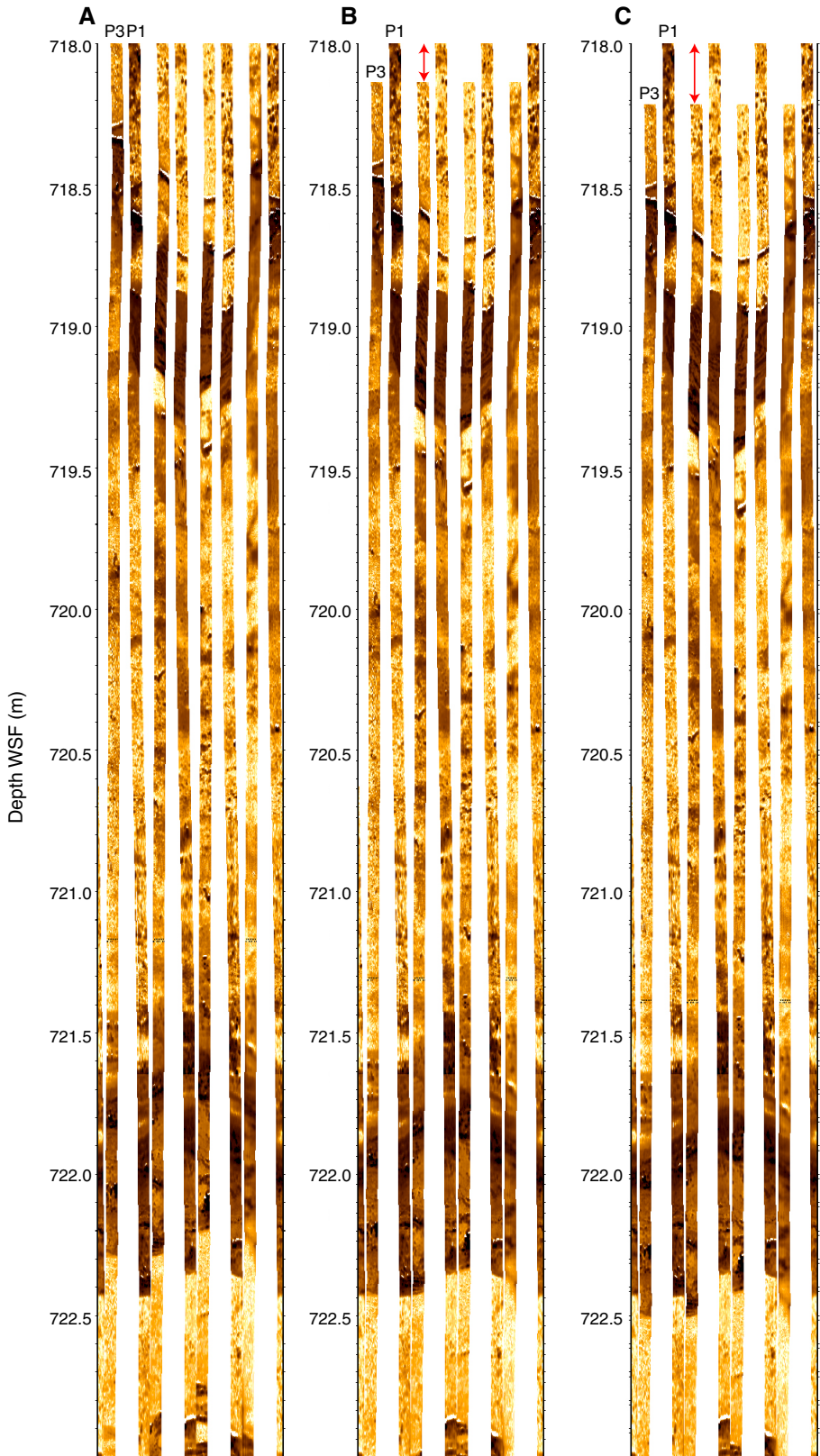
Figure F186. Example of FMS data, as processed by Lamont-Doherty Earth Observatory (LDEO) and received on board, from a single 5 m interval in the deepest section of Hole U1473A. Images from two passes (P1 and P3) are shown next to each other, with different depth shifts (see text for further discussion). A. No additional depth shift; Passes P1 and P3 are plotted against depth after LDEO processing. Features recorded by the two passes are offset. B. Pass P3 was shifted down manually (red arrow) to align geologic features in the lower portion of the interval. Offset between the 2 passes remains visible at top of interval. C. Pass P3 was shifted further down (red arrow) to align geologic features in the upper part of interval. In this case, the features in the lower part are offset again.
