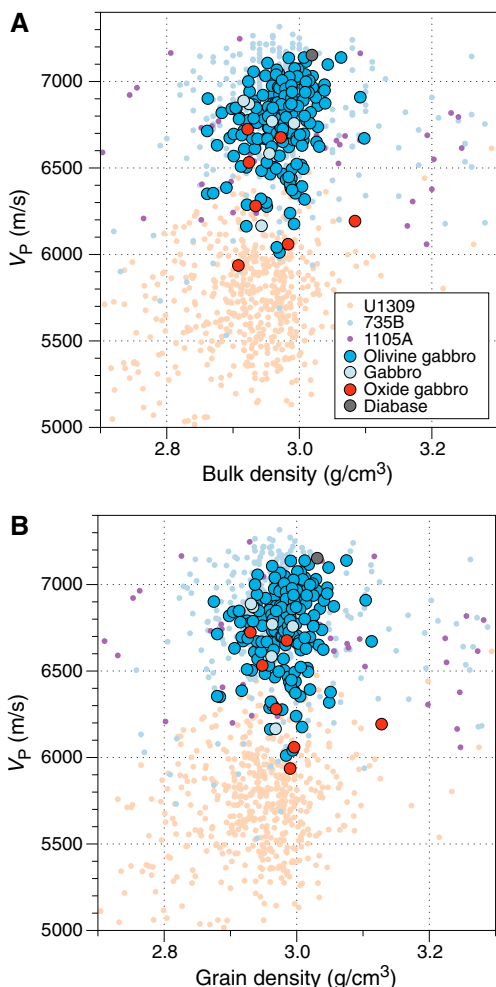
Figure F177. Compressional velocity vs. (A) bulk density and (B) grain density in Hole U1473A samples, compared with previous data in gabbroic sections from Hole 735B at Atlantis Bank (Robinson, Von Herzen, et al., 1989; Dick, Natland, Miller et al., 1999) and Site U1309 (Atlantis Massif) on the Mid-Atlantic Ridge at 30°N (Blackman, Ildefonse, John, Ohara, Miller, MacLeod, and the Expedition 304/305 Scientists, 2006). Data from Hole U1473A are color-coded by lithology.
