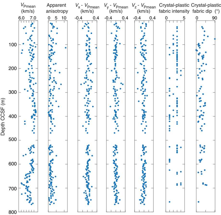
Figure F179. Downhole variation in V_p anisotropy in core samples, Hole U1473A. Mean V_p (average of V_x , V_y , and V_z ), apparent anisotropy ( 100\% \times [\max(V_i) - \min(V_i)]/V_{pmean} , where i = x, y, \text{ or } z ), difference of sample V_x relative to sample V_{pmean} , difference of sample V_y relative to sample V_{pmean} , difference of sample V_z relative to sample V_{pmean} , CPF deformation intensity estimated for section halves by structural geology team for intervals where measured cubes were taken (0 = undeformed, 1 = foliated, 2 = porphyroclastic, 3 = protomylonitic, 4 = mylonitic, 5 = ultramylonitic), and CPF foliation dip (degrees from horizontal) estimated for section halves by structural geology team.
