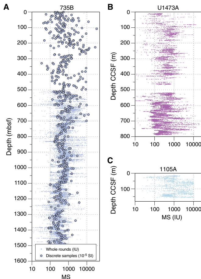
Figure F176. Comparison of magnetic susceptibility measurements on cores from Holes 735B, 1105A, and U1473A, Atlantis Bank. A. Whole-round and discrete sample data, Hole 735B. No whole-round magnetic susceptibility data were obtained during ODP Leg 118. Filtered whole-round data, (B) Holes U1473A and (C) 1105A.
