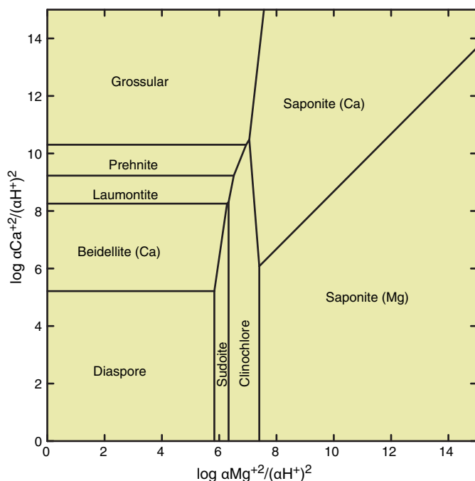
Figure F95. Activity diagram for simplified \text{MgO-CaO-Al}_2\text{O}_3\text{-SiO}_2\text{-H}_2\text{O} system at 200^\circ\text{C} and 15 bar, and silica activity in equilibrium with quartz. High Mg activities can stabilize minerals of the chlorite (sudaite and clinocllore) and smectite (saponite) group. Grossular and prehnite are stable at lower Mg activities. Activity diagram plotted using Geochemist Workbench (Bethke and Yeakel, 2015) with the Thermoddem database by Blanc et al. (2012).
