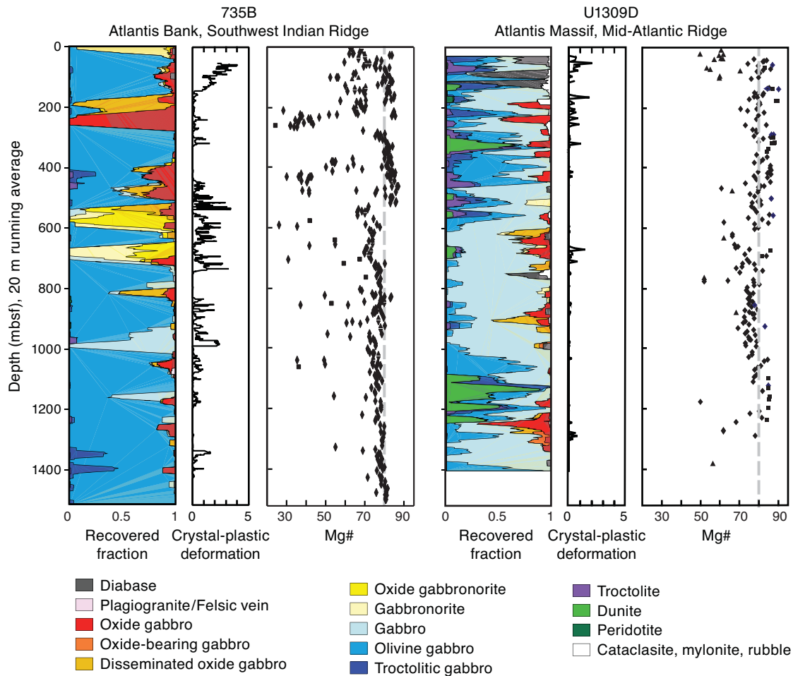
Figure F6. Running average (20 m) of lithologies, crystal-plastic deformation intensity, and whole-rock Mg# ( [(\text{Mg} \times 100)/(\text{Mg} + \text{Fe})] ) for Holes 735B and U1309D (Mid-Atlantic Ridge at 30°N), modified from Dick et al. (2000), Blackman et al. (2011), and Expedition 304/305 Scientists (2006). Different symbols for points in whole-rock Mg# diagram represent different lithologies based on modal mineralogy; definitions can be found in the Leg 118 and 176 Initial Reports volumes (Robinson, Von Herzen, et al., 1989; Dick, Natland, Miller, et al., 1999) and the Expedition 304/305 Proceedings volume (Blackman, Ildefonse, John, Ohara, Miller, MacLeod, and the Expedition 304/305 Scientists, 2006). These sections represent descriptions from two different scientific parties, and although both followed American Geophysical Institute conventions on nomenclature, exact definitions for each lithology described may vary. Lithologic plots differ from those previously presented, as the lithologies from both holes were grouped in the same manner to facilitate comparison. Gray dotted lines at Mg# = 80 emphasize overall chemical differences between the sections. Primary melts emerging from the mantle would be in equilibrium with gabbroic cumulates and dunites with an Mg# \geq 90 , largely missing from both sections.
