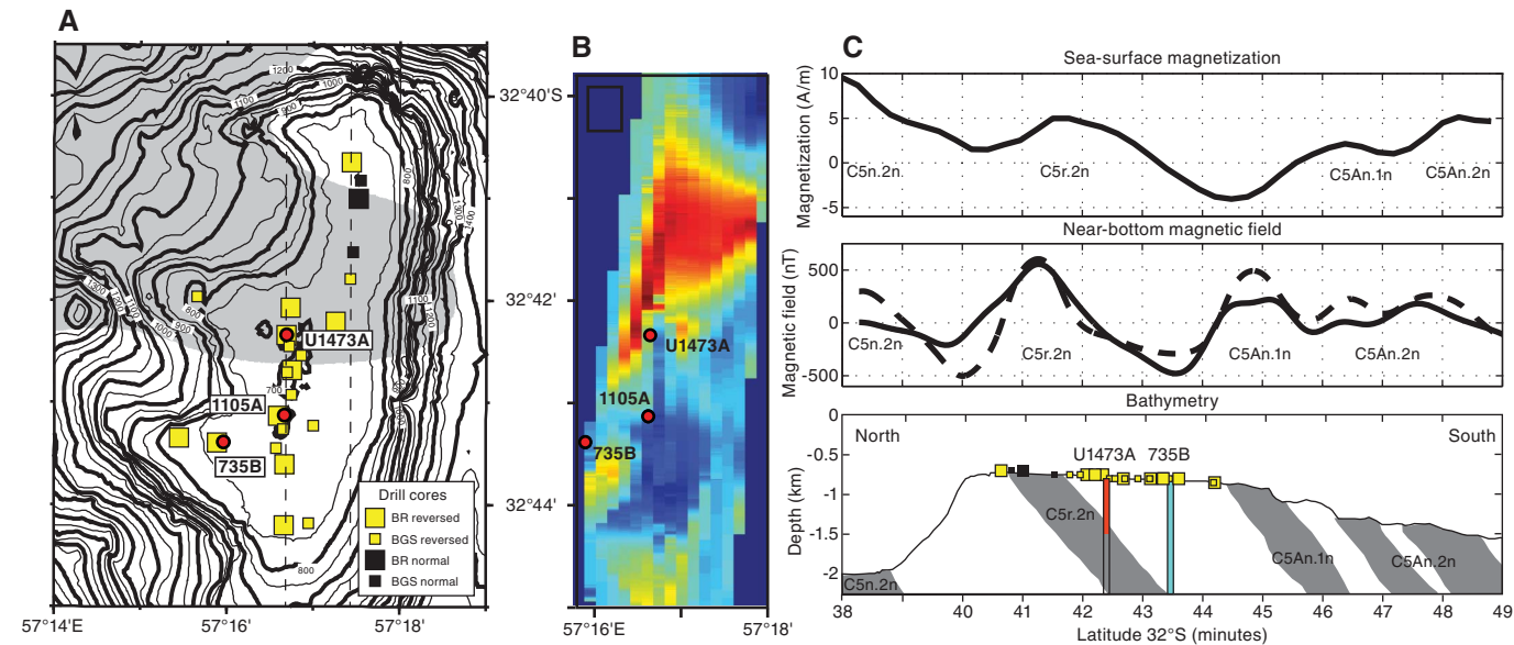
Figure F7. A. Location and magnetization of Atlantis Bank platform drill cores. B. Contoured deep-towed magnetization. C. Magnetic anomaly models with positions of Holes 735B and U1473A.
