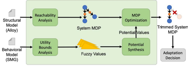
Figure 4: THALLIUM Overview
