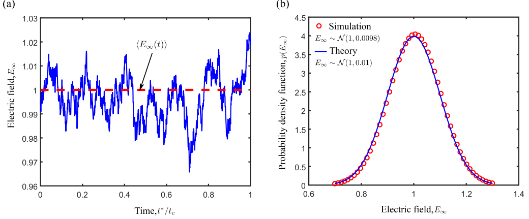
FIG. 2. (a) A simulated electric field with variance G_w\lambda = 0.1 . The solid line is an average over 100 realizations of the algorithm over the initial distribution of \epsilon_0 . The dashed line shows the mean value of the fluctuations. (b) Probability density function of the numerically computed (circles) and theoretically predicted (solid line) electric field at t = 1 .
