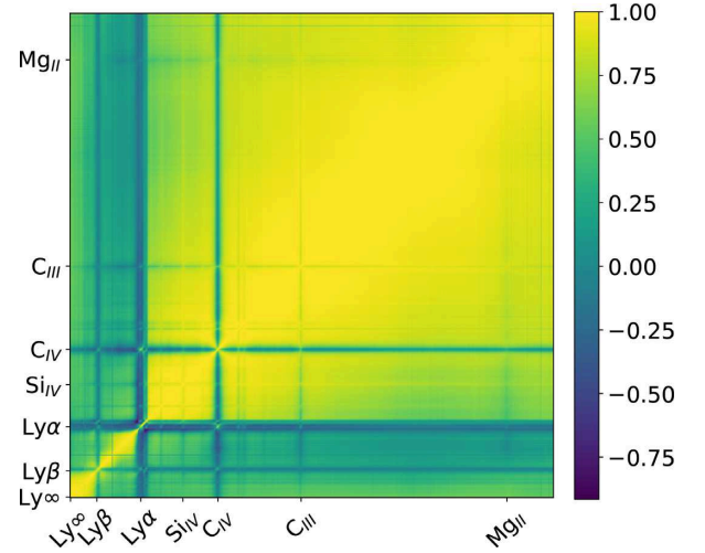
Figure 3. The trained correlation matrix K , with the \lambda range from 910 to 3000 Å. We have normalized the diagonal elements to be unity. The values in the matrix range from -1 to 1 , representing the correlation between \lambda and \lambda' in the QSO emission function.
