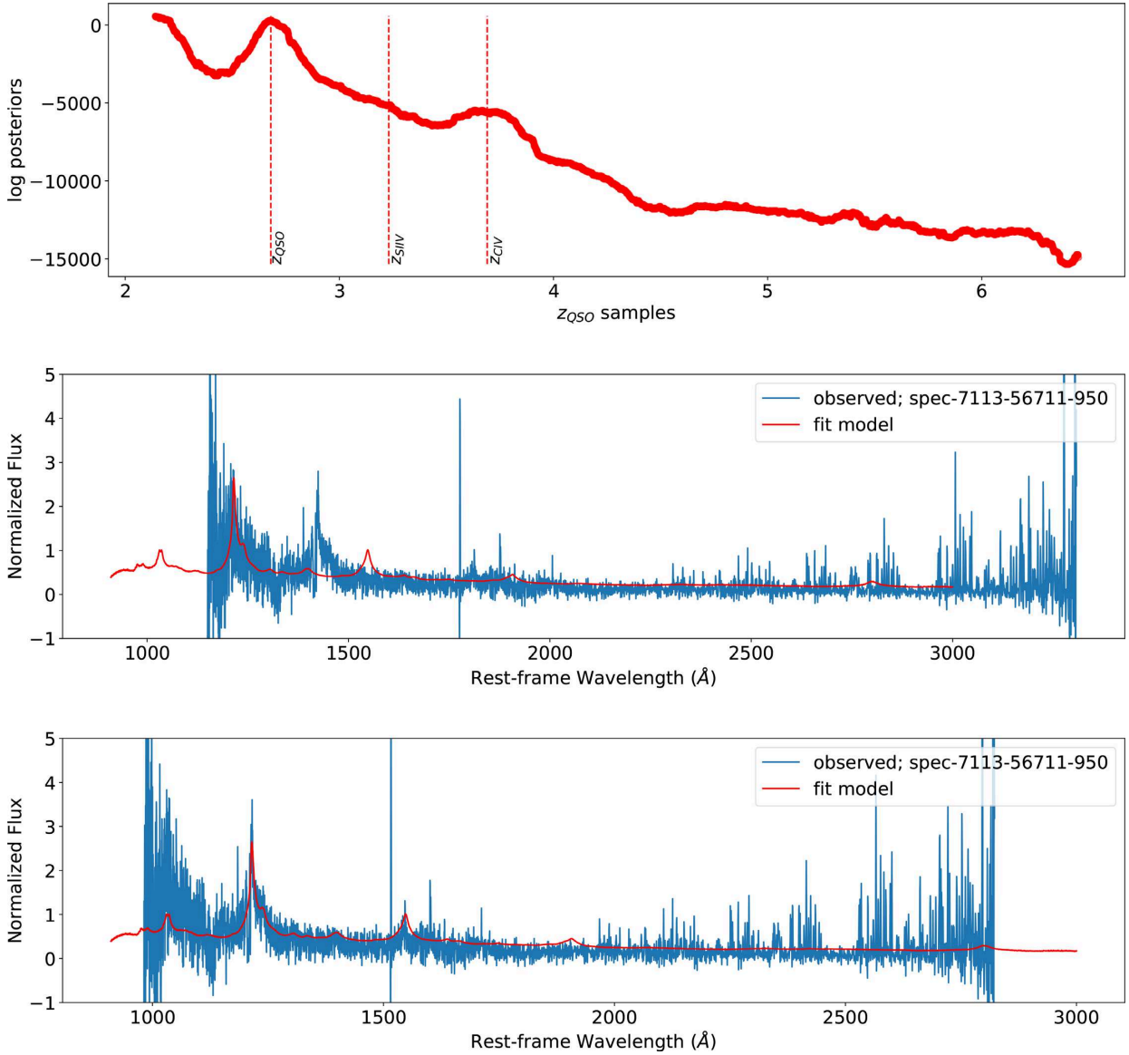
Figure 6. (Top) The sample posterior p(z_{\text{QSO}}|x, D^0) for a QSO with thingID = 544031279. The catalogue redshift is labelled as z_{\text{QSO}} . Vertical dashed lines indicate the redshifts associated with samples at particular emission peaks. For example, the redshift resulting from trying to fit the true Lyman \alpha peak on to the observed C IV peak is shown as z_{\text{CIV}} . (Middle) The rest-frame spectrum using z_{\text{MAP}} . (Bottom) The rest-frame spectrum using the SDSS visual inspection redshift z_{\text{VI}} . We use z_{\text{VI}} as it is the method with the lowest failure rate. The MAP value of our catalogue fits the Lyman \alpha peak with what is really O VI.
