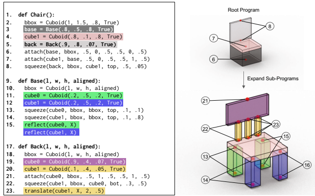
Fig. 3. An example SHAPEASSEMBLY program and the shape that it generates. Parts are colored according to the line of the program which instantiates them, and attachment points are numbered accordingly. In the top shape, we show the executed Chair program without hierarchy. In the bottom shape, we show the Chair program executed hierarchically with its sub-programs (Base and Back). For instance, the light grey back part is expanded into the purple back surface and gold slats.
