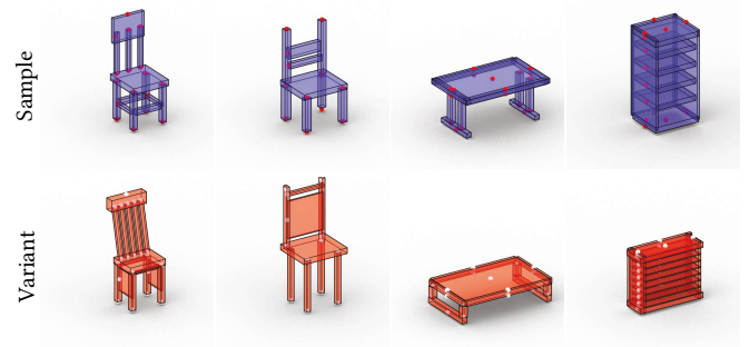
Fig. 8. Programs, by way of representational form, allow for easy semantic editing of generated output. Each column shows a sample from our model in the top row. In the bottom row we create a variant with the same structure, but different geometry, by editing only the continuous parameters of the program. Program text can be found in the supplemental material.
