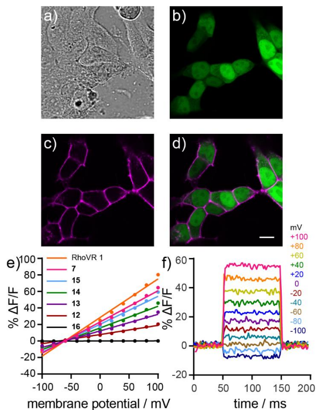
Figure 2. Cellular labeling and voltage sensitivity of RhoVR 1 -PEG x -Halo compounds. a) DIC image of HEK293T cells expressing nuclear EGFP stained with 15 . b) Confocal fluorescence image of HaloTag expressing cells from (a) as indicated by nuclear EGFP fluorescence. c) Confocal fluorescence image showing the fluorescence of 15 from cells in (a) . d) Merge of fluorescence from EGFP (green) and 15 (magenta), demonstrating the highly selective localization of 15 to HaloTag expressing cells. Scale bar is 10 \mu\text{m} . e) Plot of % \Delta F/F vs final membrane potential for RhoVR 1 , 7 and RhoVR 1 -PEG x -Halo derivatives 12-16 ( n=3-9 , error bars not shown). f) Plot of the fractional change in fluorescence of 15 vs time for 100 ms hyper- and depolarizing steps ( \pm 100 mV in 20 mV increments) from a holding potential of -60 mV for single HEK293T cells under whole-cell voltage clamp mode.
