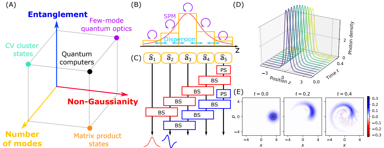
Figure 2. (A) An illustration of the different facets which contribute to the complexity of simulating continuous-variable quantum systems. Representative states/systems 59–62 belonging to each corner of the cube (marked by circles) are shown. (B) Quantum pulse propagation through a nonlinear medium is modeled as interacting quantum fields on discretized spatial bins. (C) Cascaded applications of beamsplitter (BS) and phase-shifter (PS) operations on an MPS can demultiplex nonlocal supermodes into local spatial bins. (D) Time evolution of the photon density distribution of a coherent-state Kerr soliton in a \chi^{(3)} nonlinear waveguide. (E) Dynamics of the Wigner function of the solitonic mode. Simulations for (D) and (E) were performed using time-evolving block decimation based on MPS. 63
