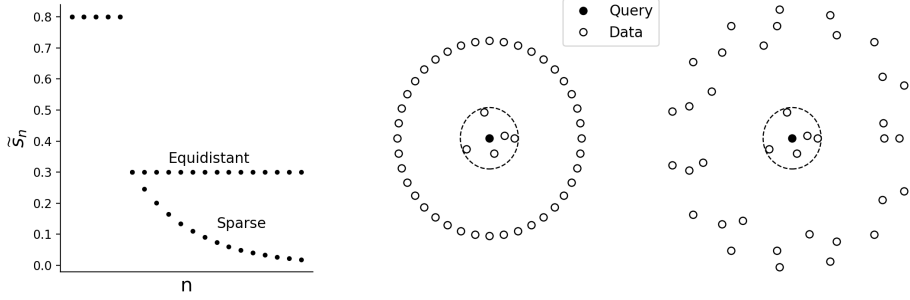
Figure 1. Geometric interpretation of B and \Delta . \Delta characterizes the gap between the v nearest neighbors, while B characterizes whether s is sparse. The worst-case situation occurs when all points are equidistant to the query (center). However, if s is already sparse, then far fewer points in the dataset are near the query (right).
