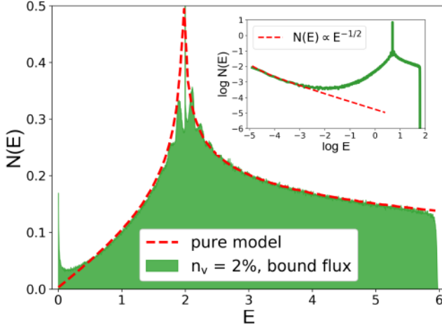
FIG. 5. (Color online) Density of states in the bound-flux sector with 2% true vacancies ( J' = 0 ). The density of states is first calculated for each L = 40 realization by Eq. (6), and then averaged over 4000 disordered realizations. The red dashed line shows the analytical density of states of the pure Kitaev honeycomb model without fluxes and vacancies. The spectral weight is transferred towards the low-energy region from the high-energy region near the Van Hove singularity. The inset shows the data in base-10 logarithmic scales and demonstrates the N(E) \sim E^{-1/2} behavior at low energies.
