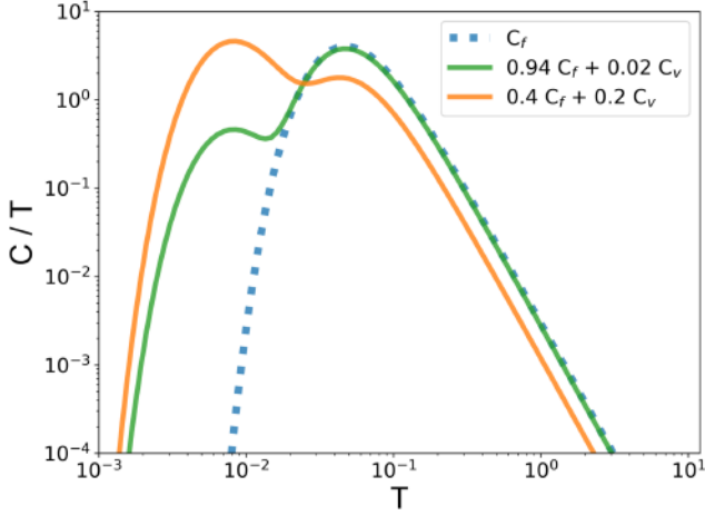
FIG. 15. (Color online) Schottky model of specific heat for independent flux excitations. The high-temperature peak comes from the normal flux excitation on the hexagonal plaquette, and the low-temperature peak comes from vacancy flux excitations.
