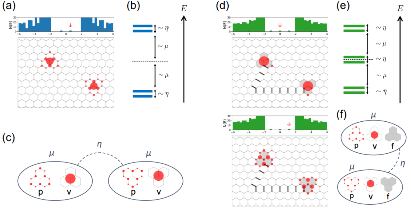
FIG. 14. (Color online) Hybridization between the low-energy modes around two vacancies in the zero-flux sector (a)-(c) and the bound-flux sector (d)-(f). The densities of states and the real-space wave functions of the low-energy modes are calculated for L = 20 systems with J' = 0.01 and \kappa = 0.2 . Note that in the density of states (a) and (d), each peak inside the gap (pointed by a red arrow) contains two states with a very small energy-level split. This split corresponds to the energy scale \eta in the spectra of the simple model Hamiltonians \delta\mathcal{H}_{\text{zero}} (16) and \delta\mathcal{H}_{\text{bound}} (17), which are shown in (b) and (e). In (c) and (f), we present cartoon pictures of the hybridization. The labels p , v , and f refer to the peripheral mode ( p -mode), the vacancy mode ( v -mode), and the flux mode ( f -mode).
