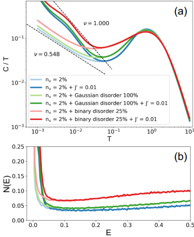
FIG. 13. (Color online) Effect of bond disorder for a 2% concentration of vacancies. For Gaussian disorder, a normal random distribution of coupling strengths with standard deviation 0.25 is applied to all bonds. For binary disorder, 25% of the bonds obtain additional coupling strength \delta J = \pm 0.8 so that the total strength becomes either 0.2 or 1.8. All results are calculated in the bound-flux sector, averaged over 4000 disordered realizations of L = 40 .
