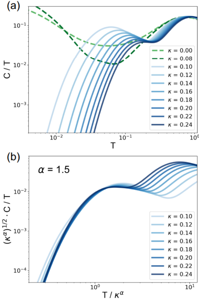
FIG. 11. (Color online) Specific heat C/T calculated from the Majorana fermion spectrum in Fig. 10. (a) Temperature dependence of C/T for various three-spin couplings \kappa . The green (blue) dashed (solid) lines are calculated for the bound-flux (zero-flux) sector, which is the ground-state flux sector for small (large) \kappa . (b) Scaling plot of the curves with large values of \kappa for which the ground-state flux sector is the zero-flux sector.
