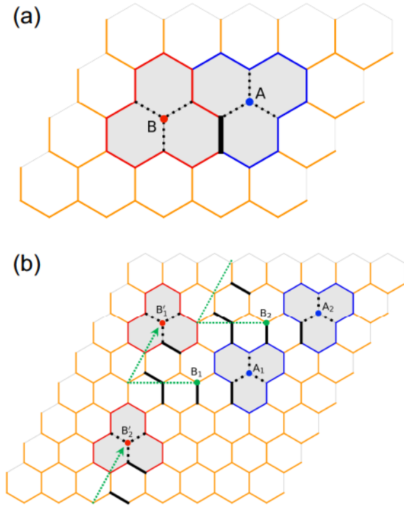
FIG. 3. (Color online) The recipe for creating vacancies with bound fluxes. (a) Randomly place one pair of vacancies on the lattice. Flip one shared link variable (thick black line) such that two fluxes are created and attached to the two vacancy plaquettes. (b) Randomly move one of the vacancies in the pair, and flip a string of link variables along the path, such that the fluxes are always bound to the vacancies. After the migration, place another pair of vacancies with fluxes and repeat the same process.
