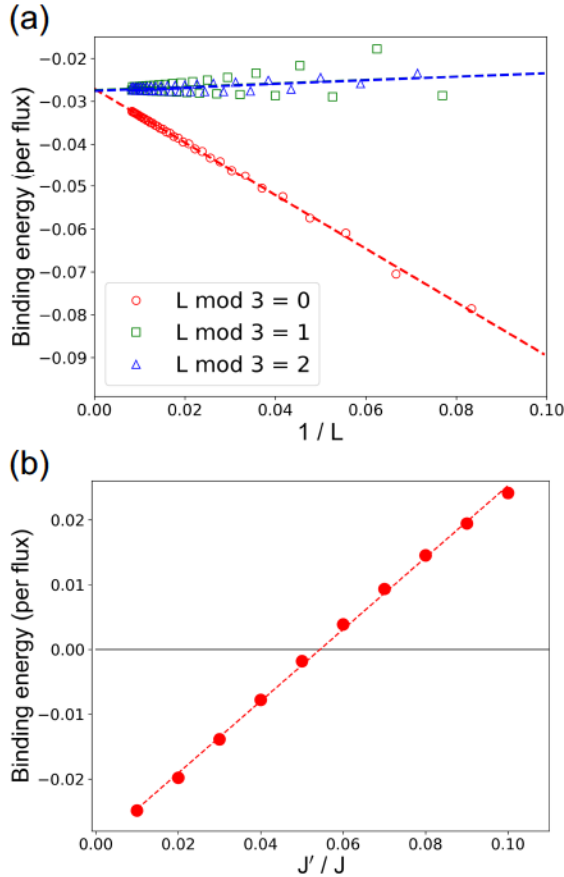
FIG. 2. (Color online) Binding energy of a flux to a vacancy, calculated by Eq. (8). (a) The flux-binding energy converges to E_{\text{bind}} = -0.0268J in the thermodynamic limit by extrapolation. System sizes are classified by L \bmod 3 since they have different rates of convergence. The binding energies are calculated for finite-size systems up to L = 120 with J' = 0 . (b) The J' dependence of the flux-binding energy. By interpolation, the critical value of J' is estimated as 0.0544J , which sets the upper limit of the flux-binding effect.
