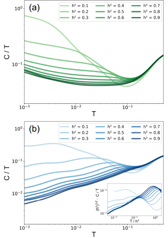
FIG. 12. (Color online) Effect of dangling Majorana fermions for a 2% concentration of true vacancies. The specific heat C/T is shown for the bound-flux sector (a) and the zero-flux sector (b). The magnetic field is applied along the z axis so that it couples the dangling Majorana fermion \hat{b}^z to the rest of the system. The inset of (b) shows the field scaling and the collapse of the curves for higher fields.
