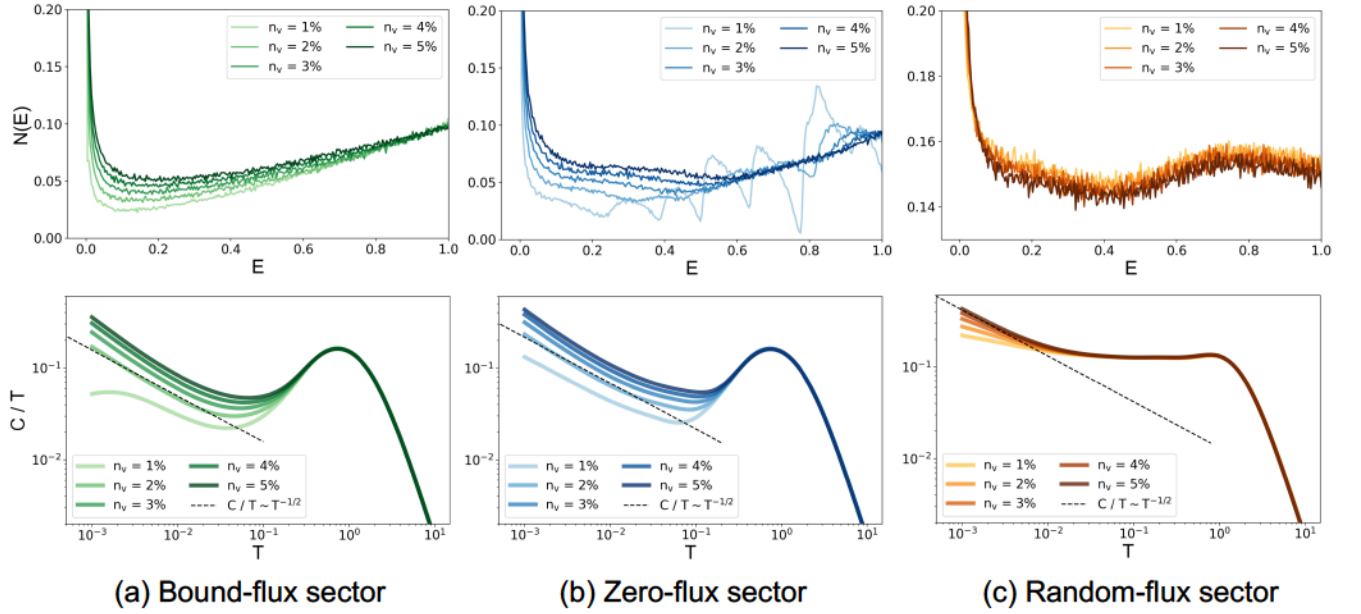
FIG. 7. (Color online) The low-energy density of states (Eq. (6)) and fermionic specific heat (Eq. (9)) with different concentrations of true vacancies ( J' = 0 ) in the (a) bound-flux, (b) zero-flux, and (c) random-flux sectors. All the three cases show a clear upturn in both the density of states and C/T . The results are averaged over 4000 disordered realizations of L = 40 .
