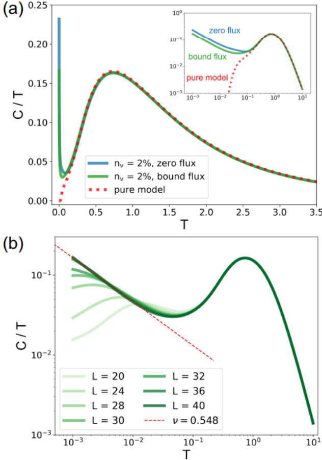
FIG. 6. (Color online) (a) Specific heat C/T for L = 40 systems calculated from the fermionic density of states (Eq. (9)). Compared to the pure Kitaev model without fluxes and vacancies, adding 2% true vacancies ( J' = 0 ) leads to a clear upturn in both the bound-flux and the zero-flux sectors. The inset shows the data in logarithmic scales. (b) The system-size dependence of C/T . The low-temperature upturn becomes more robust for larger systems due to the reduction of the finite-size effect. The curves are averaged over 4000-10000 disorder realizations, depending on the system size.
