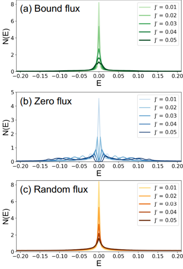
FIG. 8. (Color online) Density of states (Eq. (6)) for various quasivacancy coupling strengths J' with a concentration n_v = 2\% of quasivacancies. The low-energy states induced by the quasivacancies are accumulated around the Dirac point of the Majorana spectrum. The zero-energy peak is suppressed for larger J' due to the stronger coupling to the bulk. For the zero-flux sector, a pseudogap gradually forms by the hybridization of the quasivacancy mode and the quasilocalized mode around the same quasivacancy. The results are averaged over 4000 disordered realizations of L = 40 .
