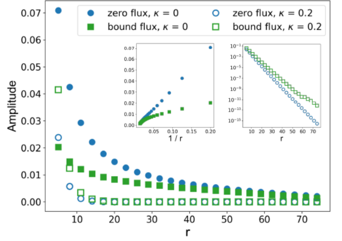
FIG. 9. (Color online) The spatial dependence of wave function amplitude of vacancy-induced modes. The distance r is in the unit of hexagonal lattice constant. The inset shows the 1/r dependence for zero-flux sector with \kappa = 0 , and the exponential decay for both sectors under finite \kappa .
