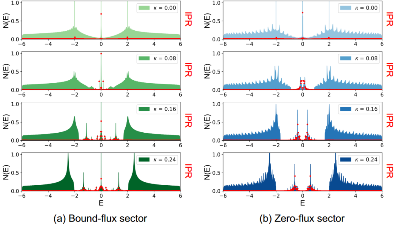
FIG. 10. (Color online) Density of states (Eq. (6)) and inverse participation ratio (IPR) (Eq. (10)) for different three-spin couplings \kappa with fixed J' = 0.01 and n_v = 2\% . The IPR results are intensified by a factor of 2 in order to be comparable to the density of in-gap states. (a) Bound-flux sector: three broad peaks of in-gap states appear when a bulk gap opens for \kappa > 0 . (b) Zero-flux sector: only two broad peaks appear inside the gap. The crucial difference in the number of peaks comes from the hybridization of localized states in the low-energy subspace and, in particular, from the presence of Majorana zero modes in the bound-flux sector. The results are averaged over 4000 disordered realizations of L = 40 .
