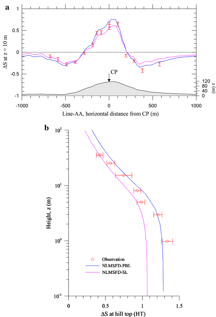
Fig. 12 Comparisons between model calculations (Weng and Taylor 2011) and Askervein 1983 field data (Taylor and Teunissen 1985) a 10-m mean wind speeds along transect AA. b hill-top speed-up profiles
