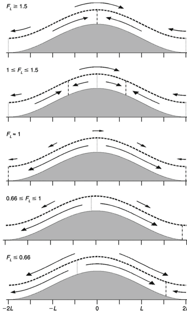
Fig. 10 Schematic showing forces on flow deep within and just above the canopy on a sinusoidal ridge from Fig. 9. For a range of boundary layer stabilities as quantified by the Froude number F_L . Above the canopy top (dashed line) arrows indicate the hydrodynamic pressure gradient only. Within the canopy (below the dashed line) arrows indicate the balance between the hydrodynamic and hydrostatic pressure gradients. Arrow lengths indicate the magnitude of the forcings. Dotted lines indicate regions of divergence within the canopy (and descent at canopy top). Dash-dotted line indicate regions of convergence in the canopy and ascent at canopy top
