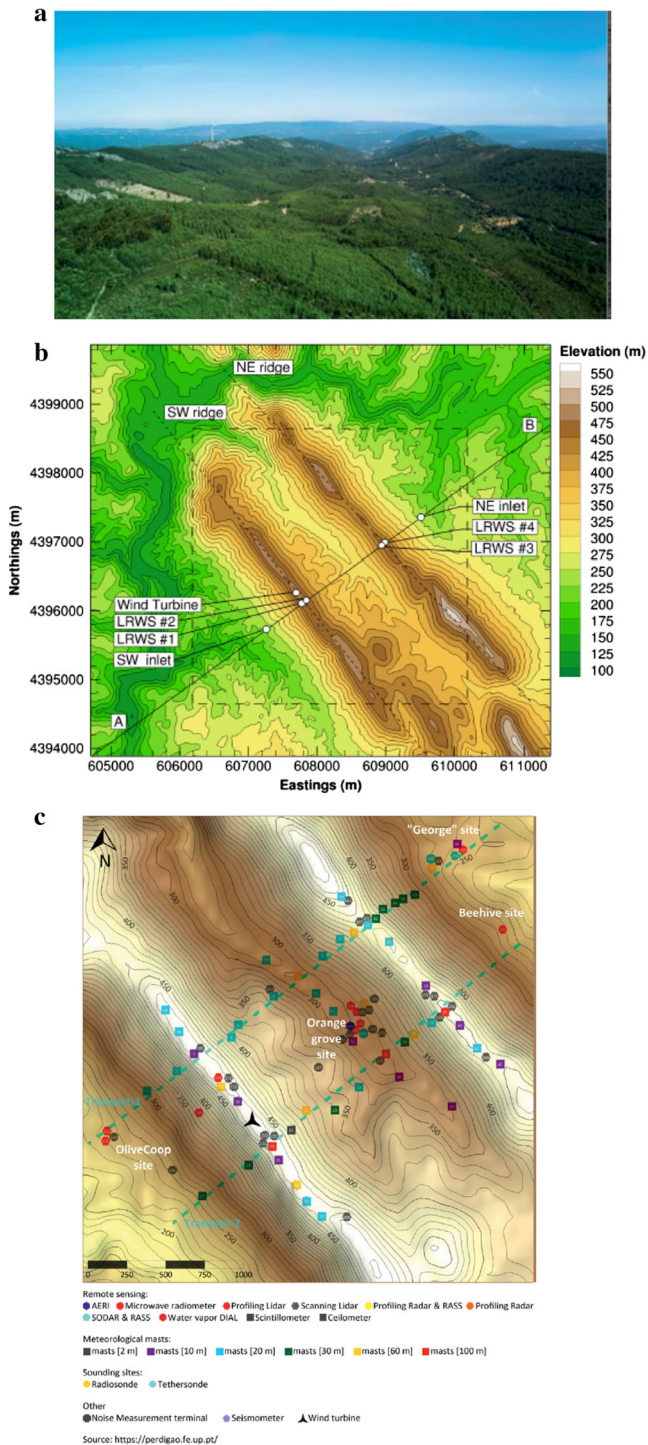
Fig. 13 Perdigo Field site, Portugal. a photo, b contour map of the region, c sensor locations
