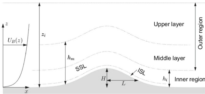
Fig. 2 Definitions of hill scales and HLR88 layers. SSL denotes the shear-stress layer and ISL the inner surface layer. h_i is the depth of the shear-stress layer and h_m the middle layer depth. U_B(z) is the undisturbed approaching wind profile
