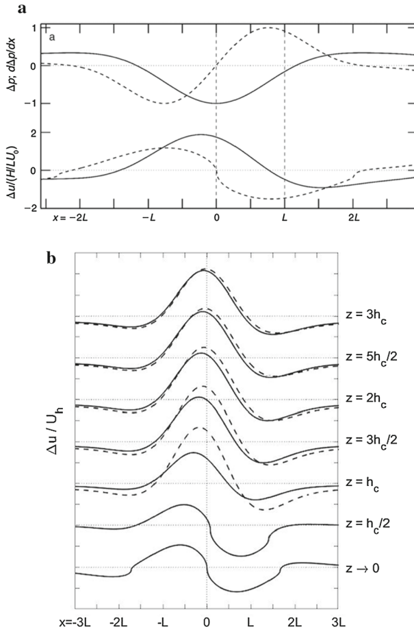
Fig. 4 a Phasing of forcing terms across the hill. Upper part of the panel shows variation across the hill of the pressure perturbation (solid line) and the pressure perturbation gradient (dashed line); perturbations have been normalized by the maximum value taken across the hill. The lower part of the panel shows variation of the normalized wind-speed perturbation across the hill. Solid line is at z = 3h_c above the canopy, which is nearly in phase with the pressure perturbation. The dashed line is at z = h_c/2 within the canopy, which is in phase with the pressure perturbation gradient. b velocity perturbations along streamwise transects through the shear-stress layer and down into the canopy. Solid line denotes RB04 solution and dashed line HLR88
