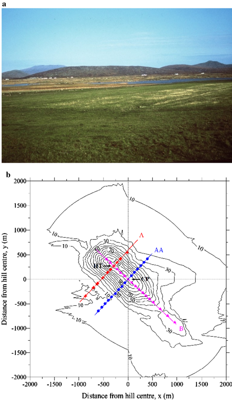
Fig. 11 Askervein. a Photo, by Hans Teunissen, taken from the 50-m reference mast. b topographic contours (m) and mast positions
