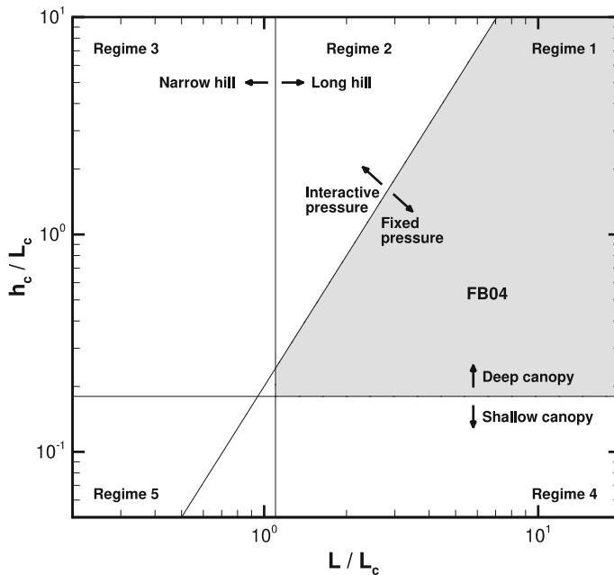
Fig. 5 Length-scale regimes imposed by hill geometry and canopy morphology for low hills where H \ll L , after Poggi et al. (2008). Hills are classified as narrow or long and canopies as deep or shallow
