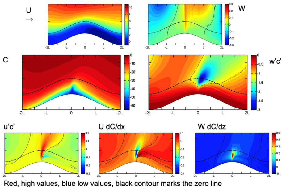
Fig. 7 Numerical calculation of scalar transport driven by the RB04 model. Cosine hill profile with H = 20 m, L = 400 m, h_c = 20 m, L_c = 30 m, u^*/U(h_c) = 0.3 , S(z) = S_0 = \text{constant} for h_c > z > 0 . S_0 = -1 . Figures from IN Harman
