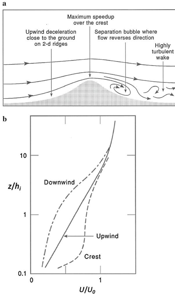
Fig. 1 Main features of flow over low hills: a flow over a 2D ridge. b perturbation to an upstream logarithmic mean velocity profile. See Fig. 2 for definitions of h_i and U_0 . (after Kaimal and Finnigan 1994)
