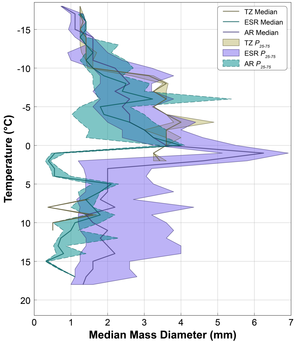
977 Fig. 5: As in Fig. 2, but with vertical profiles of D_{mm} (mm).
