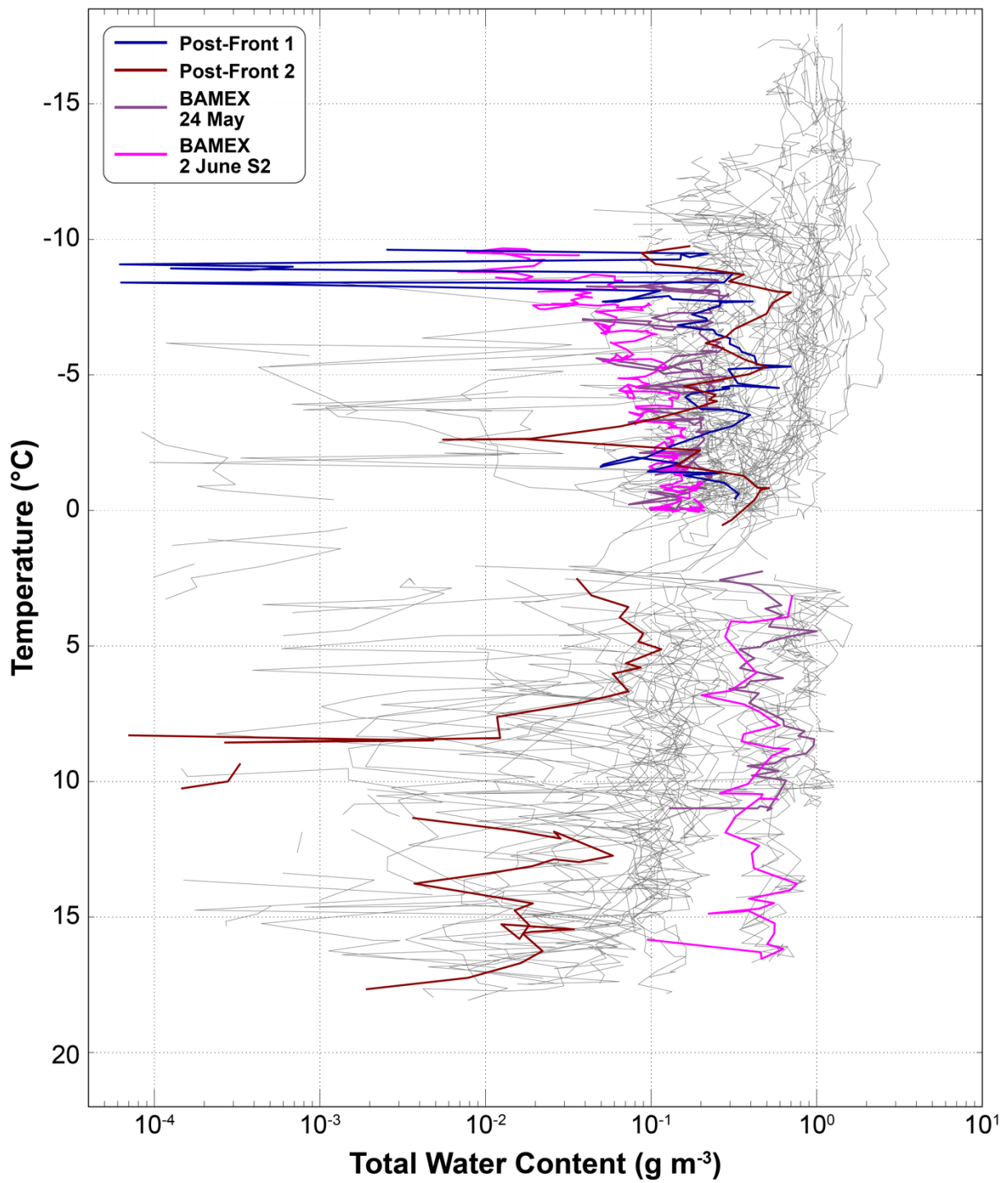
1007 Fig. 17: As in Fig. 16, but with vertical profiles of TWC ( \text{g m}^{-3} ).
