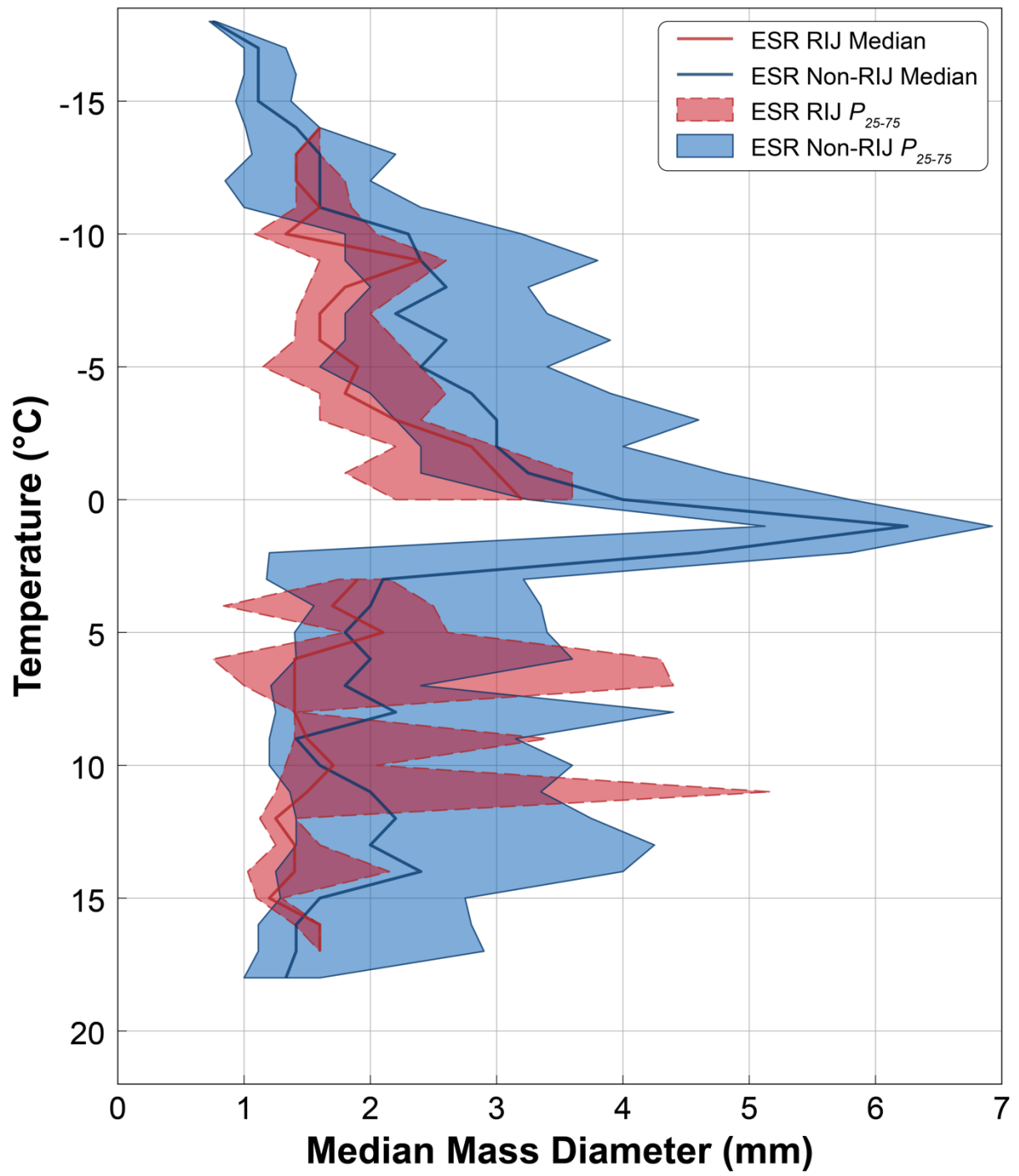
992 Fig. 12: As in Fig. 9, but with vertical profiles of D_{mm} (mm).
