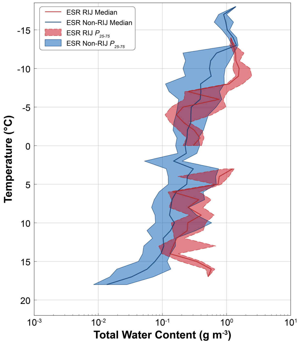
991 Fig. 11: As in Fig. 9, but with vertical profiles of TWC ( \text{g m}^{-3} ).
