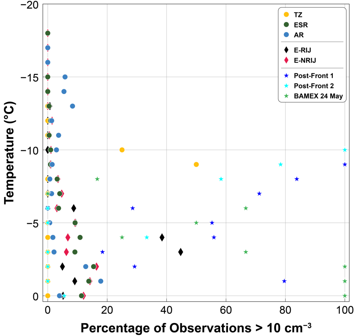
979 Fig. 7: Percentage of CDP and FSSP observations of N_t exceeding 10 \text{ cm}^{-3} as a function of T (°C). 980 The yellow, green, and blue circle markers correspond to the TZ, ESR, and AR observations, 981 respectively. The black and red diamond markers represent ESR observations in the vicinity of the 982 RIJ (E-RIJ), and non-RIJ (E-NRIJ) observations, respectively. The star markers correspond to the 983 two PECAN post-frontal spirals from 6 July 2015 (blue and cyan), and the BAMEX MCV spiral 984 from 24 May 2003 (green).
