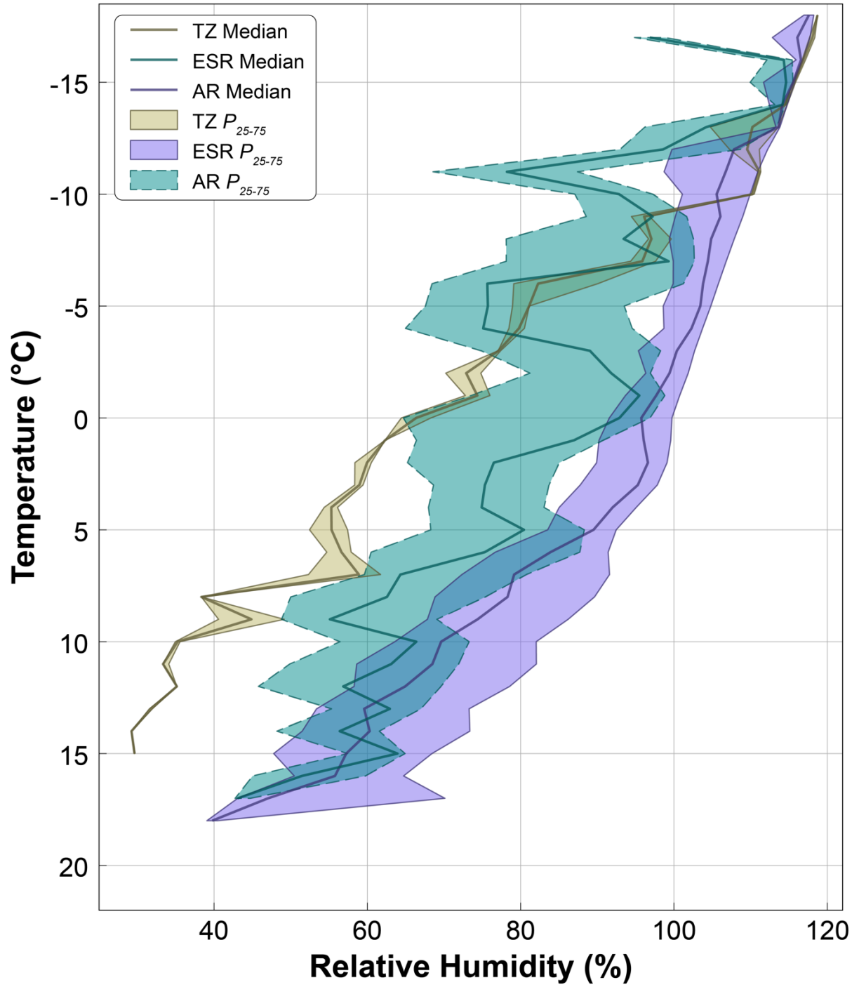
972 Fig. 2: Vertical profiles of \widetilde{RH} (%) (tan, blue, and green solid lines) and the 25 th -75 th percentile 973 range of RH (%) (filled tan, blue, and green) for the TZ, ESR, and AR MCS zones as a function of 974 T (°C). RH is with respect to ice for T \leq 0^\circ\text{C} , and with respect to liquid water for T > 0^\circ\text{C} .
