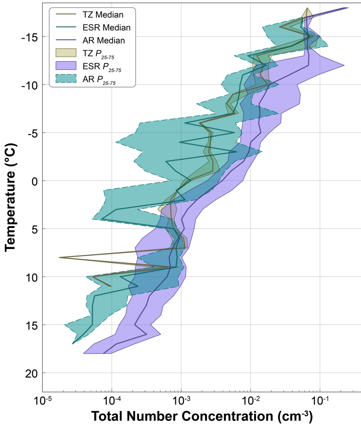
975 Fig. 3: As in Fig. 2, but with vertical profiles of N_t (cm -3 ).
