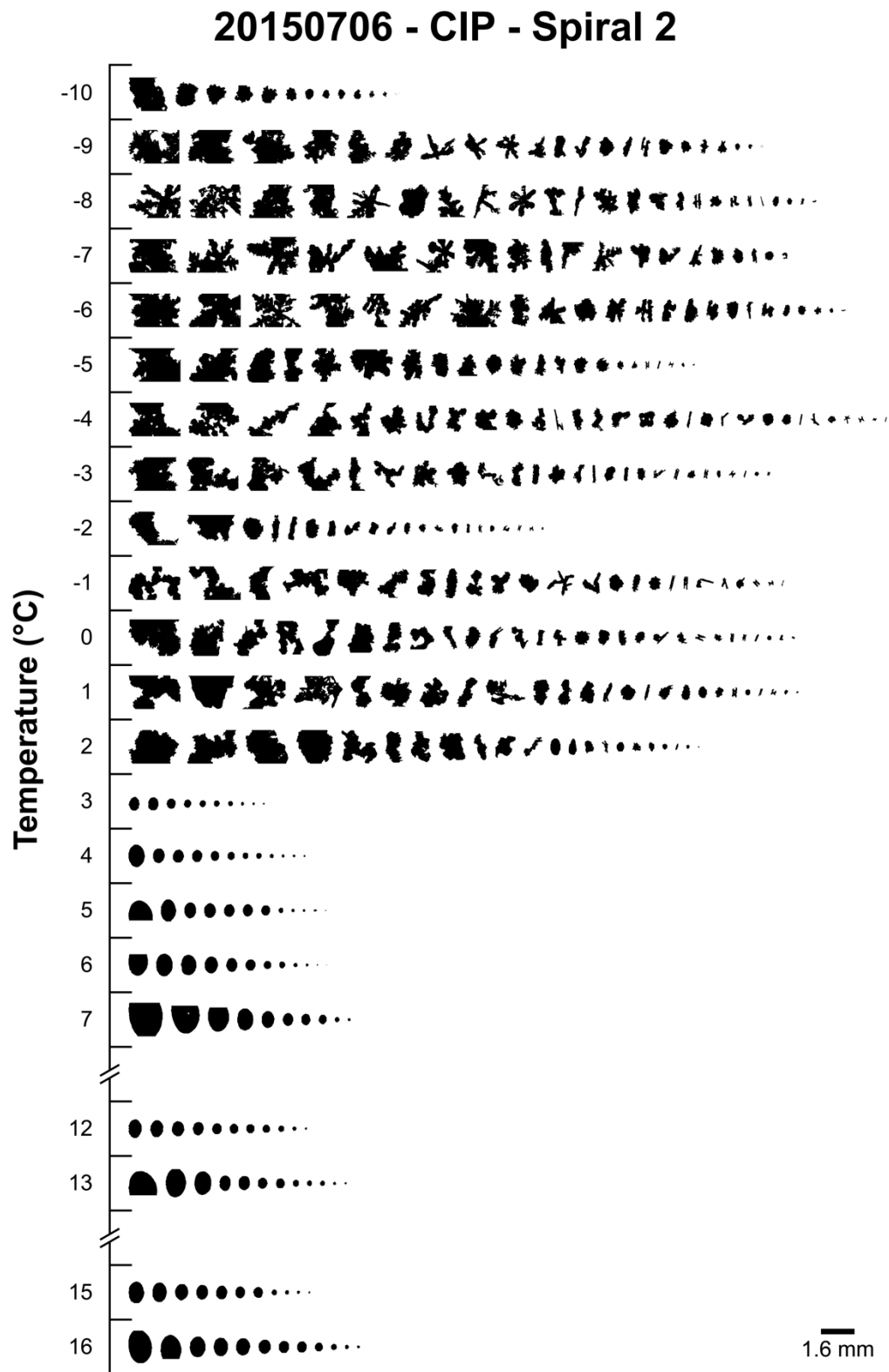
1000 Fig. 15: Representative particle images observed by the CIP as a function of T (°C) within spiral 2 1001 of the 6 July 2015 PECAN MCS.
