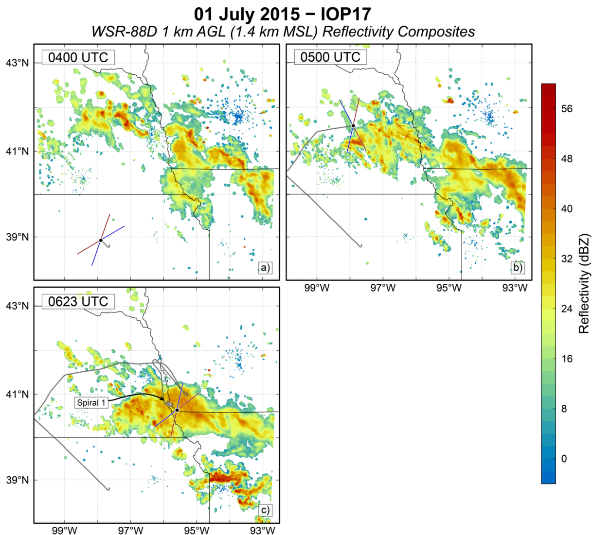
1015 Fig. A2: As in Fig. A1, though for the 1 July 2015 IOP17 MCS. Key periods discussed in the text 1016 are shown between 0400 and 0623 UTC.
