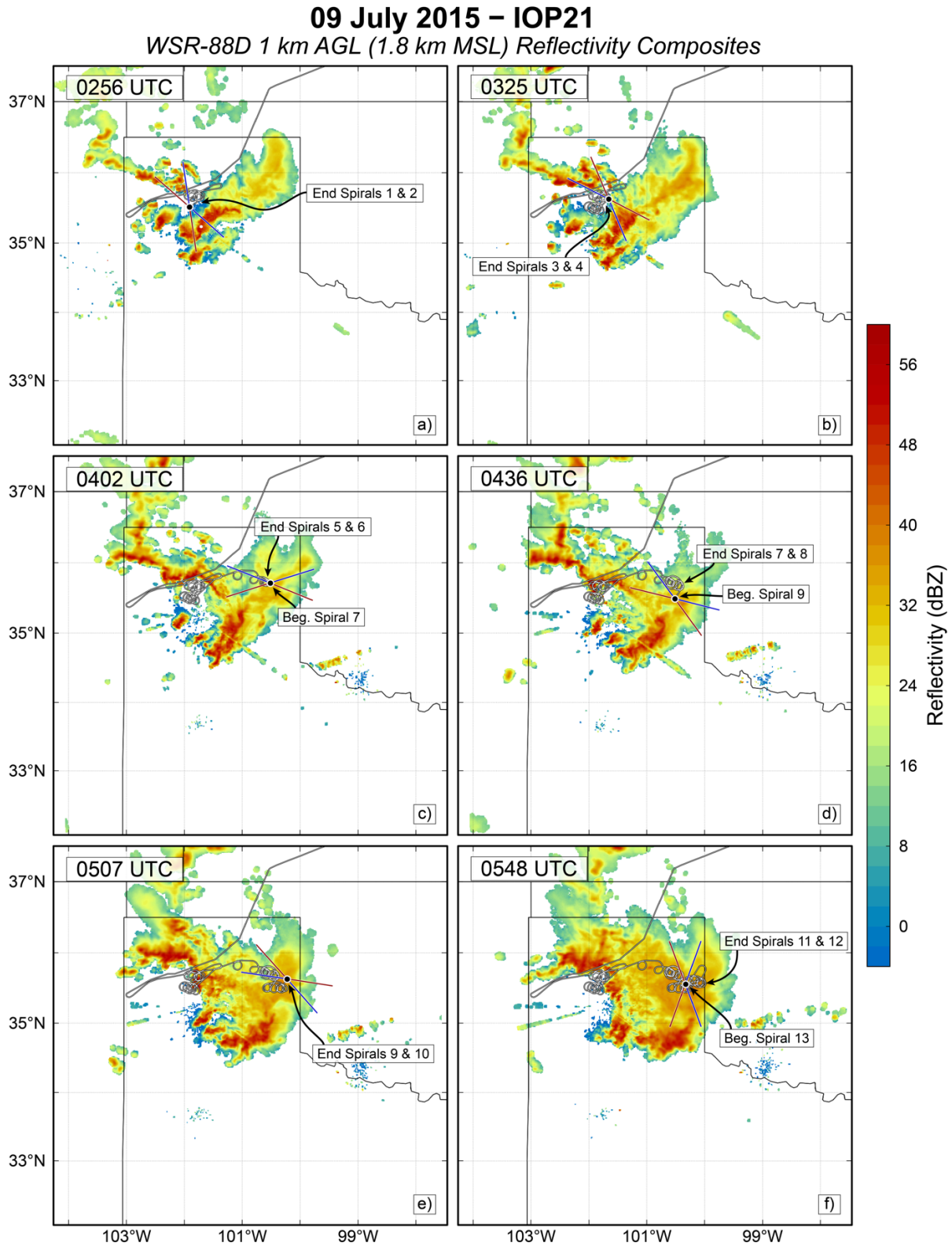
Fig. A4: As in Fig. A1, though for the 9 July 2015 IOP21 MCS. Key periods discussed in the text are shown between 0256 and 0645 UTC.
