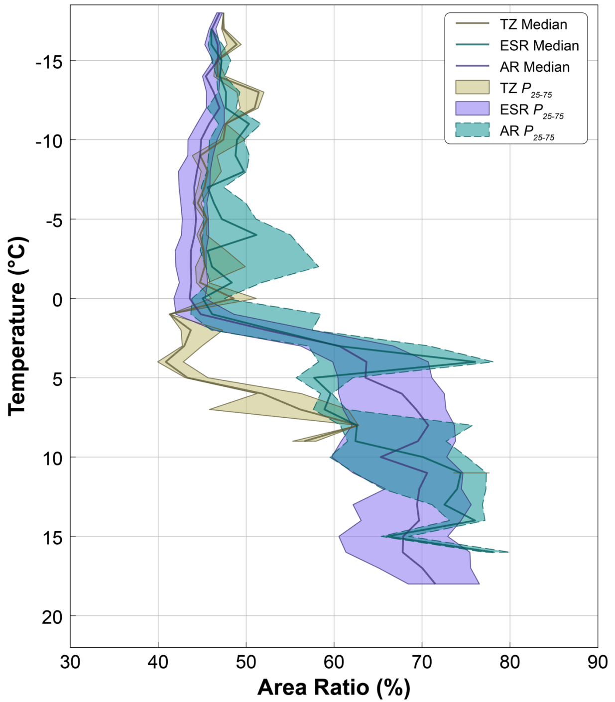
978 Fig. 6: As in Fig. 2, but with vertical profiles of \mathcal{A} (%).
