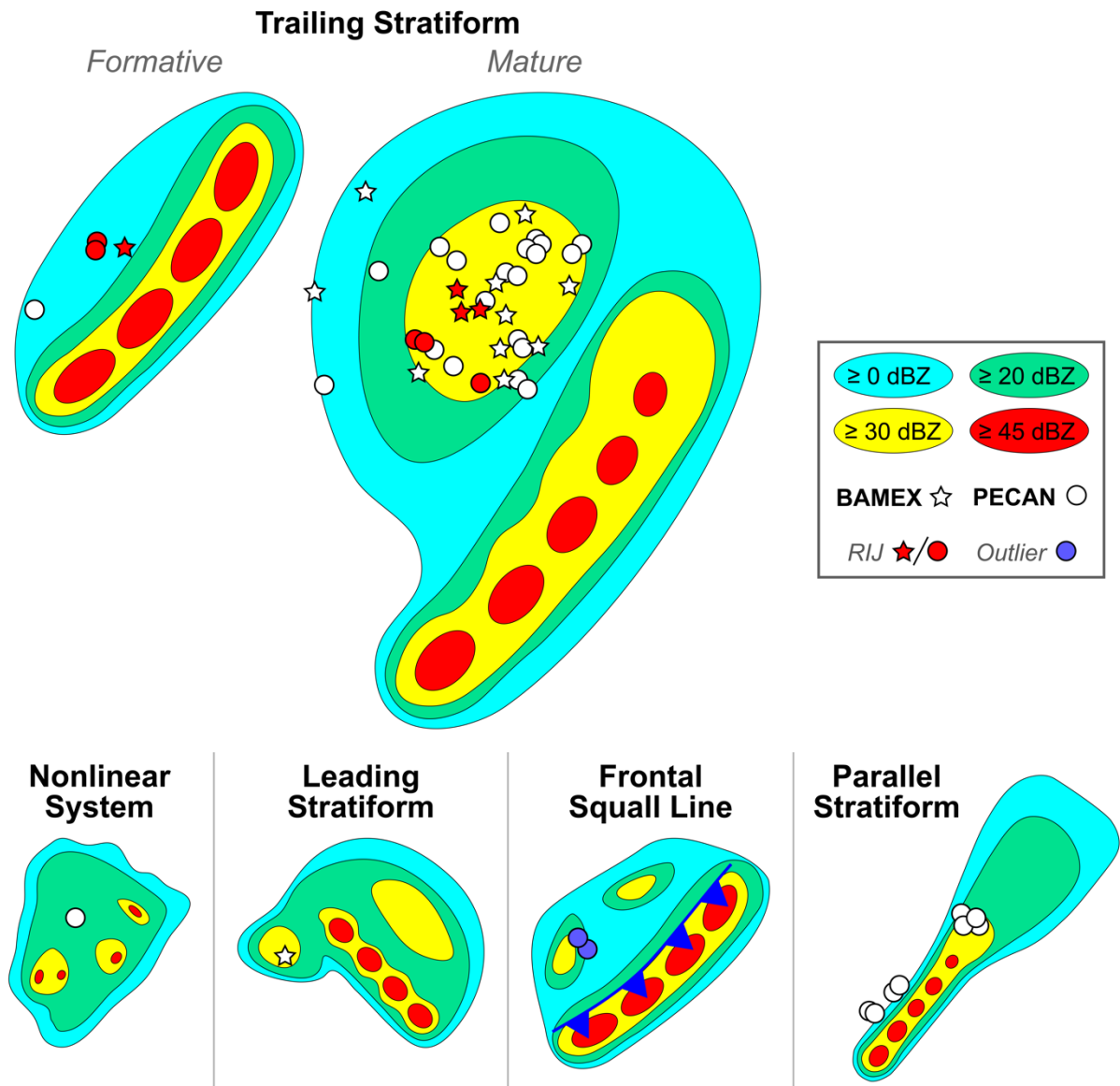
967 Fig. 1: Idealized representation of MCS structures (partially adapted from Parker and Johnson 968 (2000) and Gallus et al. (2008)). Symbols indicate the general locations of spiral profiles executed 969 during BAMEX and PECAN. Red symbols indicate the given spiral occurred within or near the 970 axis of the RIJ, while blue symbols represent outlier spirals excluded from primary MCS zone 971 analysis.
