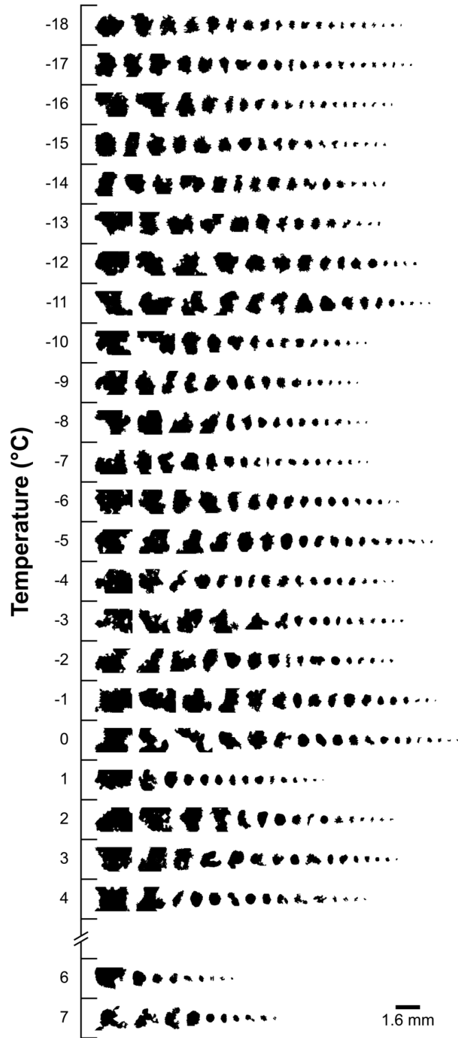
985 Fig. 8: Representative particle images observed by the CIP as a function of T (°C) within spiral 2 986 of the 20 June 2015 PECAN MCS.
