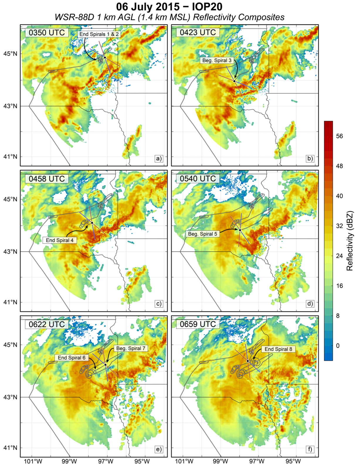
Fig. A3: As in Fig. A1, though for the 6 July 2015 IOP20 MCS. Key periods discussed in the text are shown between 0350 and 0659 UTC.
