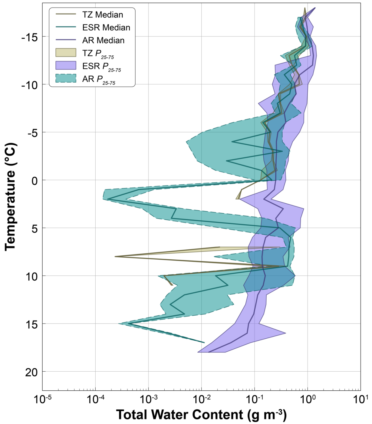
976 Fig. 4: As in Fig. 2, but with vertical profiles of TWC ( \text{g m}^{-3} ).
