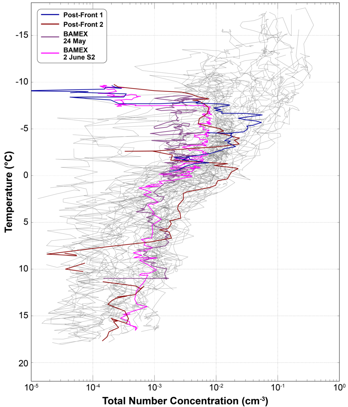
1002 Fig. 16: Vertical profiles of N_t ( \text{cm}^{-3} ) as a function of T ( ^{\circ}\text{C} ) from the two PECAN post-frontal 1003 spirals (dark blue and dark red lines), the 24 May 2003 BAMEX spiral (dark purple line), and 1004 spiral 2 from the 2 June 2003 BAMEX MCS (magenta line). Profiles from each of the other 1005 BAMEX and PECAN spirals in the primary analysis set are underlaid for reference (thin dark grey 1006 lines).
