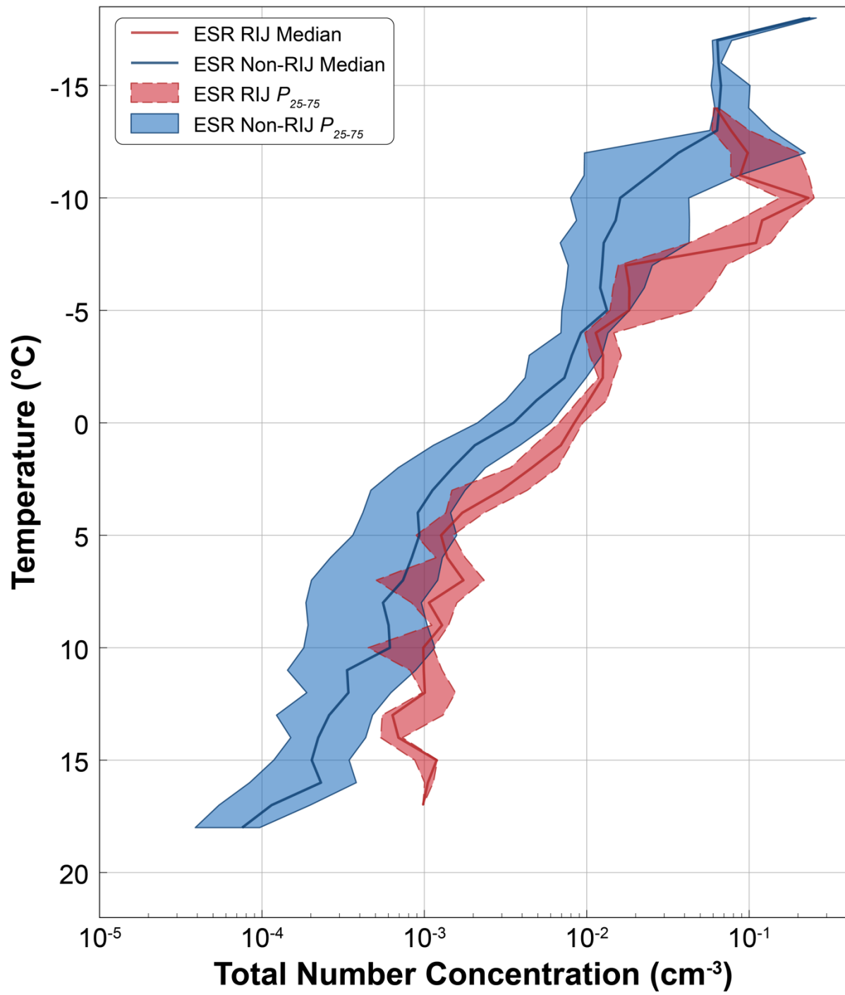
990 Fig. 10: As in Fig. 9, but with vertical profiles of N_t ( \text{cm}^{-3} ).
