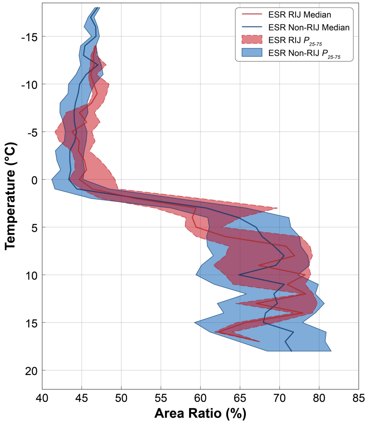
993 Fig. 13: As in Fig. 9, but with vertical profiles of \mathcal{A} (%).
