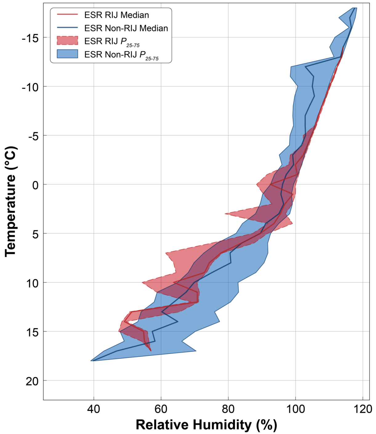
987 Fig. 9: Vertical profiles of \widetilde{RH} (%; red and blue solid lines) and the 25 th -75 th percentile range of 988 RH (%; red and blue filled) for the ESR RIJ and ESR non-RIJ classification sets as a function of 989 T (°C). RH is with respect to ice for T \leq 0^\circ\text{C} , and with respect to liquid water for T > 0^\circ\text{C} .
