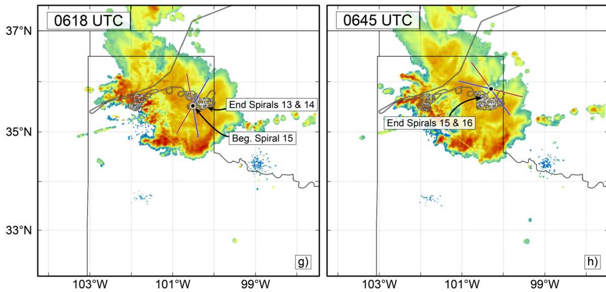
1021 Fig. A4: ( continued )
