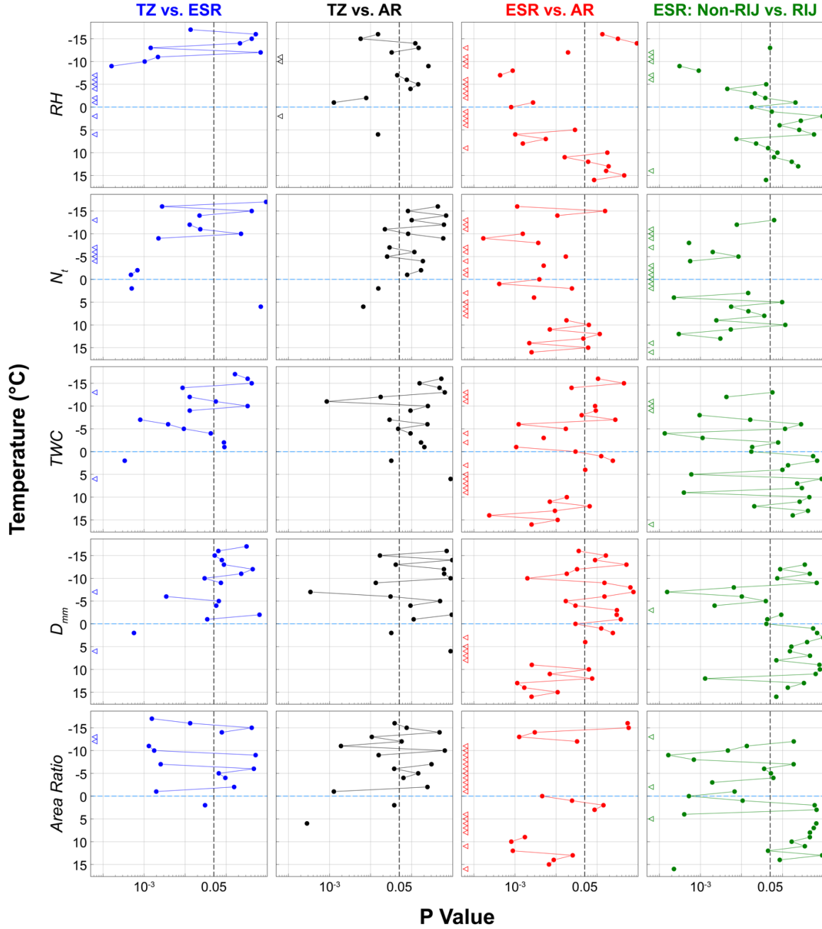
Fig. 14: Results of the K-S test for the TZ vs. ESR (blue traces), TZ vs. AR (black traces), ESR vs. AR (red traces), and the ESR RIJ vs. ESR non-RIJ (green traces). The results of each comparison for RH , N_t , TWC, D_{mm} , and \mathcal{A} are given as a function of T(^{\circ}\text{C}) , where the 0.05 P value is indicated in each panel by a vertical dashed grey line. Triangles indicate P values less than 10^{-4} for a given interval of T . The T = 0^{\circ}\text{C} level is denoted by the horizontal dashed blue line. RH is with respect to ice for T \leq 0^{\circ}\text{C} , and with respect to liquid water for T > 0^{\circ}\text{C} .
