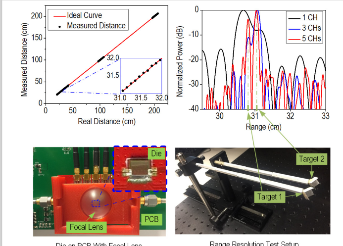
Figure 4.8.5: Measured ranging accuracy and resolution without windowing. Photos of the die on PCB with TPX lens and ranging resolution test setup are also shown.
