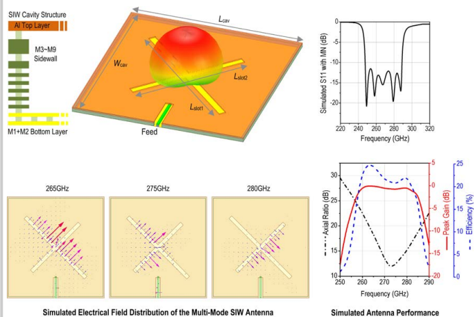
Figure 4.8.3: Structure and simulation of the multimode SIW antenna (CH3).
