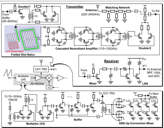
Figure 4.8.2: Schematics of the THz transmitter and receiver of one channel (CH1), as well as the input multiplier, buffer, and SSB upconversion mixer along the frequency-conversion chain.
