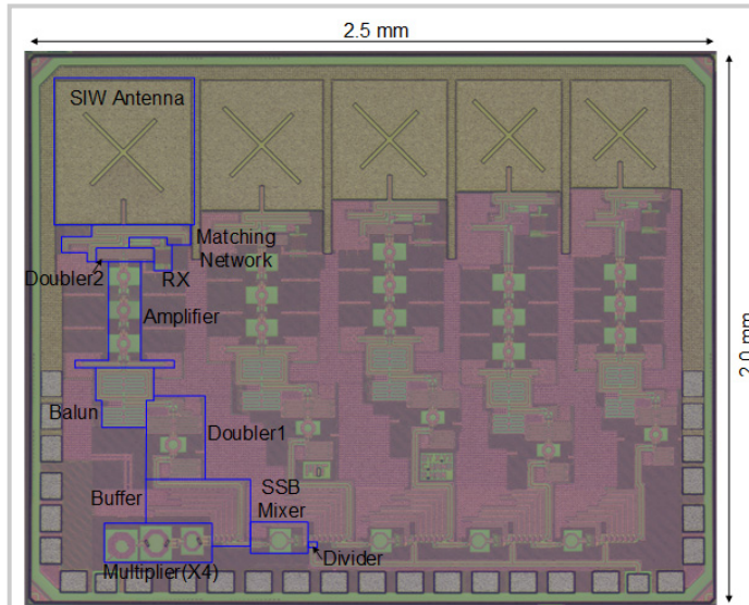
Figure 4.8.7: Die micrograph.
