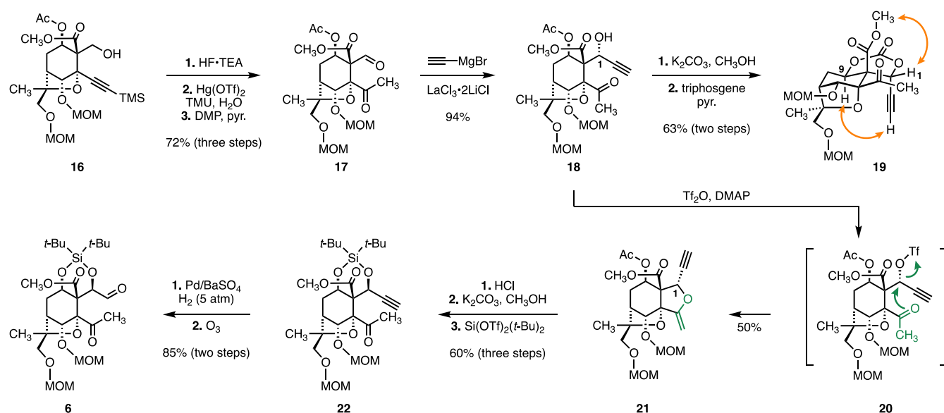
Scheme 3. Synthesis of the Keto Aldehyde 6 ; NOE Enhancements Supporting the Relative Stereochemistry of 19 Are Indicated by Orange Arrows
