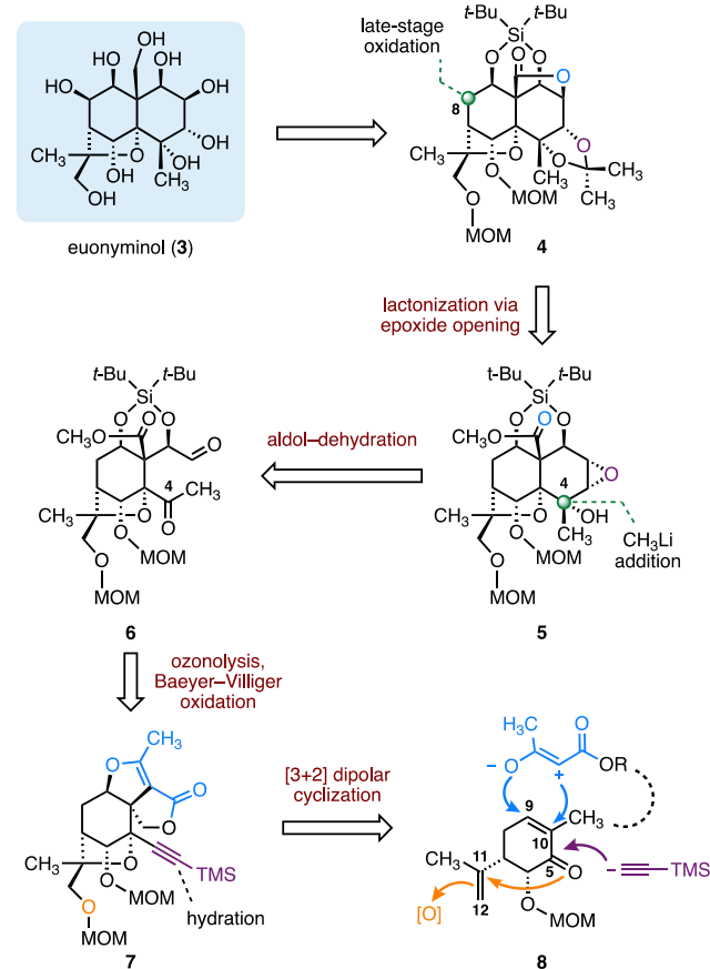
Scheme 1. Retrosynthetic Analysis of Euonyminol (3)
