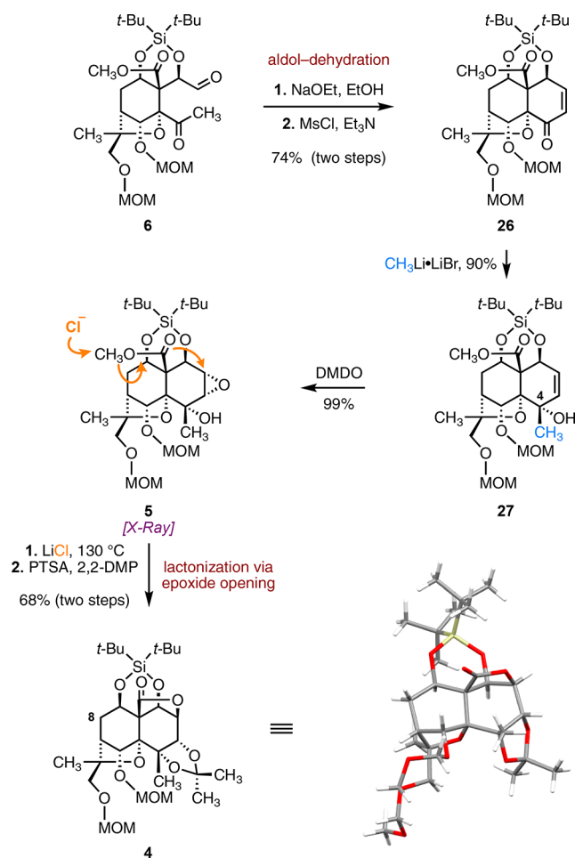
Scheme 4. Synthesis of the Fully Protected Lactone 4
