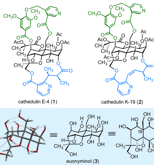
Figure 1. Structures of cathedulin E-4 ( 1 ), cathedulin K-19 ( 2 ), and euonyminol ( 3 ). The cathic acid residues in 1 and 2 are shown in green. The evoninic and eudolinic acid residues found in 1 and 2 , respectively, are shown in blue. The tube representation corresponds to the DFT-optimized structure of 3 . Intramolecular hydrogen bonds are shown with dashed lines.
