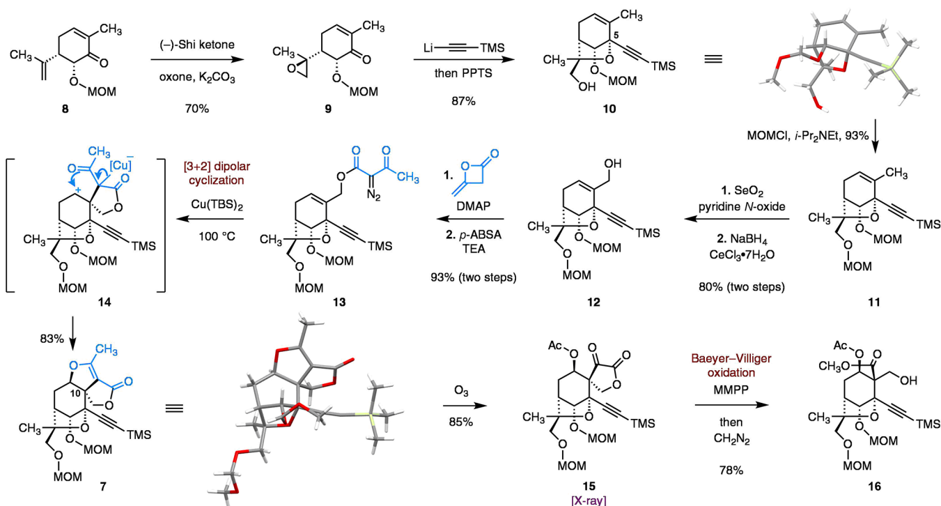
Scheme 2. Synthesis of the Methyl Ester 16 from the Carvone Derivative 8
