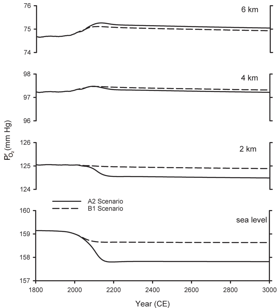
FIGURE 4 | Predicted changes in O 2 partial pressure ( P'_{O_2} ) at different elevations. The curves for sea level are from Shaffer et al. (2009) and repeated from Figure 2 . The curves for other elevations were calculated by accounting both for global O 2 loss and for changes in barometric pressure with warming ( Table 1 ), scaled by the modeled temperature changes from Shaffer et al. (2009).
