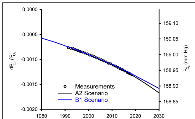
FIGURE 2 | Modeled changes in atmospheric O 2 from Shaffer et al. (2009) versus observed global averages from the Scripps O 2 program (Keeling and Manning, 2014). The O 2 levels are shown on left as fractional change in O 2 partial pressure relative to a preindustrial reference and on right as absolute partial pressure. The observations, originally reported as changes in O 2 /N 2 ratio in per meg units (see Appendix A), were converted to dP'_{O_2}/P'_{O_2} and offset with an additive constant to align with the model results. Global averages are based on the data from Alert (82.5°N), La Jolla (32.9°N), and Cape Grim (40.7°S) stations, following Keeling et al. (1996).
