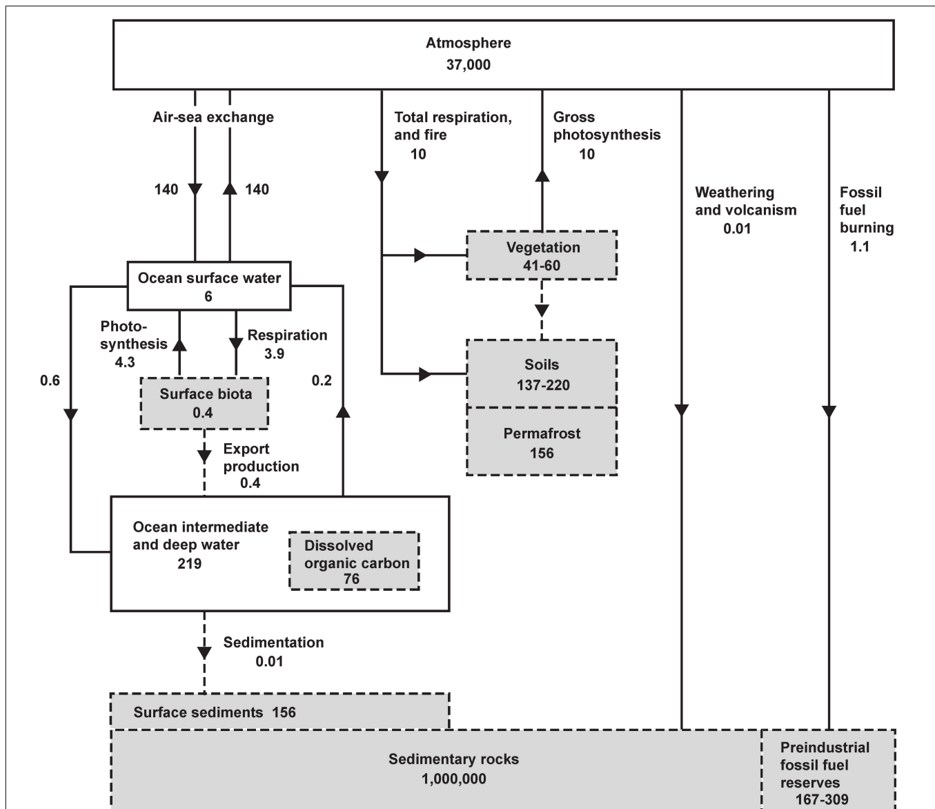
FIGURE 1 | The global oxygen cycle, from Keeling (1988), showing short-term and long-term sources and sinks and coupling with the reservoirs of organic carbon in units of 10^{15} moles and 10^{15} moles year -1 . Oxygen fluxes and reservoirs are denoted by solid lines and solid boxes. Organic fluxes reservoirs are denoted by gray boxes with dashed perimeter, and organic fluxes with dashed lines. Organic matter is expressed in terms of O 2 equivalent, i.e., the amount of O 2 consumed when the material is fully oxidized. Organic reservoirs other than surface biota and sedimentary rocks have been updated using recent estimates from Ciais et al. (2013) using O 2 /C oxidative ratios of 1.1 (vegetation, soils, permafrost), 1.3 (dissolved organic carbon), and for fossil-fuel by fuel type from Keeling (1988). Fluxes and reservoirs other than fossil-fuel burning are notionally for a pre-industrial steady state. Fossil-fuel burning is for year 2019 (Friedlingstein et al., 2020).
