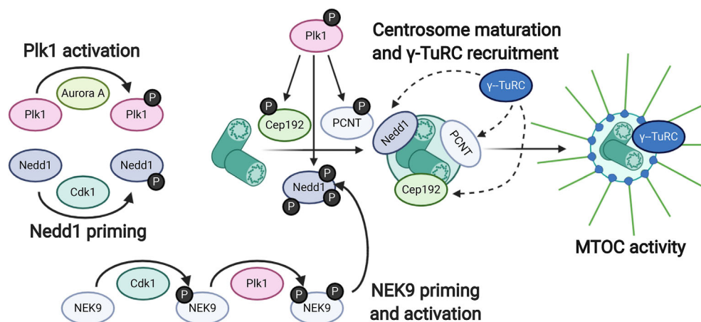
FIGURE 4 Plk1 regulates centrosome maturation and microtubule organizing center (MTOC) activity. Once activated by Aurora A, Plk1 phosphorylates centrosomal proteins like Cep192, PCNT, and Nedd1. Cdk1 primes NEK9 for activation by Plk1, and NEK9 also phosphorylates Nedd1. These and other centrosomal proteins play roles in centrosome maturation, pericentriolar material expansion, and \gamma -TuRC recruitment to the centrosome, allowing the centrosome to serve as a MTOC [Color figure can be viewed at wileyonlinelibrary.com ]
