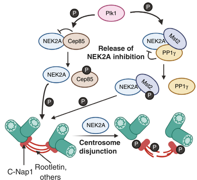
FIGURE 5 Plk1 regulates NEK2A in centrosome disjunction. Plk1 phosphorylates Cep85 to free Cep85 inhibition of NEK2A. Similarly, Plk1 phosphorylates Mst2 to disrupt the PP1 \gamma from antagonizing the activity of NEK2A. Once activated, NEK2A phosphorylates a number of linker proteins at the centrosomes, including C-Nap1 and Rootletin, to free the two centrosomes from each other [Color figure can be viewed at wileyonlinelibrary.com ]
