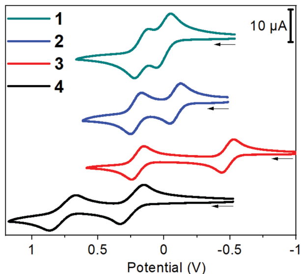
Fig. 3 Cyclic voltammograms of 1–4 (ca. 0.001 M in \text{CH}_2\text{Cl}_2 ) with [\text{tBu}_4\text{N}]\text{PF}_6 electrolyte (0.1 M), scan rate 100 \text{ mV s}^{-1} , potentials referenced to \text{Fc}^+/\text{Fc} at 0 V.
