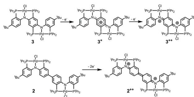
Fig. 5 Dominant resonance forms upon oxidation of 2 and 3 .
