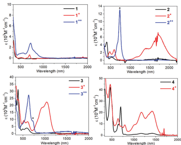
Fig. 8 UV-Vis-NIR spectra of compounds 1–4 and their oxidized derivatives. The monocations were produced in situ via addition of 1 equiv. of oxidant ([Ox] = [(BrC 6 H 4 ) 3 N]SbCl 6 ) solutions of 1–4 in CH 2 Cl 2 and the dications were produced via addition of 2.2 equiv. of oxidant. The asterisk labels the possible overlapping at 732 nm of excess [(BrC 6 H 4 ) 3 N]SbCl 6 .
