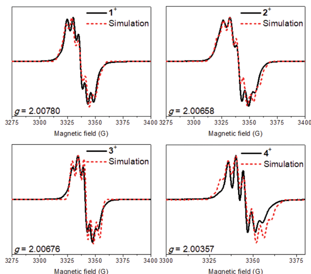
Fig. 6 X-band EPR spectra (in black) of monocations 1–4 (ca. 0.01 M in \text{CH}_2\text{Cl}_2 ) generated in situ by treating 1–4 with 0.9 equiv. of [(p\text{-BrC}_6\text{H}_4)_3\text{N}]\text{SbCl}_6 . Instrumental parameters: T = 292\text{ K} ; freq = 9.38 GHz; power = 0.6 mW, modulation 1 G. Simulations are shown in red (EasySpin).
