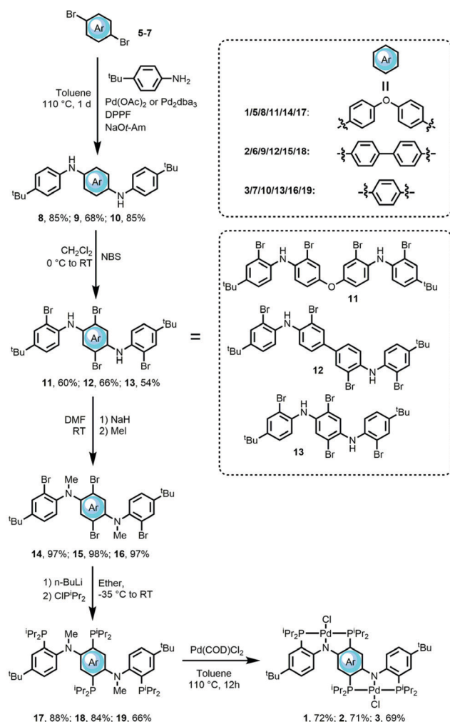
Scheme 1 Synthesis of bis(PNP) pro-ligands and their Pd complexes 1–3.
