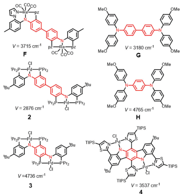
Fig. 10 Hush coupling constants comparison.
