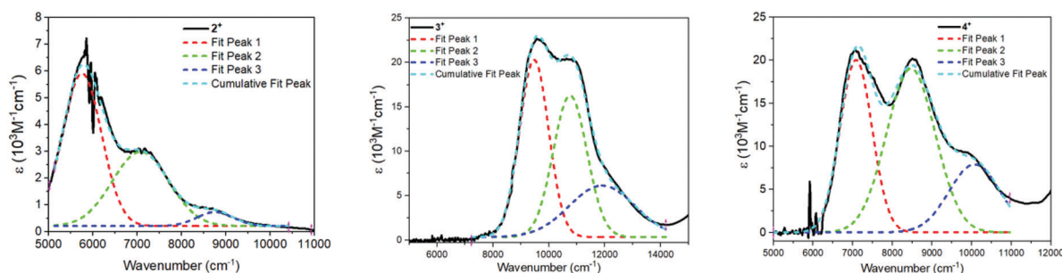
Fig. 9 Deconvolution of low energy bands of 2 + –4 + .
