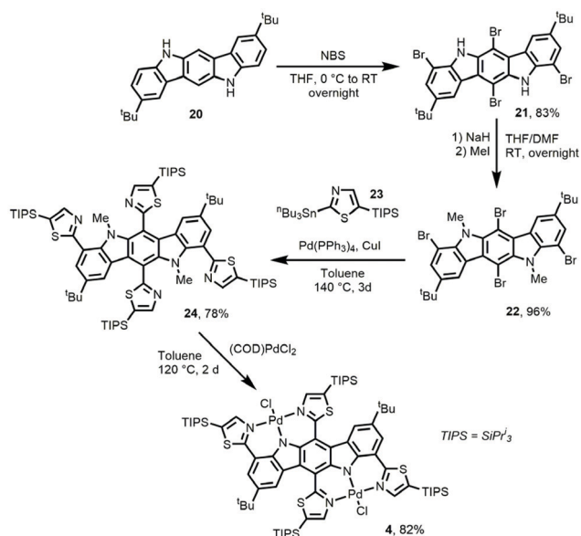
Scheme 2 Synthesis of Pd complex 4.
