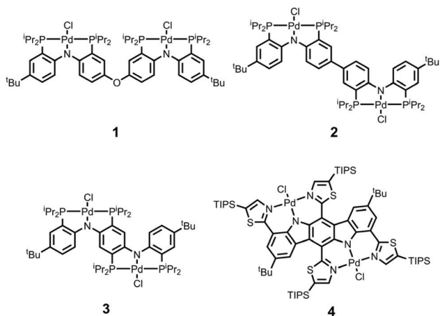
Fig. 2 Bis(pincer) complexes synthesized and studied in this work.
