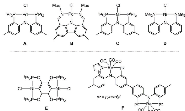
Fig. 1 Top: selected examples of diarylamido-centered pincer complexes, whose reversible redox properties have been studied previously. Bottom: recent examples of Janus pincers in the literature.
