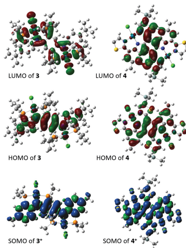
Fig. 7 Depictions of the calculated LUMO, HOMO and SOMO for 3/3^+ (left) and 4/4^+ (right) (isovalue = 0.02). The silyl groups on the outer thiazole rings of 4/4^+ have been removed from the graphic for clarity.
