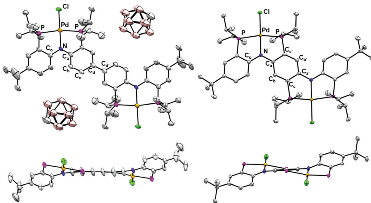
Fig. 4 ORTEP drawings depicting the structure of [2][\text{CB}_{11}\text{H}_{12}]_2 and 3. Displacement ellipsoids are shown at the 50% probability level and all hydrogen atoms have been removed for clarity.
