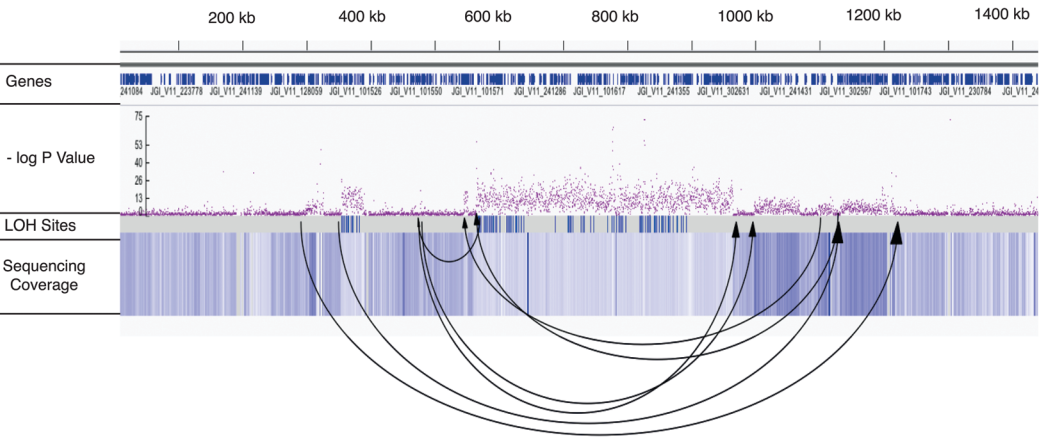
Figure 5. Complex mutation event leading to multiple duplications and deletions in the MA subline CYC-17. Arrows denote the left and right Illumina read pairs (with arrows not signifying left or right, specifically) and provide evidence for complex de novo events on scaffold 18 in CYC-17, including a large-scale deletion ( center of figure) and multiple smaller duplications and deletions. While distance between read pairs should only be a few hundred base pairs, the arrows show read pairs with drastic differences in mapping distance and are indicative of indel activity. The sequence coverage track represents the normalized depth of sequencing coverage, relative to the other CYC MA sublines, where lighter color represents lower relative coverage (e.g., the 401-kb deletion). Also, -\log P is plotted for each consecutive sliding window (i.e., the probability of a region deviating from 1:1 coverage ratios by chance, or the probability of an indel), and higher values relative to lower values represent increasing probability of CNV (see Methods).
