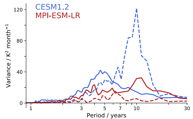
FIGURE 4 Power spectra of monthly-mean Nino 3.4 SST variability in simulations with either interactive clouds (solid) or locked clouds (dashed) in the CESM1.2 (blue: Middelmas, Clement, Medeiros, & Kirtman, 2019) and the MPI-ESM-LR models (red; Rädel et al., 2016). The spectra were calculated from 100-year chunks using Welch's method as implemented in Python's scipy version 1.3.1
