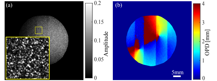
Fig. 13. Failure case with WISHED: Imaging the glass stack with a diffuser as shown in Fig. 7 with speckles averaged on the sensor plane. (a) Amplitude with speckles averaged on the sensor plane. (b) Reconstructed depth profile with the same synthetic wavelength using the proposed method.
