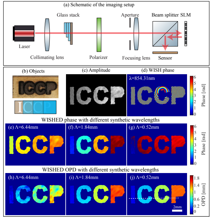
Fig. 5. Experiment on optical smooth objects in transmissive mode. (a) Setup illustration. (b) The object: a letter mask with a glass stack in front. (c) Amplitude measurement. (d) WISH reconstruction: phase maps with one optical wavelength. (e-g) WISHED reconstruction: phase maps with different synthetic wavelengths. (h-j) OPD with different synthetic wavelengths. Smaller synthetic wavelength provides higher depth precision.
