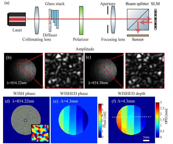
Fig. 7. Experiment on optical rough objects in transmissive mode. (a) Setup illustration. (b,c) Amplitude measurement (no SLM modulation) with two close wavelengths 854.22nm (b) and 854.38nm (c). These two speckle patterns are similar since their wavelengths are close. (d) phase map from WISH reconstruction. The 3D information is totally lost due to the speckle pattern. (e) phase map from WISHED reconstruction. The synthetic wavelength is 4.3mm. (f) Estimated OPD, where glass layers are clearly visualized.
