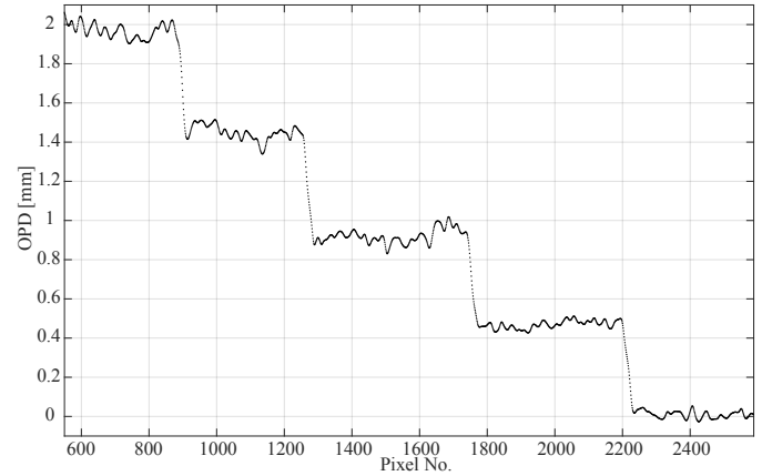
Fig. 8. OPD profile along one line on the plate stack as shown in Fig. 7(f). The x-axis marks the different points along the line, and y axis is the OPD value. Note: each glass plate introduces an OPD of 0.5mm. The RMSE in optical depth for the measurement is 69 \mu m.
