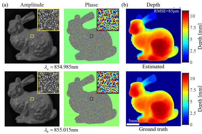
Fig. 4. Simulation reconstruction. (a) Recovered object fields for two wavelengths. (b) Comparison between ground truth and WISHED estimated depth using a synthetic wavelength of 24.4mm (RMSE = 85μm).
