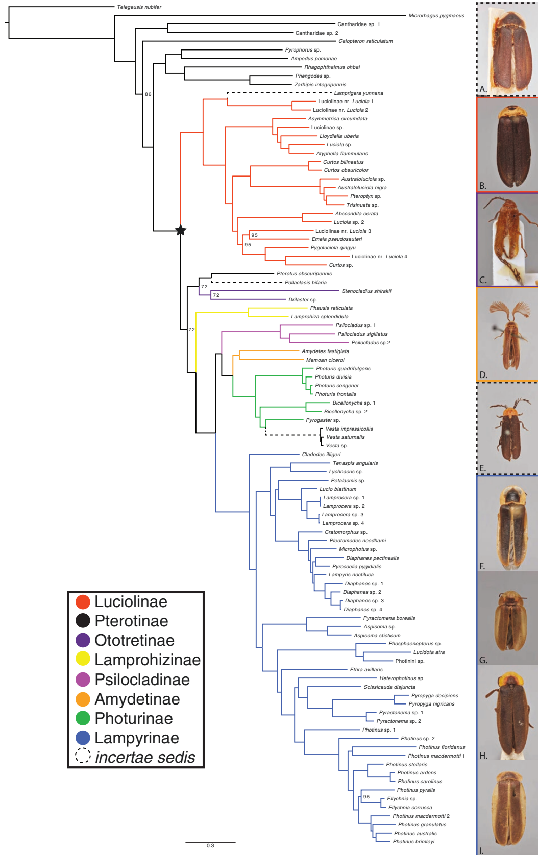
Fig. 1. ML reconstruction of full, untrimmed dataset aligned in MAFFT; log-likelihood = -26,321,164.240. The numbers at nodes indicate UFBoot support. Unlabeled nodes have UFBoot values of 100%, colors represent the newly proposed classification. Star at node depicts Lampyridae; A.-I. Dorsal habitus of genus representatives: A. Lamprigera yunnana ; B. Luciola cyathigera ; C. Stenocladus davidi ; D. Amydetes fastigiata ; E. Vesta chevrolati ; F. Diaphanes sp.; G. Aspisoma gentile ; H. Ellychnia aurora ; I. Photinus laticollis ;
