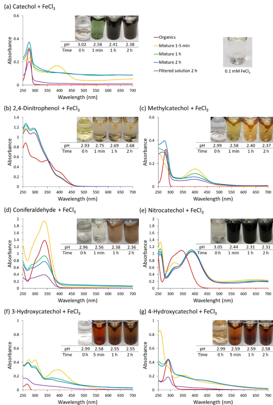
Figure 1: UV-Vis absorption spectra of mixtures of Fe(III) with (a) pyrocatechol, (b) 2,4-dinitrophenol, (c) 4-methylcatechol, (d) coniferaldehyde, (e) 4-nitrocatechol, (f) 3-hydroxycatechol, and (g) 4-hydroxycatechol. Different colors of traces correspond to spectra of organic reactant before mixing (red), 1-5 min after mixing (orange), 1 h after mixing (green), 2 h after mixing (blue), and filtered solution (purple). The final concentration of organics is 1mM, and the final concentration of Fe(III) is 2 mM. The photographs are those of unfiltered solutions.
