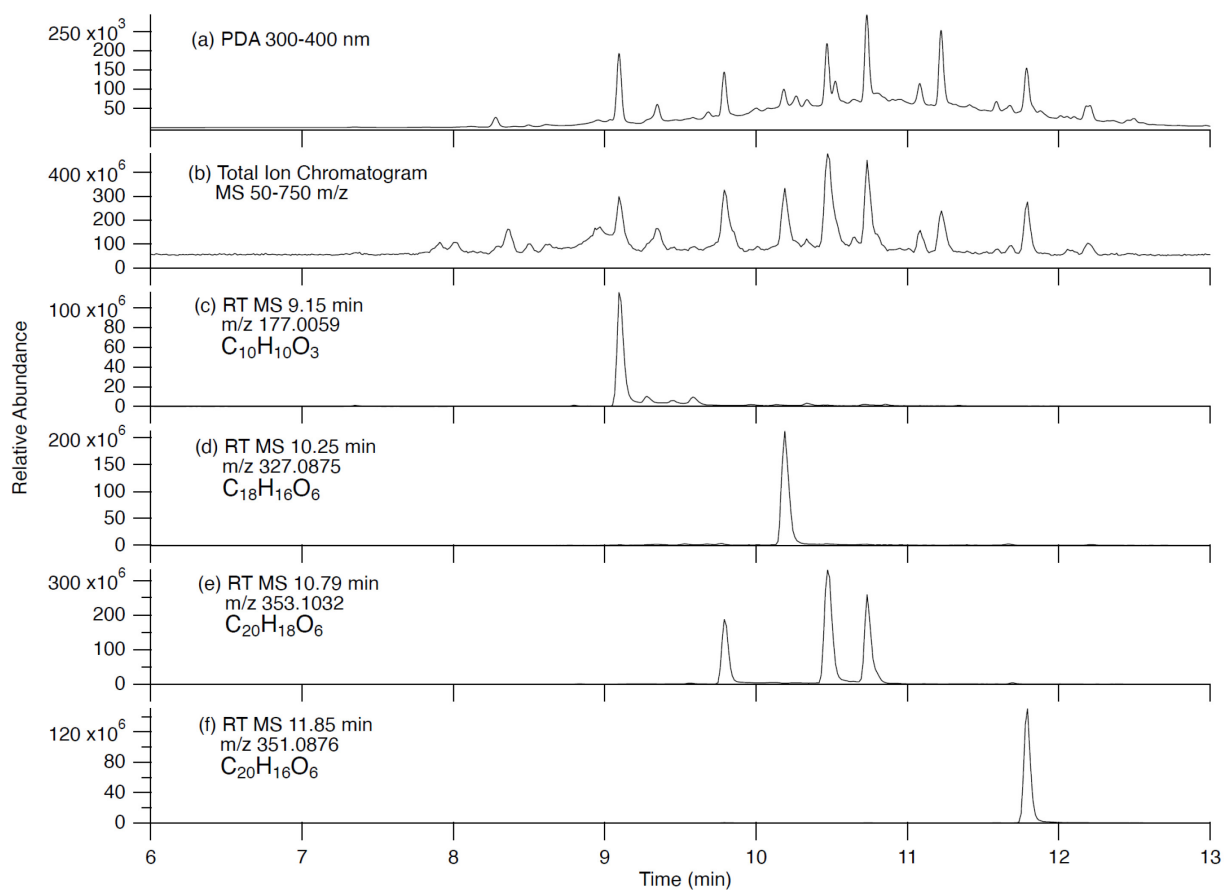
Figure 4: UPLC-PDA-HRMS data for the CON + Fe(III) reaction products: (a) photodiode array (PDA) chromatogram; (b) total ion current (TIC) chromatogram; and (c & d) single ion monitoring (SIM) chromatograms. The TIC and SIM chromatograms were corrected for the 0.06 min delay time between PDA and Orbitrap detectors. The formulas listed correspond to neutral compounds observed as deprotonated ions at the specified m/z values.
