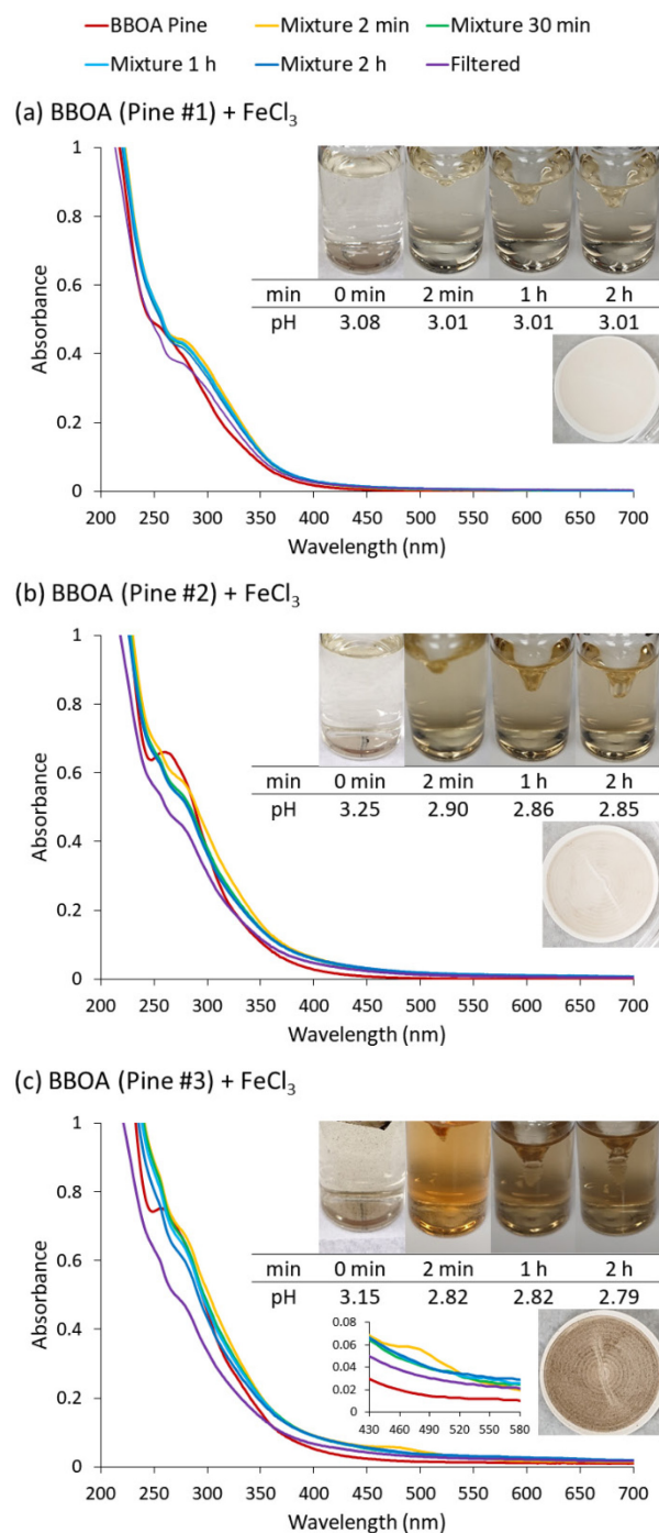
Figure 5: UV-Vis absorption spectra of mixture of excess \text{Fe(III)} and BBOA extracts. Different colors of traces correspond to spectra of BBOA before mixing (red), 2 min after mixing (orange), 30 min after mixing (green), 1 h after mixing (light blue), 2 h after mixing (dark blue), and filtered solution (purple).
