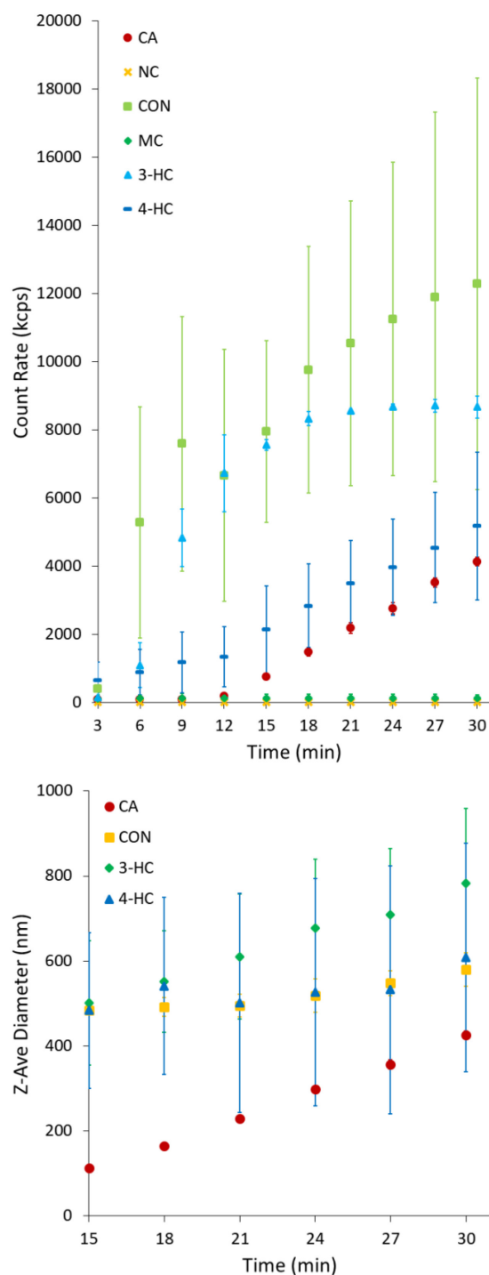
Figure 3: DLS measurements of the derived count rate of each iron-organic solution mixture as a function of reaction time during the dark condition of the organics including pyrocatechol (red), 4-nitrocatechol (orange), coniferaldehyde (green), 4-methylcatechol (dark green), 3-hydroxycatechol (blue), and 4-hydroxycatechol (dark blue). Error bars represent a standard deviation from two repeat measurements.
