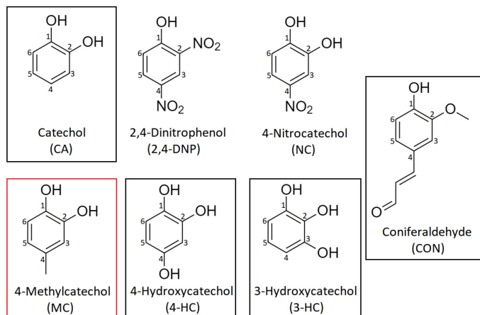
Scheme 1: Chemical structures and abbreviation codes of pyrocatechol (CA), 2,4-dinitrophenol (2,4-DNP), 4-nitrocatechol (NC), coniferaldehyde (CON), 4-methylcatechol (MC), 4-hydroxycatechol (4-HC), and 3-hydroxycatechol (3-HC). The frames in black highlight the organic compounds that produced particles promptly due to reaction with Fe(III); MC is surrounded by a red frame because it produced particles on a slower time scale.
