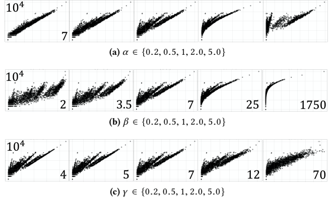
Figure 11: PfV plots for Columbus Bike varying each exponent in \{0.2, 0.5, 1, 2.0, 5.0\} , while fixing the other two at 1. The main takeaways are that small values of \beta (0.2 or 0.5) increase the spread of points, while increasing \gamma (2.0 or 5.0) emphasizes points in the lower left (i.e., very regular snippets). Thus, it is generally effective to set \alpha = 1 , \beta \in (0, 1) , and \gamma \in (1, \infty) .
