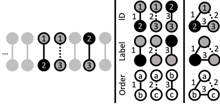
Figure 3: Left: An update sequence that is ordered but not contiguous. Right: The activity snippet for the sequence, depending on the view \phi (ID, LABEL, or ORDER), and a graph describing the activity. Solid/dashed edges capture types of interactions (e.g., edge types or insertions vs. deletions), and the node colors denote labels.
