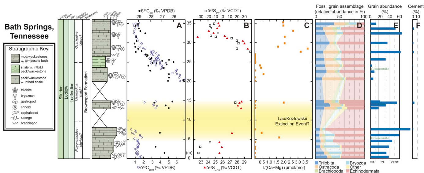
Fig. 6. Composite stratigraphic column for the Bath Springs roadcuts with geochemical and microfossils data. A) Carbonate and organic carbon isotope data. B) Carbonate-associated sulfate and pyrite sulfur isotope data. C) I/(Ca + Mg) ratio data. D) Relative abundances of fossil grains. E) Grain abundance with presence of glauconite noted and the approximate divisions for different Dunham (1962) carbonate textures marked. F) Percentage of cement.
