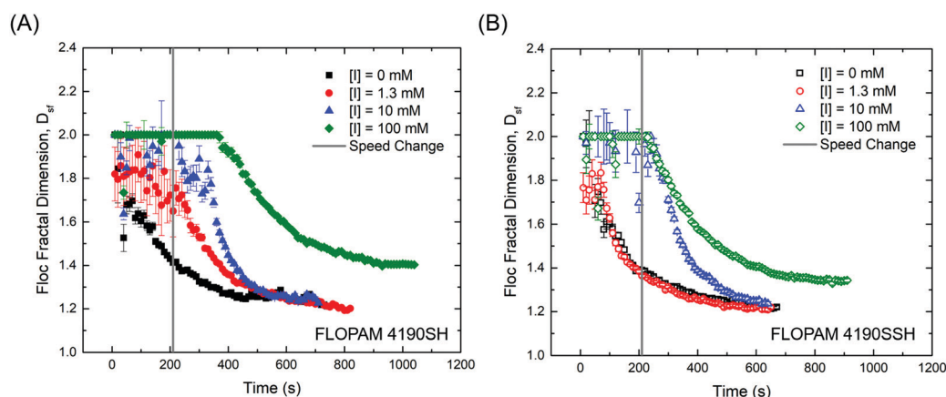
Fig. 5 Floc morphology quantified as a 2-D perimeter-based fractal dimension, D_{sf} , as a function of ionic strength with time for the (A) lower molecular weight cationic polyacrylamide flocculant (4190SH) and the (B) higher molecular weight cationic polyacrylamide flocculant (4190SSH). The vertical, gray line depicts where the inner cylinder speed transitions from \Omega_i = 0.50 s -1 to \Omega_i = 0.46 s -1 .
