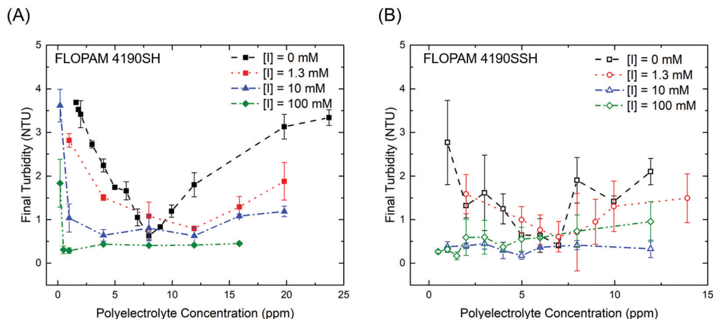
Fig. 1 Jar test results as a function of solution ionic strength using the (A) lower molecular weight cationic polyacrylamide flocculant (4190SH) and the (B) higher molecular weight cationic polyacrylamide flocculant (4190SSH). The final turbidity in terms of nephelometric turbidity units (NTU) is expressed as a function of the polyelectrolyte dose, or concentration, in parts per million (ppm). The global minimum in each curve denotes the optimal dose for a set of solution conditions. Error bars represent one standard deviation from the mean turbidity.
