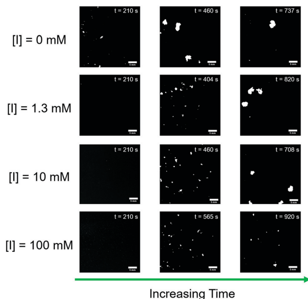
Fig. 2 Time lapse of binarized images of bentonite–cationic polyacrylamide flocs (here, the 4190SH flocculant was used) as a function of ionic strength. The first image in each row is at 210 s, which is the onset of the inner cylinder speed change from Stage 1 to Stage 2 mixing. The last image in each row occurs where the floc size plateaus. The middle image in each row occurs at the midpoint time between the times associated with the first and last images. The white scale bar in the lower right-hand corner of each image represents 5 mm. The movie frames have been resized to comply with figure dimension limitations. The actual movie frames used in the quantitative analysis are larger than what is shown here (actual dimensions of each frame are 1280 × 1024 pixels).
