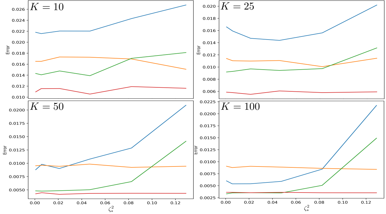
Figure 1: Binary logistic regression between even vs odd digits of MNIST. Twenty-five “tasks” were constructed, one for each combination of i vs j for even i and odd j . For p \in \{0, 20, 40, 60, 80, 100\} , we assigned to each of M = 25 machines p\% data from task m , and (100 - p)\% data from a mixture of all tasks. For several choices of R and K , we plot the error (averaged over four runs) versus the value of \zeta_*^2 resulting from each choice of p . For both algorithms, we used the best fixed stepsize for each choice of K , R , and \zeta_* individually. Additional details are provided in Appendix D.
