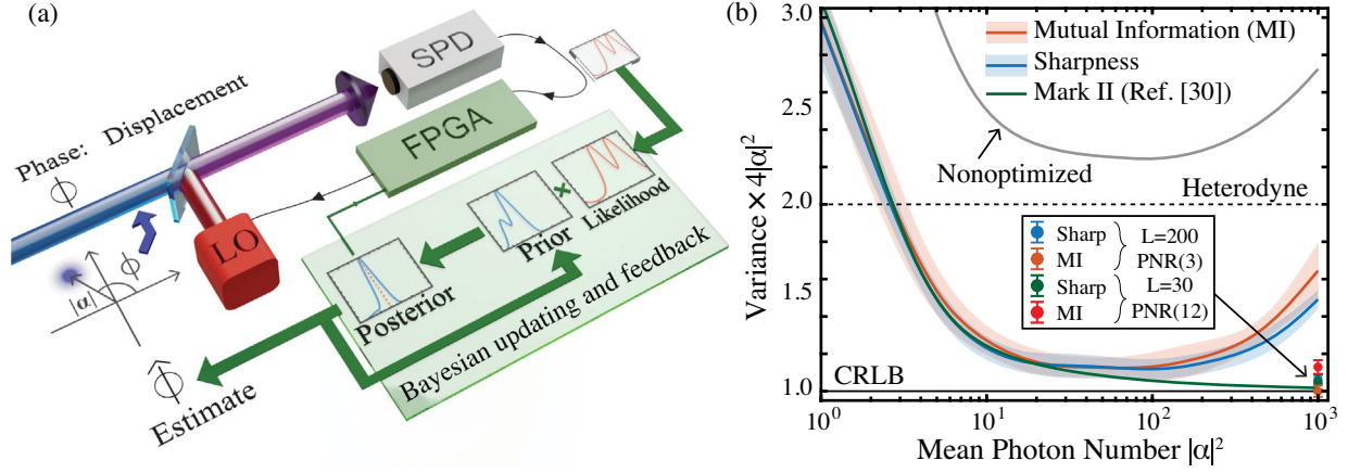
FIG. 1. Optimized non-Gaussian estimation strategy. (a) Concept of the adaptive displaced photon counting measurement for single-shot phase estimation. (b) Simulated Holevo variance multiplied by the quantum Fisher information for coherent states ( 4|\alpha|^2 ). Shown are strategies maximizing the sharpness \langle S(\beta, m) \rangle (blue) and the mutual information I(\beta, m) (orange), and a nonoptimized strategy (gray), all with L = 30 adaptive steps, PNR(3), and ideal efficiency. Also shown is the CRLB for coherent states ( 1/4|\alpha|^2 ), the lower bound of a heterodyne measurement ( 1/2|\alpha|^2 ), and the performance of the adaptive homodyne scheme termed “Mark II” from Ref. [30]. Bold lines are the average of five Monte-Carlo simulations of 10^3 randomly distributed initial phases, and the shaded regions represent one standard deviation. The performance of both estimation strategies at |\alpha|^2 = 10^3 for PNR(3) with L = 200 and for PNR(12) with L = 30 are shown for reference.
