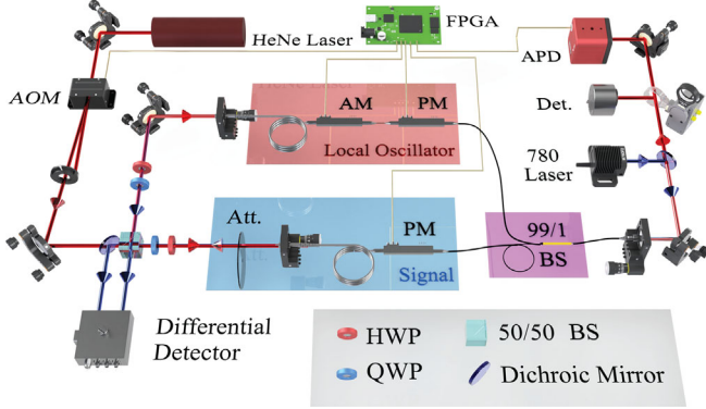
FIG. 2. Experimental setup for the adaptive displaced photon counting measurement (see text for details). HeNe: helium-neon laser, AOM: acousto-optic modulator, Att.: attenuator, PM: phase modulator, AM: amplitude modulator, BS: beam splitter, APD: avalanche photodiode; FPGA: field-programmable gate array.
