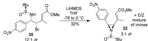
Scheme 8. Vinyl Aziridine Cyclization Studies
