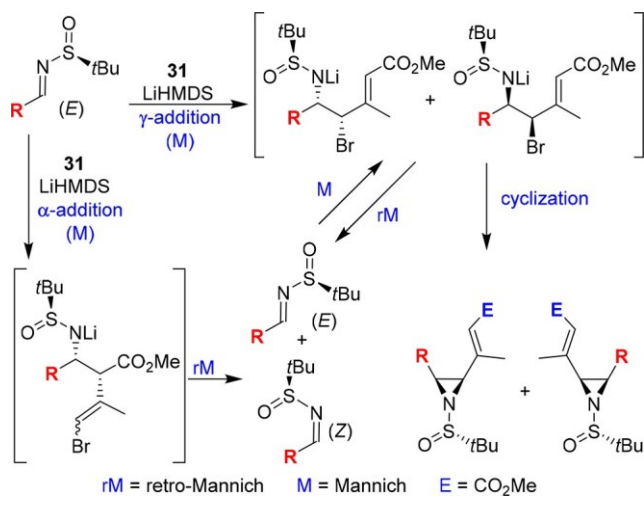
Scheme 9. Mechanistic Proposal
