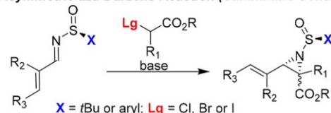
Scheme 1. Vinylogous Asymmetric Aza-Darzens Proposal
