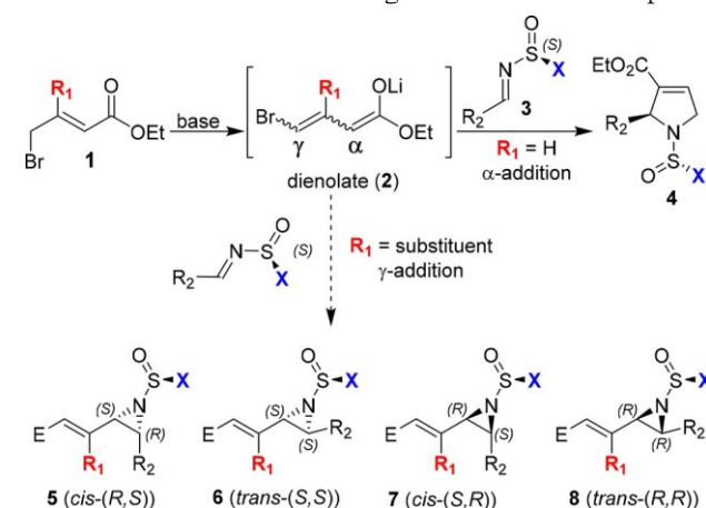
Scheme 2. Mechanistic Challenges: Choice of Nucleophile
