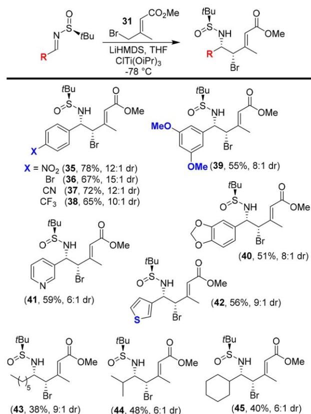
Scheme 7. Titanium Enolate-Mediated Mannich Reactions a
