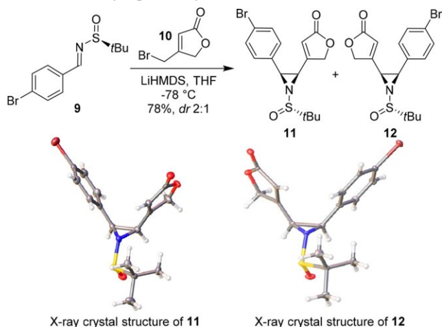
Scheme 3. Vinylogous Asymmetric Aza-Darzens Reaction
