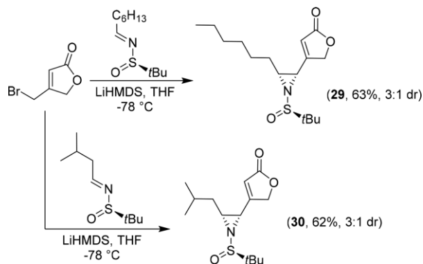
Scheme 6. Altering Nucleophile Impacts Reaction Yields
