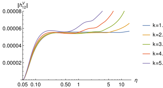
FIG. 9. Time evolution of the vector mode h_{12}^V excited by the tensor mode at different k , with the same initial condition as in Fig. 5.
