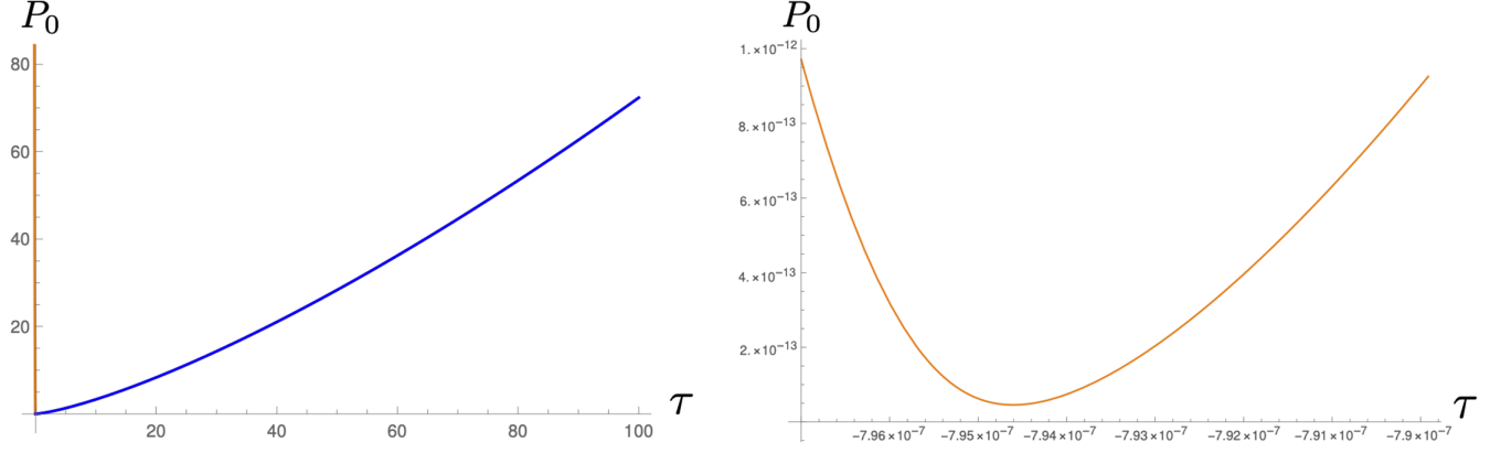
FIG. 1. The left panel plots of P_0(\tau) solving Eqs. (4.2) and (4.3) (orange curve) and P_0(\tau) solving Friedmann equations (blue curve). Two solutions approximately coincide in \tau > 0 except for regime near the big-bang singularity. The solution of Eqs. (4.2) and (4.3) replaces the singularity by a bounce. The right panel enlarges the regime near where the bounce happens. The solutions use initial conditions P_0(1) = 0.153262 , K_0(1) = 0.260992 . Values of other parameters are \Lambda = 10^{-5} , \beta = 1 , \kappa = 1 , and \mu = 10^{-3} . The final time is T = 100 .
