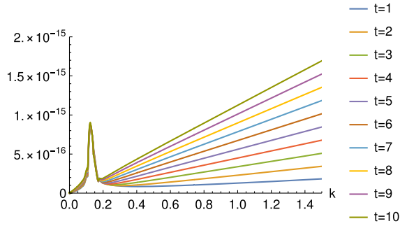
FIG. 4. This figure plots the error of closure condition |G|^2 = \sum_{i=1}^3 G_i^2 where G_i are given by Eqs. (4.15). |G|^2 at different \tau are illustrated by different colors. |G|^2 is much smaller than \mu^4 = 10^{-12} in the plotted range of k .
