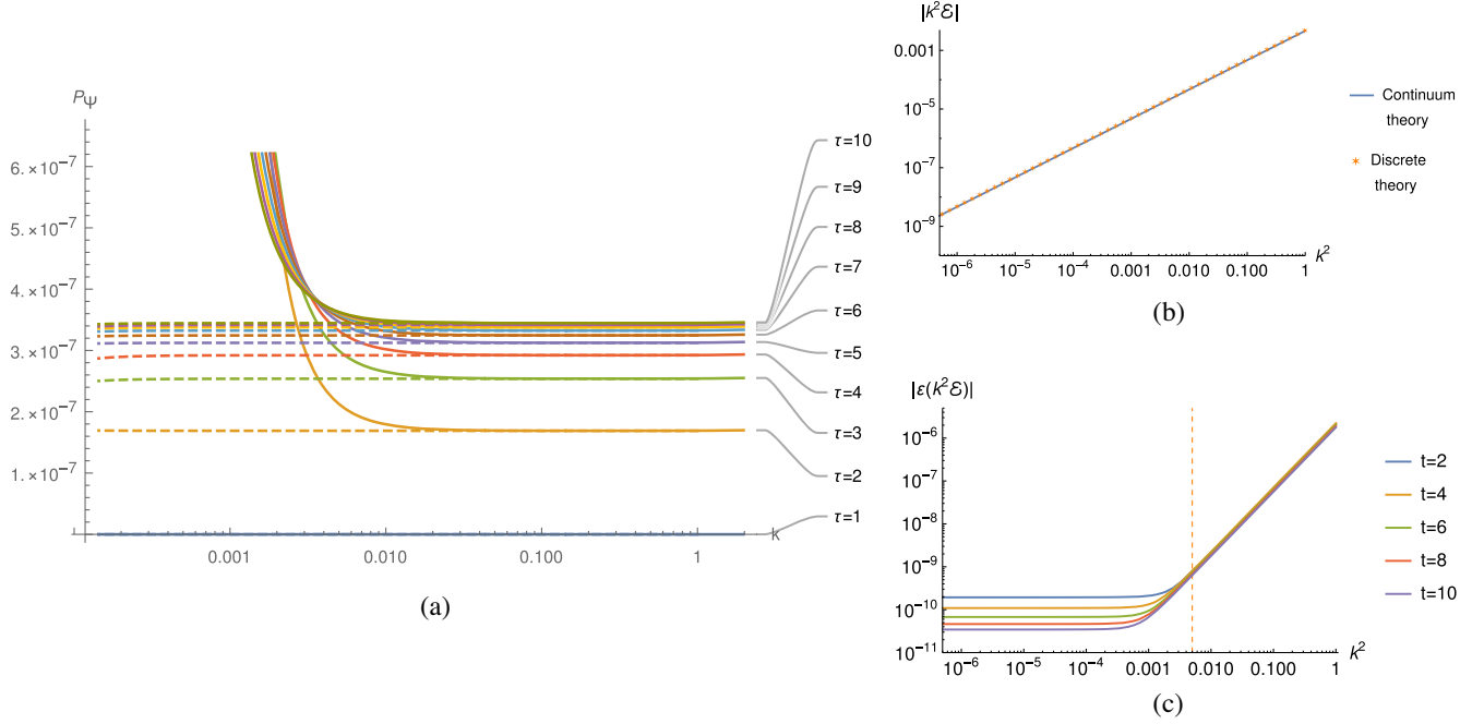
FIG. 2. (a) Comparing the scalar mode power spectrum P_\Psi of Bardeen potential between the classical continuum theory and the discrete theory from LQG. Dashed lines are P_\Psi from the classical continuum theory, while solid curves are from the discrete theory. Different colors illustrate P_\Psi (as functions of k ) at different time \tau . (b) Plots of |k^2 \mathcal{E}| = |(h_{11}^S - h_{22}^S)/2| versus k^2 at \tau = 10 . In the continuum limit \mathcal{E} does not depend on k . (c) Plots of |\epsilon(k^2 \mathcal{E})| where \epsilon(k^2 \mathcal{E}) = k^2(\mathcal{E} - \mathcal{E}|_{\mu \rightarrow 0}) are differences between solutions of discrete EOMs and classical continuum theory. Orange dashed line separates approximately the k dominant region and the background dominant region. Initial condition of those plots are imposed at \tau_i = 1 . Initial values of \psi, \dot{\psi}, \mathcal{E}, \dot{\mathcal{E}} are given by Eqs. (5.15)–(5.17) with C_2 = 0.001 , \epsilon_0 = 0.16 , and \tau_0 = 0 . Values of other parameters used in numerical computations are \Lambda = 10^{-5} , \alpha = 1 , \beta = 1 , \kappa = 1 , and \mu = 10^{-3} .
