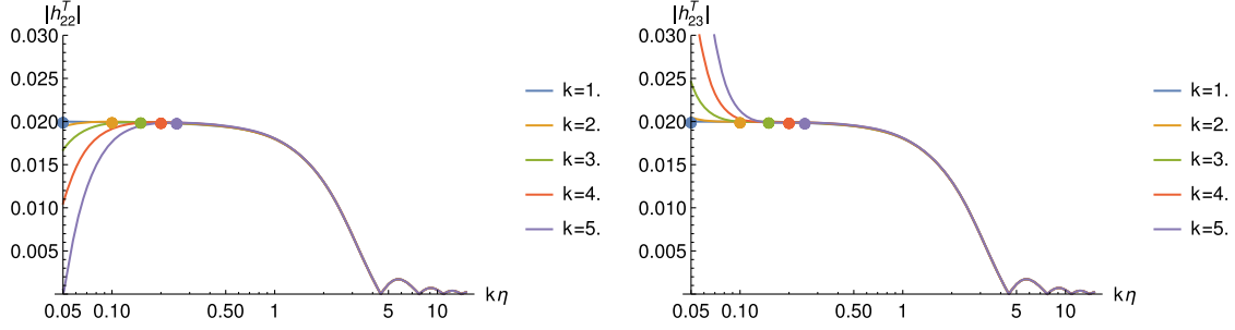
FIG. 5. Plots of |h_{22}^T| and |h_{23}^T| as functions of k\eta at different k . Colored dots illustrate their initial values. The initial condition is imposed at \eta_i = 0.05 . Initial values are u^{1,4,5,7,8} = 0 , u^3 = -u^2 = u^6 = u^9 = 0.00999754 and u'^3 = -u'^2 = u'^6 = u'^9 = -0.000099816 . Values of parameters are \Lambda = 0 , \alpha = 1 , \beta = 1 , \kappa = 1 , and \mu = 10^{-3} .
