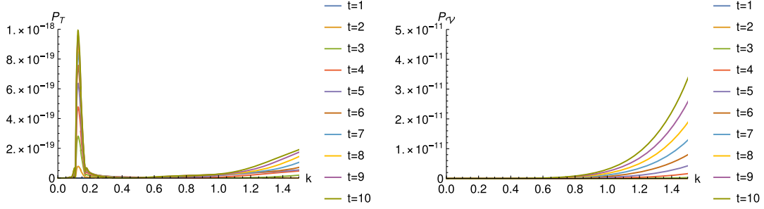
FIG. 3. The left panel plots tensor mode power spectra P_T = |h_{23}^T(\tau, k)|^2 as functions of k at different \tau , evolving from the scalar mode initial condition (the same as in Fig. 2). P_T at different \tau are illustrated by different colors. The other h_{IJ}^T component |h_{22}^T(\tau, k)|^2 is even smaller than |h_{23}^T(\tau, k)|^2 , thus is not demonstrated. The right panel plots vector mode power spectra P_V = |\vec{V}(\tau, k)|^2 at different \tau .
