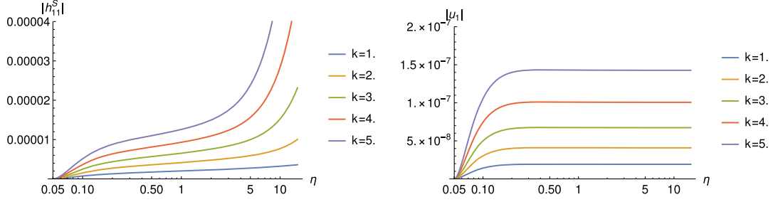
FIG. 8. Time evolution of the scalar modes h_{11}^S = (-V^1 + V^2 + V^3)/P_0 and u^1 = V^1/P_0 excited by the tensor mode at different k , with the same initial condition as in Fig. 5.
