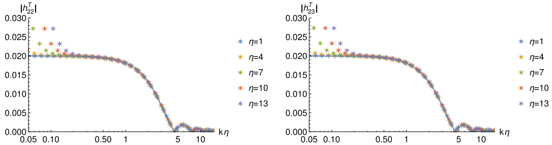
FIG. 7. Colored stars illustrate power spectra |h_{22}^T| and |h_{23}^T| , resulting from EOMs with \mu = 10^{-3} , as functions of k\eta at different conformal times \eta . Different colors label different \eta . The blue curve is the power spectrum from the continuum theory. The initial condition is the same as in Fig. 5.
