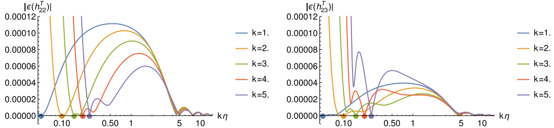
FIG. 6. Plots of |\epsilon(h_{22}^T)| and |\epsilon(h_{23}^T)| where \epsilon(h_{IJ}^T) = h_{IJ}^T - h_{IJ}^T|_{\mu \rightarrow 0} are differences between solutions of discrete and continuum EOMs. Colored dots illustrate initial values.
