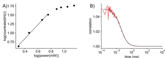
Figure 5. 2P single-molecule characterization of ABN. (A) logarithmic plot of the power dependence of the emission intensity. The first four points show a linear behavior with a slope of 1.9; the slope changes for powers higher than 5.7 mW, presumably due to saturation effects. (B) FCS measurement (red line) and fit to the data (black line). The fit gives an average of 7 molecules in the focus which leads to an average count rate per molecule of 7 \pm 0.5 kHz/molecule. The
