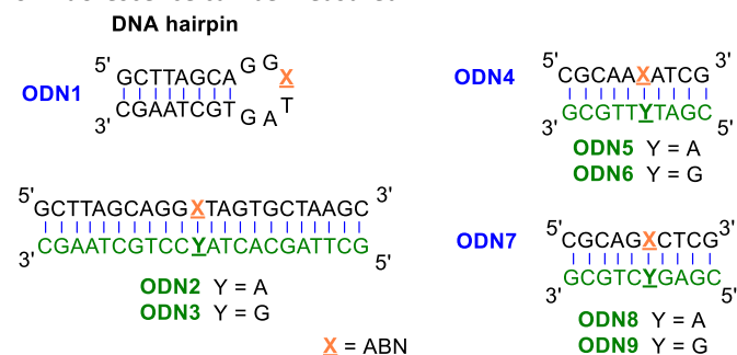
Figure 3. Oligonucleotides used to study the fluorescence and base pairing properties of ABN.
