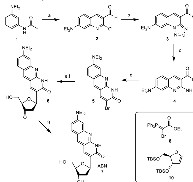
Figure 2. Synthesis of the ABN nucleoside analogue. Reagents, conditions, and yields: (a) DMF, \text{POCl}_3 , 50 °C, 20 min (15%). (b) \text{NaN}_3 , DMF, 90 °C, 18 h (85%). (c) \text{PPh}_3 , 2 N HCl, reflux, 2 h (70%). (d) 8 , NaOEt, ethanol, 70 °C, 4 h. (e) 10 , \text{AsPh}_3 , \text{Pd}(\text{OAc})_2 , \text{Bu}_3\text{N} , 60 °C, 18 h. (f) TBAF, AcOH, rt, 1 h. (g) \text{NaBH}_4(\text{OAc})_3 , AcOH, \text{CH}_3\text{CN} , 0 °C, 1 h (9% over 4 steps).
