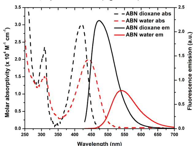
Figure 4. Absorption (dashed line) and emission (solid line) spectra of ABN in dioxane (black) and water (red). The integral areas of emission spectra are normalized to brightness \epsilon \cdot \Phi_{\text{em}} .
