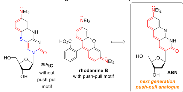
Figure 1. Push-pull motifs are hallmarks of bright organic fluorophores, but are rare in fluorescent nucleosides. The redesign of a nucleoside analogue to include this motif significantly increases \epsilon and \Phi_{\text{em}} , enabling single-molecule detection.
