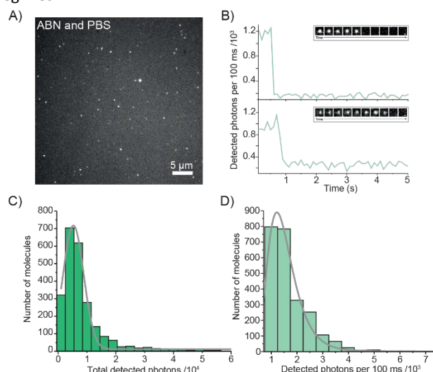
Figure 6. 1P single-molecule characterization of ABN. (A) Average fluorescence intensity projection of a 15 s movie of single ABN molecules adsorbed onto a glass surface. (B) Fluorescence intensity as a function of time of two single ABN molecules, with subsections of the traces shown as time montages (inset, scale bar = 200 nm). (C) A histogram showing the distribution of the total number of photons detected from single ABN emitters, \mu = 5300 \pm 1800 photons determined from a log-normal distribution fit. (D) A histogram showing the mean number of photons detected/frame for single ABN emitters, \mu = 1500 \pm 600 photons / 100 ms, determined from a log-normal distribution fit. ( N=2402 molecules).
