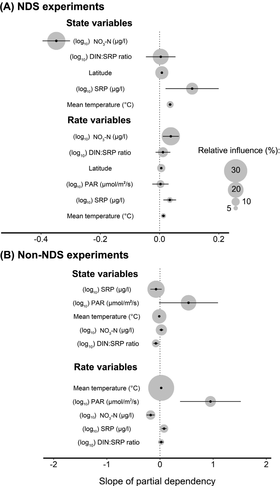
Fig 6. Slopes of relationships between partial dependency values derived from boosted regression tree (BRT) models and values for independent variables with >5% relative influence. Slope estimates \pm 95% confidence intervals are shown. The relative influence of each variable is depicted by the size of the grey bubble. DIN, dissolved inorganic nitrogen; NDS, nutrient-diffusing substrata; PAR, photosynthetically active radiation; SRP, soluble reactive phosphorus.
